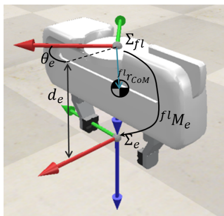
Figure 8.2 – Coppeliasim model of the Franka Hand gripper. End-effector position {}^{fl}\mathbf{r}_e = [0; 0; d_e]^\top [m] and orientation {}^{fl}\mathbf{R}_e = R_z(\theta_e) and CoM position {}^{fl}\mathbf{r}_{CoM} = [-0.01; 0; 0.03]^\top [m] in flange frame. Mass m_L = 0.73 [kg] and inertia tensor \mathbf{I}_L = \text{diag}(0.001; 0.0025; 0.0017) [kg.m^2] . \theta_e = -45^\circ , d_e = 0.1034[m] .
