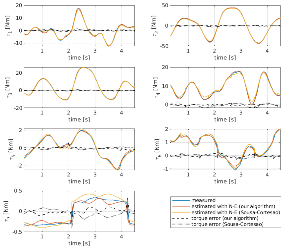
Figure A.1 – Comparison between measured joint torques during a validation trajectory (blue solid lines) and estimated torques generated from a N-E routine using the \hat{\boldsymbol{p}} parameters from our parameter retrieval method in [8] (see Chap. 7) (solid red lines) and the parameters \boldsymbol{\delta} from the LMI-SDP framework in [91] (solid yellow lines). The torque errors are reported as well.
