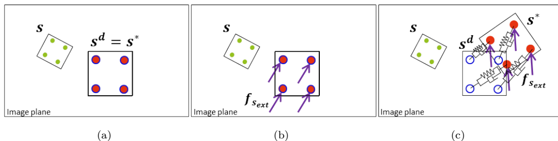
Figure 6.1 – The Compliant frame concept extended to the feature space: (a) Desired and Compliant features are coincident, the current features follow the compliant features. (b) The sensor undergoes the action of an external force. (c) The compliant features are linked to the desired ones with a mass-spring-damper relationship.
