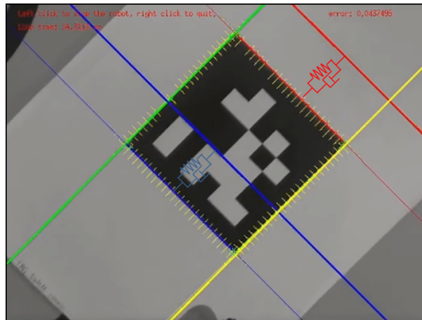
Figure 6.2 – The four sides of the AprilTag are used as image line features. The reference lines (thicker lines) experience a spring-like displacement according to the chosen impedance parameters and the sensed forces.
