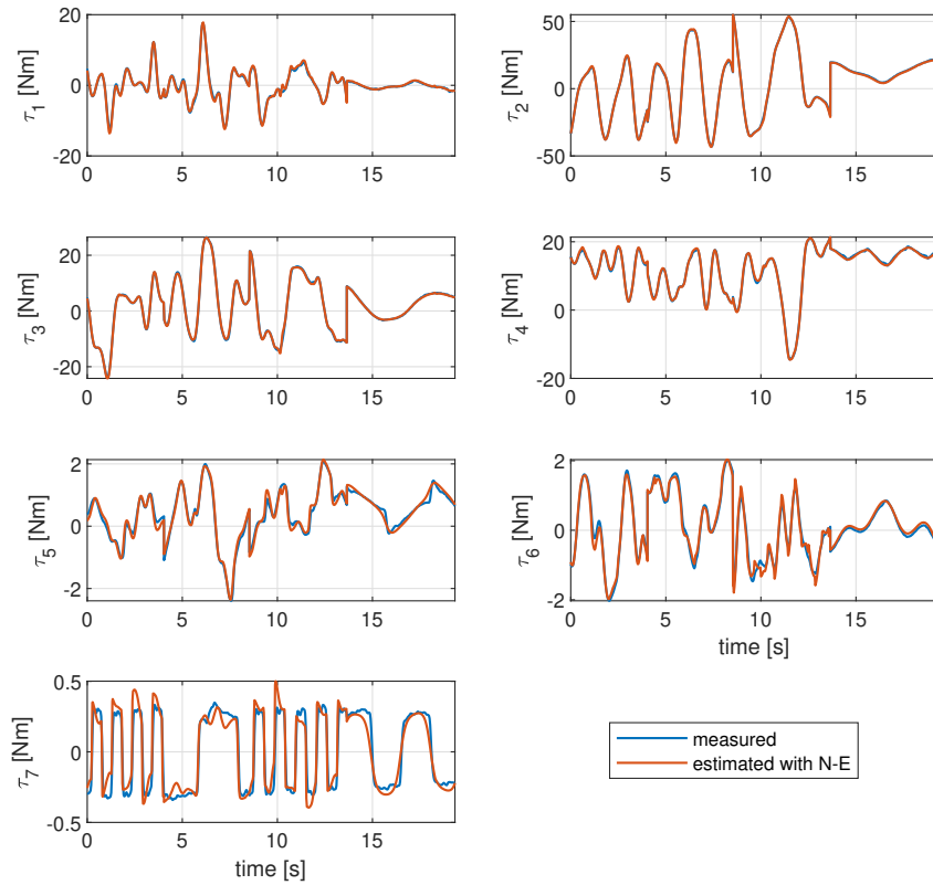
Figure 7.4 – Comparison between the torques \hat{\tau}_{ne} (including friction \hat{\tau}_f ) from the N-E dynamic model and the ones retrieved from the the joint torque sensors. The overlapping of two signals shows the quality of the obtained parameters estimation \hat{\mathbf{p}} .
