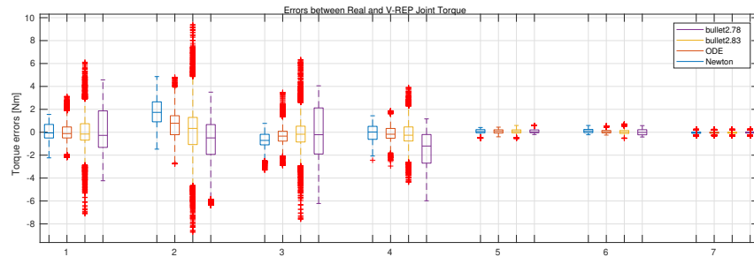
Figure 7.7 – Torque errors (w.r.t. the real robot) of the physics engines Bullet 2.78, Bullet 2.83, ODE, and Newton in CoppeliaSim during an experiment with the Panda robot for each of its 7 joints. The boxes indicate mean values of the errors while the bars denote their standard deviations.
