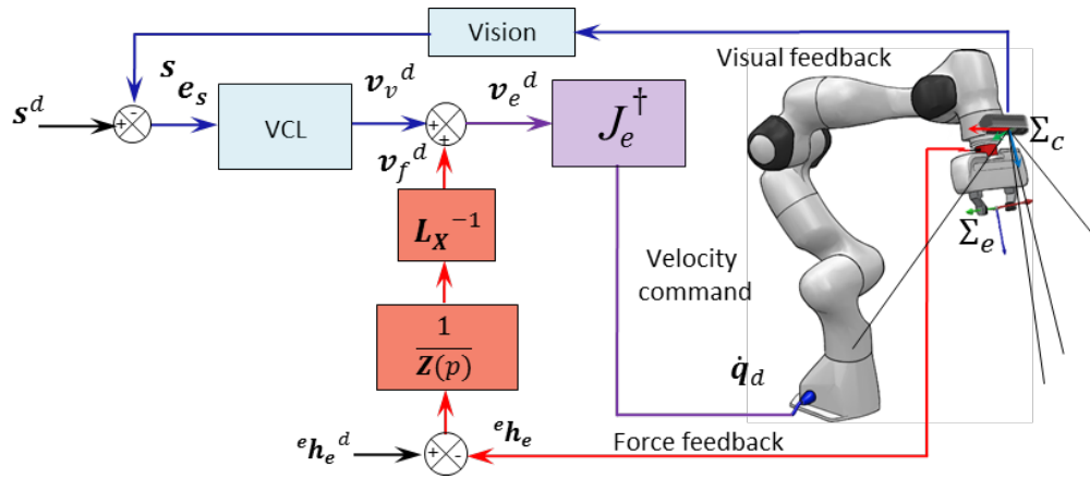
Figure 4.2 – Impedance-based vision/force control scheme
