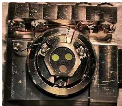
Figure 2.8. Photograph of the sample holder used to fix the cells for the TEMPO beamline.
