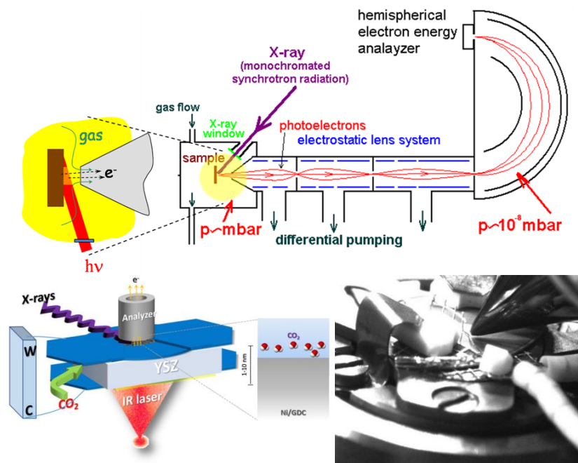
Figure 2.7. (Top) Schematic diagram of the in-situ NAP-XPS set-up under the electrochemical gas-phase conditions. Reproduced with permission [122]. Copyright 2019, the RSC. (Bottom) A schematic depicting the experimental setup. The cell is based on dense yttria-stabilized zirconia (YSZ) solid-oxide electrolyte, with porous Ni/Gd-doped ceria (Ni/GDC) as the working electrode and porous Pt as the counter electrode. The sample holder was mounted inside the NAP-XPS chamber.
