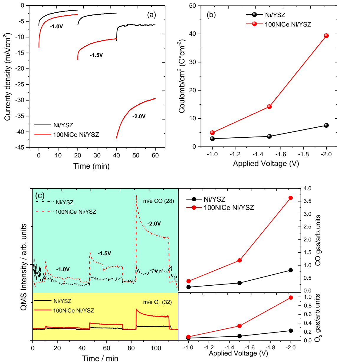
Figure 6.1. (a) Three potential step chronoamperometric measurements as well as corresponding total charge in coulomb (b) over Ni/YSZ (black lines) 100NiCe Ni/YSZ (red lines) (c) The evolution of the CO (m/e 28) and O 2 (m/e 32) gas phase signals recorded by on line QMS in parallel with the chronoamperometric measurements, as well as corresponding integrated O 2 and CO gas QMS signal at each potential. Ni/YSZ (black lines) 100NiCe Ni/YSZ (red lines), Reaction conditions: 0.5 mbar CO 2 at 550 °C.
