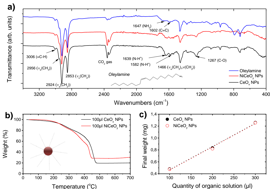
Figure 5.1. (a) FTIR spectrum of as-synthesized CeO x and NiCeO y NPs as well as of OLA reference sample. (b) The TGA thermogram of 100 μL CeO x and NiCeO y NPs in their organic solutions. (c) The final weight of CeO x and NiCeO y NPs at 500 °C as a function of different quantities of organic solutions in TGA measurement.
