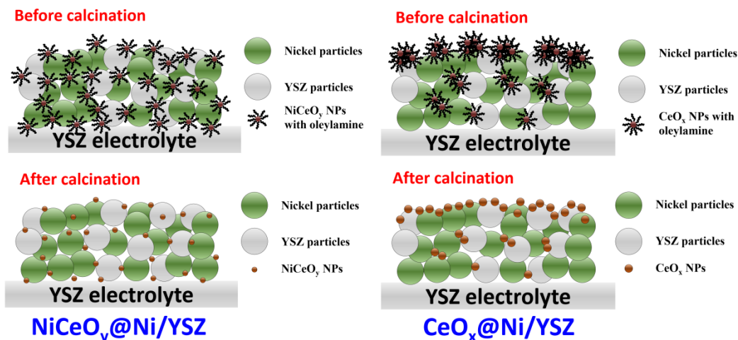
Figure 5.18. Schematic representation of the arrangement of the \text{NiCeO}_y and \text{CeO}_x NPs over the Ni/YSZ cermet before and after firing step.
