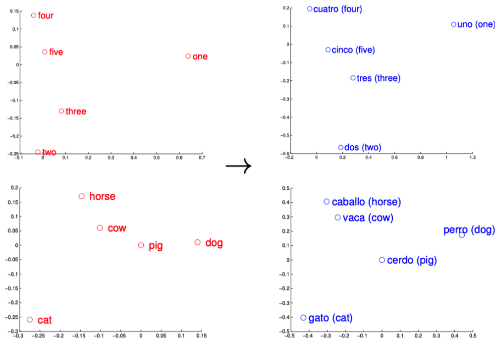
FIGURE 2.4: An example for the distributed representation of words
