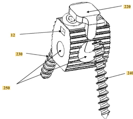
FIGURE 4.9: Frontal perspective view of the posterior lumbar elliptical design of the vertebral cage/BDFT construct (frontal isometric)
