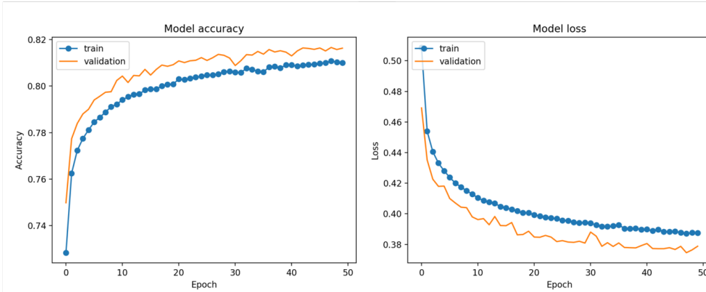
FIGURE 4.6: The illustration of learning curves
