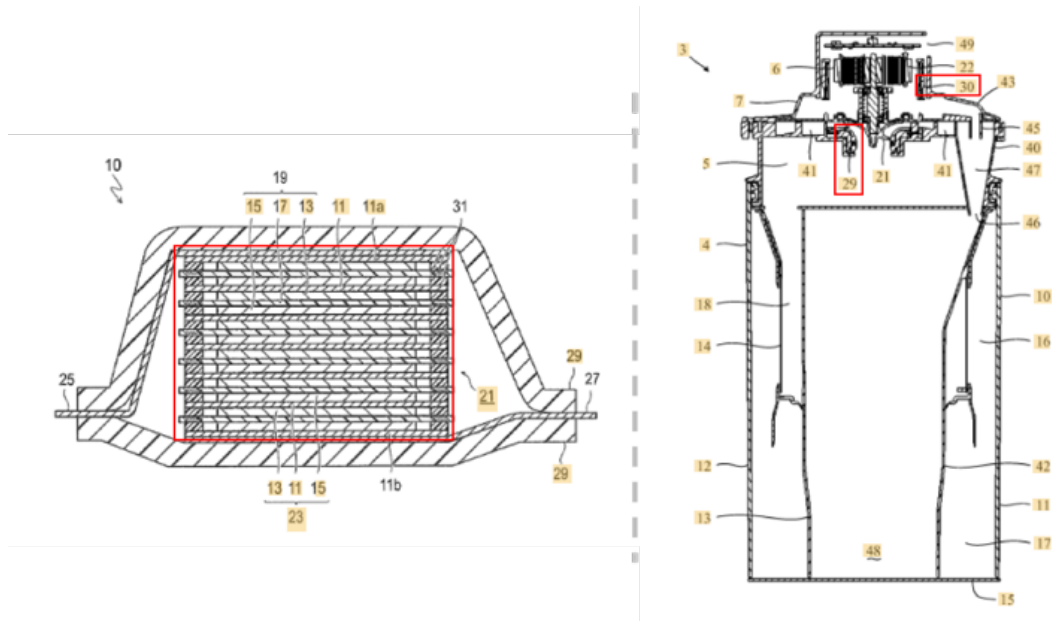
FIGURE 4.7: Diagrams of the sealing member (left) and the elastomeric material (right)
