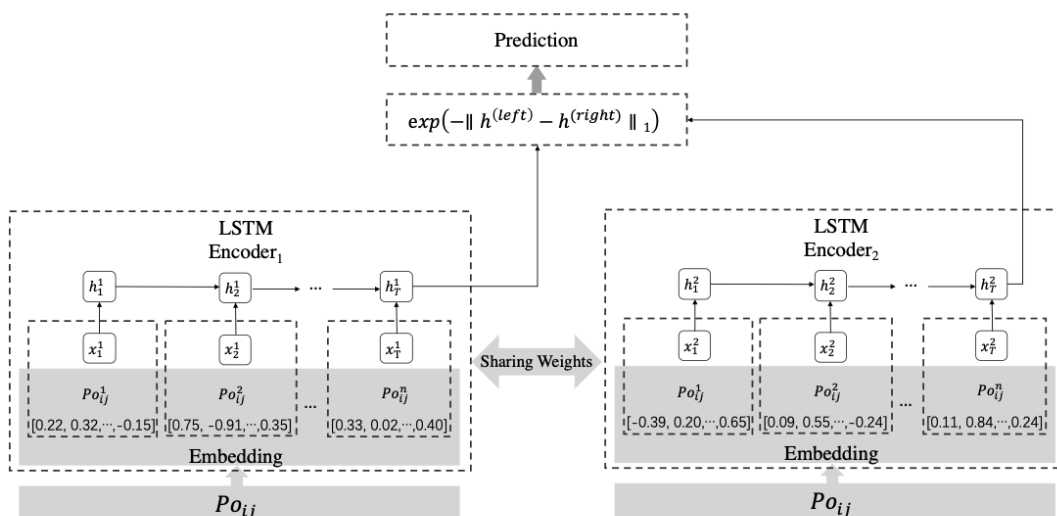
FIGURE 4.4: The structure of MaLSTM
