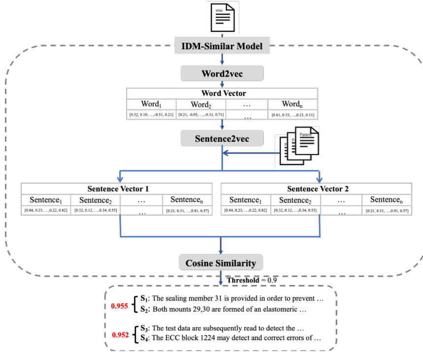
FIGURE 4.1: An overview of IDM-Similar
