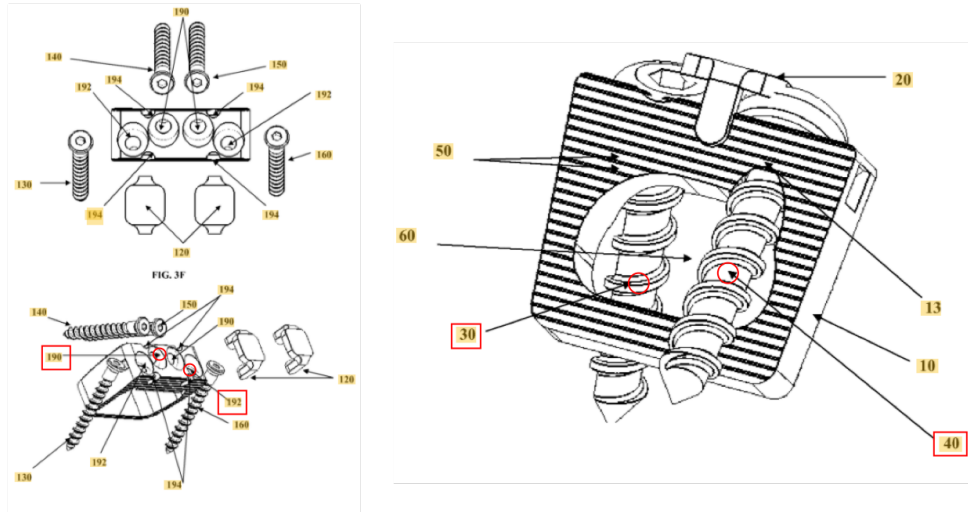
FIGURE 4.10: The illustration of the locking mechanism
