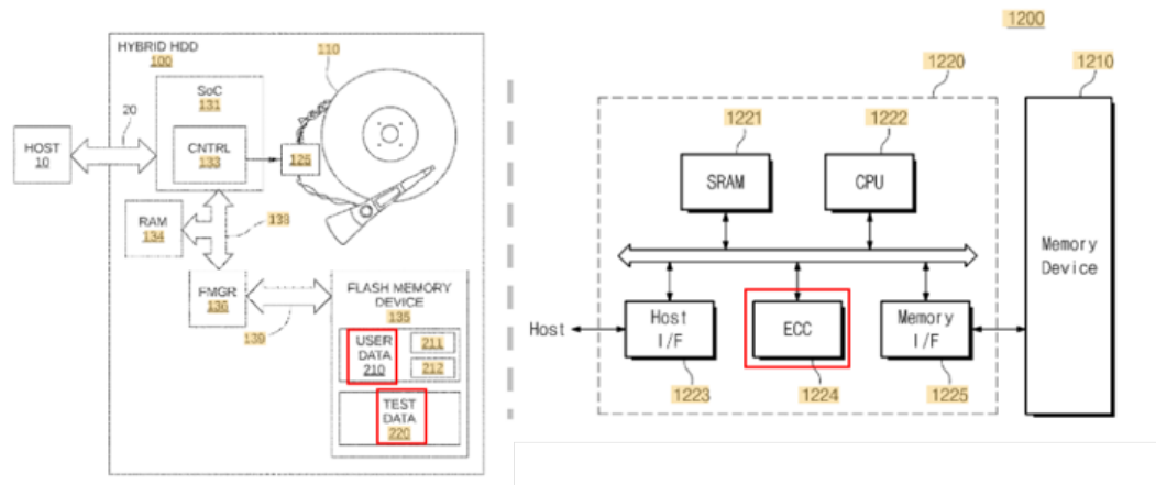
FIGURE 4.8: Diagrams of the hybrid HDD (left) and the memory systems (right)
