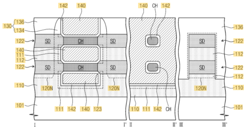
FIGURE 4.11: The illustration of a semiconductor device with a domain effect transistor.
