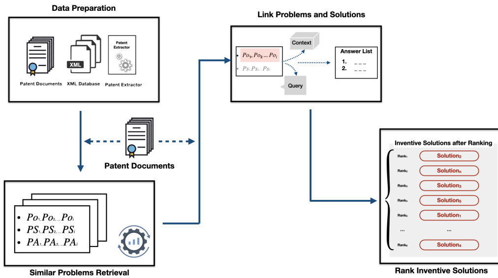
FIGURE 1.2: The global architecture of the thesis
