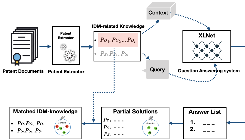
FIGURE 5.1: The framework of IDM-Matching
