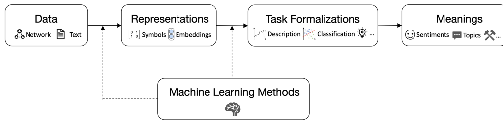
FIGURE 2.1: The generic process of NLP
