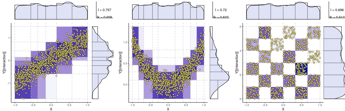
Figure 3.10: Optimal discretization of three joint distributions with the same marginal X , as found by maximizing \hat{I}'(X;Y) .
