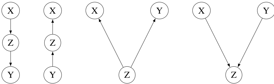
Figure 3.4: DAGs with 3 nodes and 2 edges.
