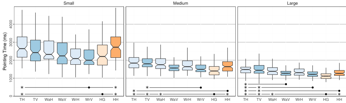
Fig. 1.9: Notched box plots for the pointing time per \text{TECHNIQUE} \times \text{TARGETWIDTH} condition.
