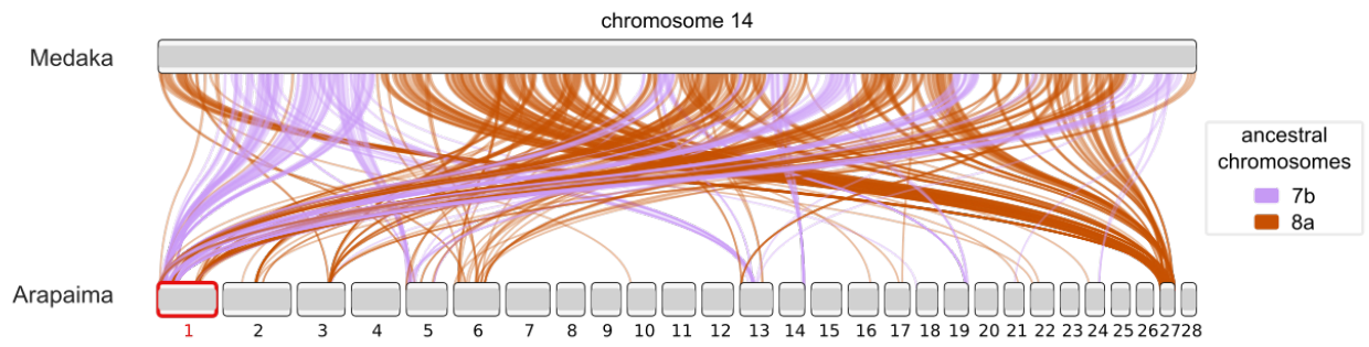
Supplementary Figures S8: Synteny comparisons of arapaima genome and medaka chromosome 14. Medaka chromosomes 14 descend from the fusion and mixing of ancestral chromosomes 7b and 8a. A few orthologous genes of chromosome 14 descending from 7b and 8a are mixed together on arapaima chromosome 1.
