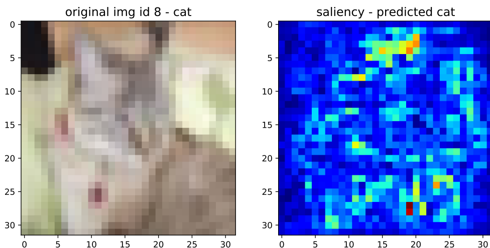
Figure 2.12 – A test image (a cat) from CIFAR dataset and the gradient-based saliency map of the test image predicted on a customize CNN model. A saliency map in which pixels are colored by their contribution to the classification.
