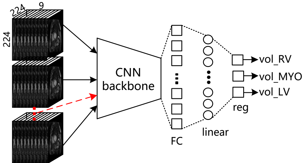
Figure 5.5 – The architecture of regression CNN for predicting the volume of RV, MYO, LV directly. The input training data are preprocessed MRI images (224,224,9), the ground truth are the volume of 3 structures of cardiac. FC is fully connected layer after feature representation, the FC layer goes through linear regression layer, the output is the predicted volumes (vol_RV, vol_MYO, vol_LV).
