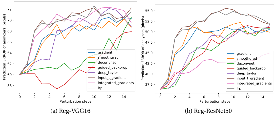
Figure 4.13 – Prediction error (in pixels) of different analyzers during each perturbation step based on Regression VGG16 and Regression ResNet50 model. The horizontal axis is the perturbation steps.
