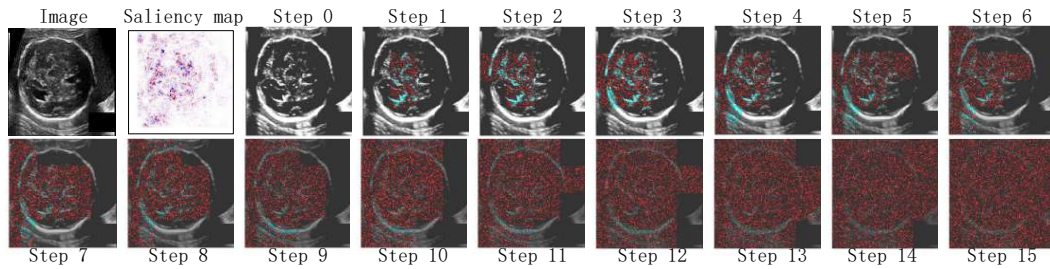
Figure 4.12 – Perturbation process for the saliency map produced by the Gradient method. Step 0 is the original input image. From step 1 to step 15, Gaussian noise is added gradually on the image subwindows. The perturbation order of these subwindows corresponds to the saliency scores assigned by the Gradient method analysis, i.e. the most contributing pixels are perturbed first. Red: noise, blue: original image pixels.
