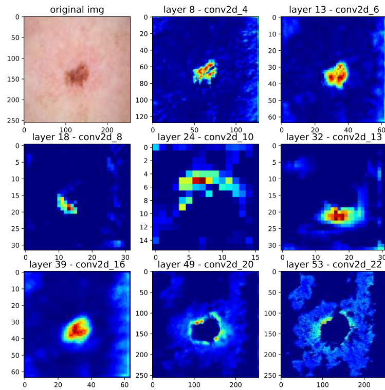
Figure 3.9 – Feature maps of U-Net with Dice loss on a skin image with small lesion.
