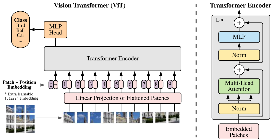
Figure B.3 – Vision Transformer model. An image is split into certain number of patches. The position information is added in each patch. A learnable classification matrix is also added. The figure is obtained from [Dosovitskiy et al., 2020].
