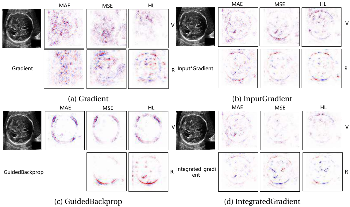
Figure A.2 – Saliency maps of different explanation methods under 3 different loss functions and regression CNN model VGG16 (V) and ResNet50 (R).
