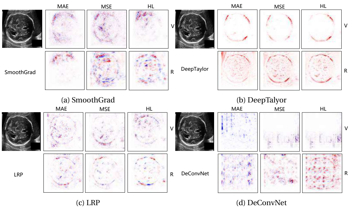
Figure A.3 – Saliency maps of different explanation methods under 3 different loss functions and regression CNN model VGG16 (V) and ResNet50 (R)
