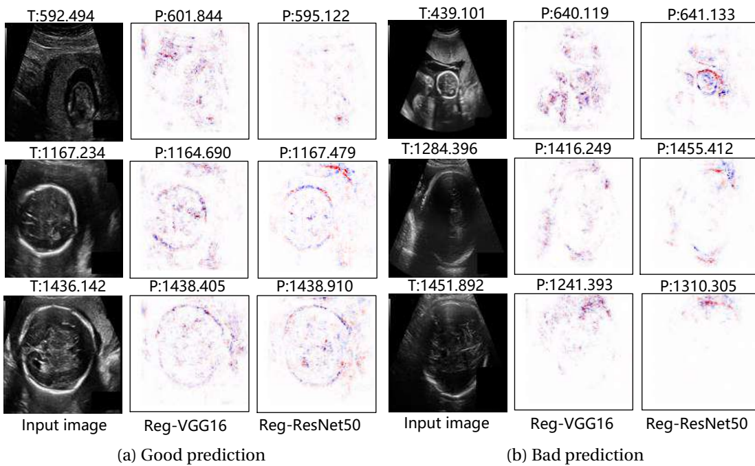
Figure A.1 – Saliency map of Reg-VGG16 and Reg-ResNet50 with Input*Gradient explanation method. P and T: resp. predicted and ground truth HC values (pixels).
