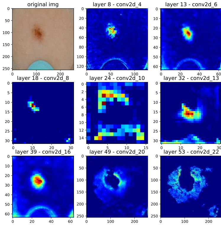
Figure 3.7 – Feature maps of U-Net with Dice loss on a noisy skin lesion image.
