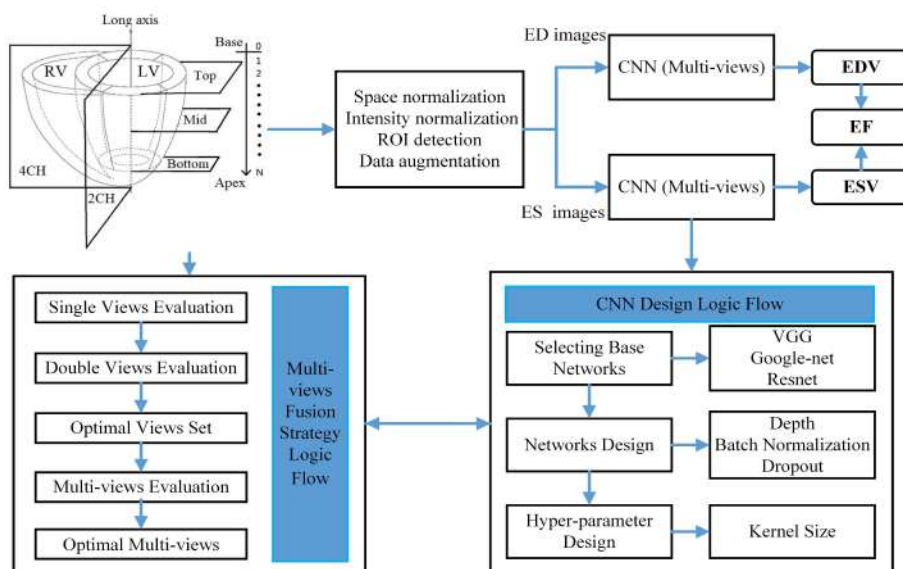
Figure 2.5 – Multi view/channel fusion strategy, the input is cardiac top slice, middle slice and bottom slice, the figure is obtained from [Luo et al., 2017].
