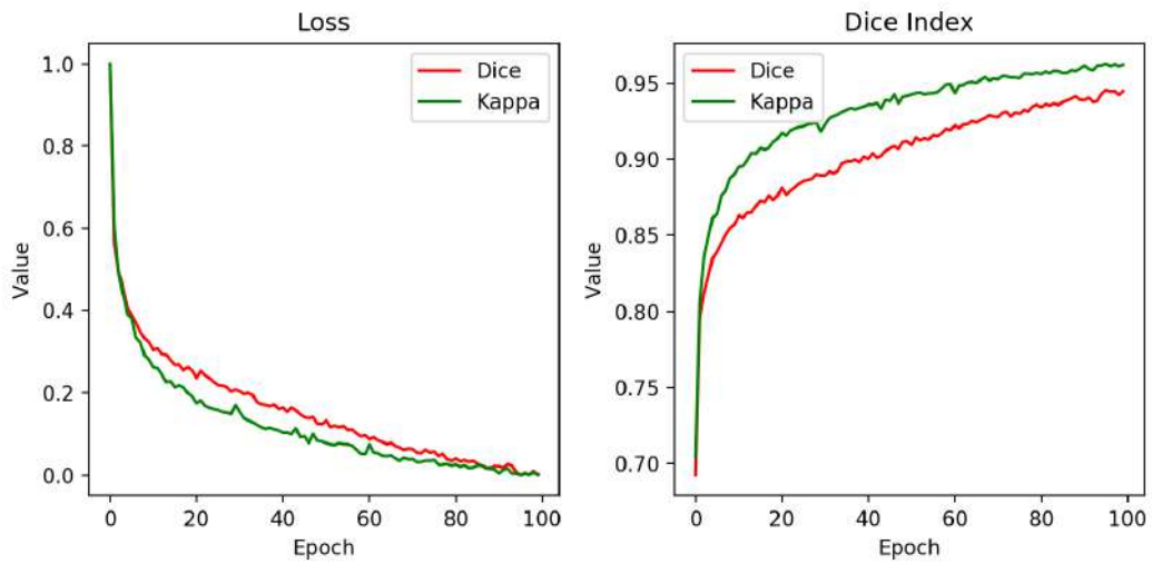
Figure 3.5 – Loss function (left) and DI metric (right) during the 100 epochs of training process on the dataset ISIC 2016.
