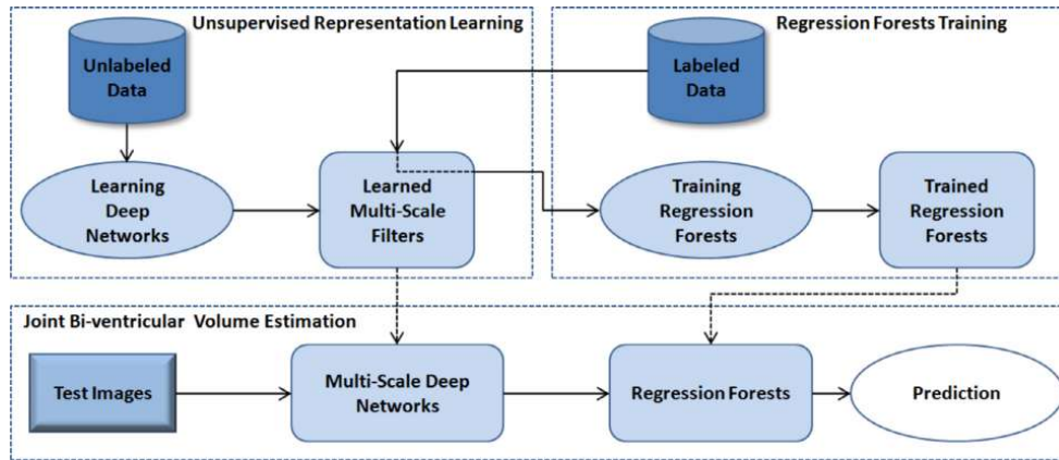
Figure 2.9 – The flowchart of the feature learning and random forest regression, the figure is obtained from [Zhen et al., 2016a].
