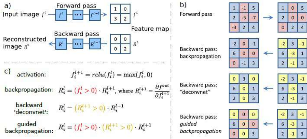
Figure 2.14 – Comparison of gradients, deconvnet, guided backpropagation methods (Figure is adapted from [Springenberg et al., 2015]).
