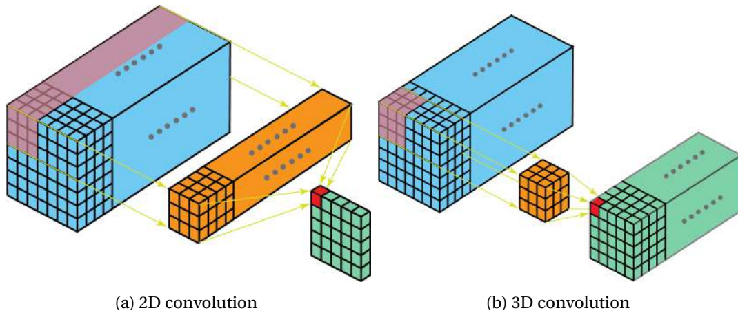
Figure 5.4 – 2D (a) and 3D (b) convolution on 3D image. For 2D convolution, the input layer and the filter have the same depth (channel number = kernel/filter number), the output is a one-layer matrix. For 3D convolution, the filter moves on 2D channel then moves in z direction, the output is a 3D matrix. The figure is taken from Towardsdatascience.
