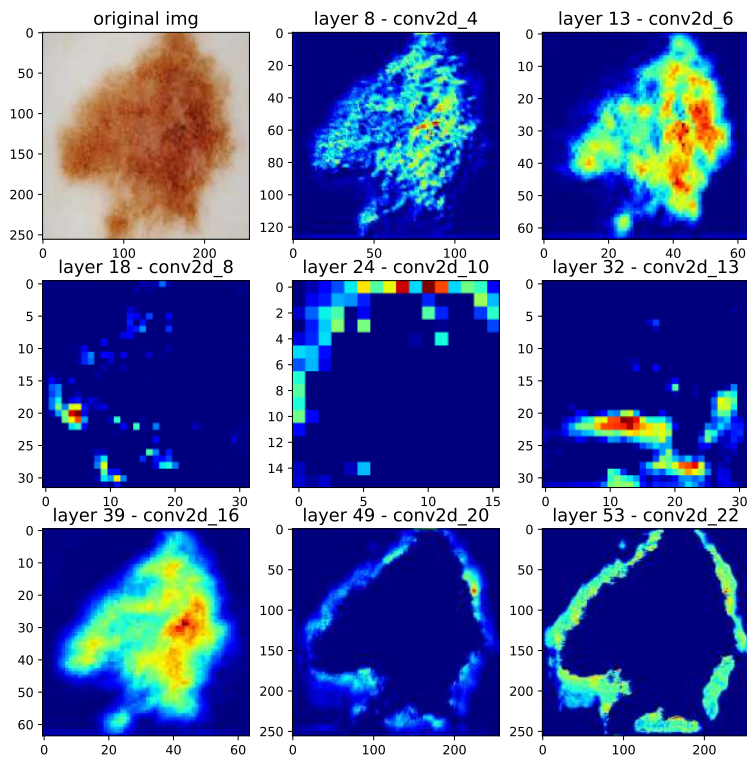
Figure 3.11 – Feature maps of U-Net with Dice loss on a skin image with large lesion.
