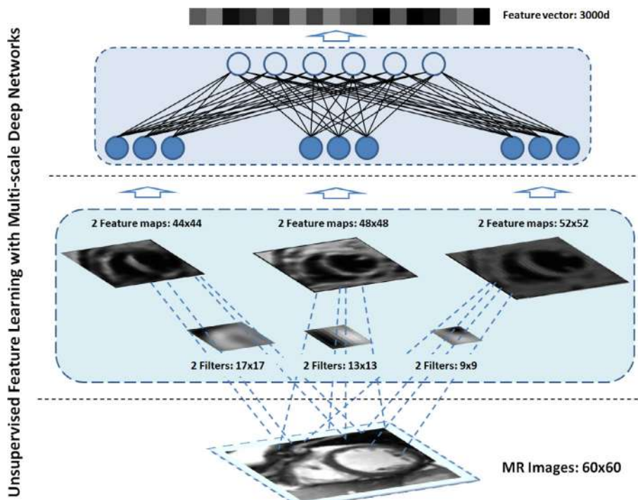
Figure 2.6 – Multi-feature fusion strategy, the input is cardiac images, the feature maps are in different size because of different kernel/filter size, the figure is obtained from [Zhen et al., 2016a].
