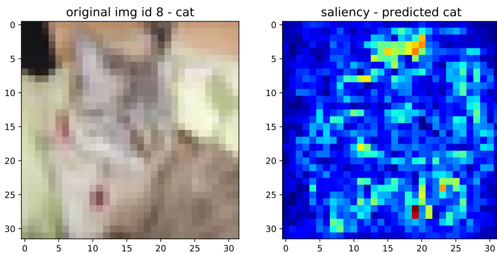
Figure 2.12 – A test image (a cat) from CIFAR dataset and the gradient-based saliency map of the test image predicted on a customize CNN model. A saliency map in which pixels are colored by their contribution to the classification.
