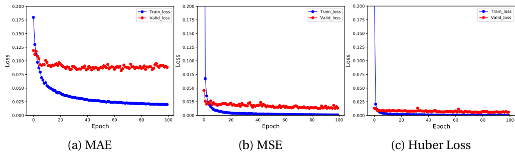
Figure 5.6 – Learning curves of regression ResNet model with different loss functions. Blue curve is training loss, red curve is valid loss.
