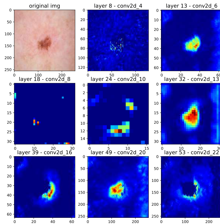
Figure 3.10 – Feature maps of U-Net with Kappa loss on a skin image with small lesion.
