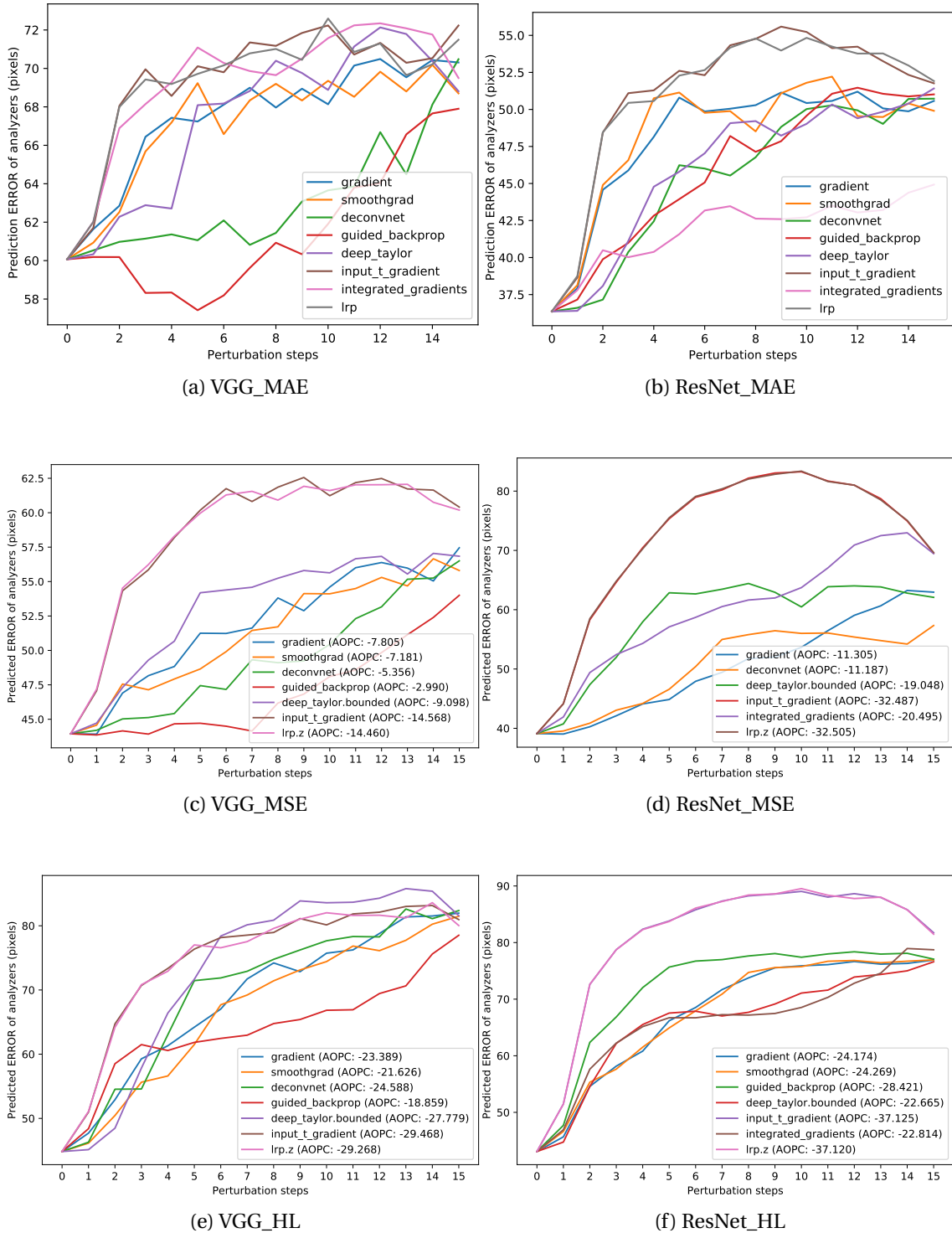
Figure A.4 – Perturbation steps of different analyzers under Regression VGG16 and Regression ResNet model with loss function MAE, MSE, HL, respectively.
