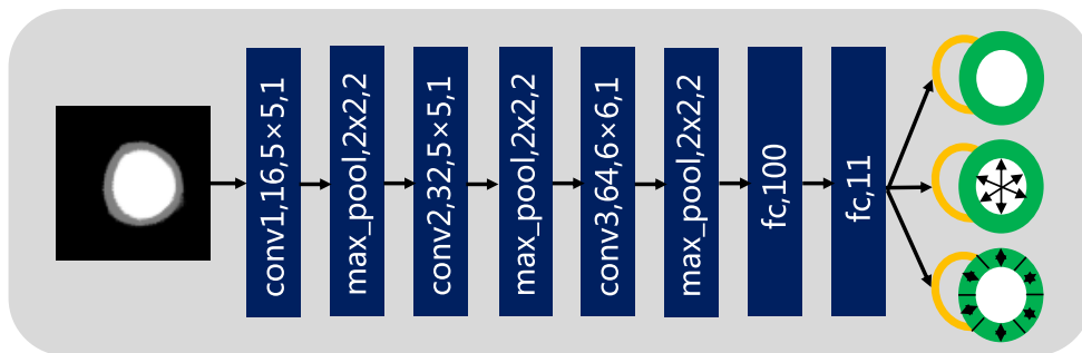
Figure 2.8 – Segmentation results as input training data, the outputs are indices of cardiac, the figure is obtained from [Wang et al., 2019].
