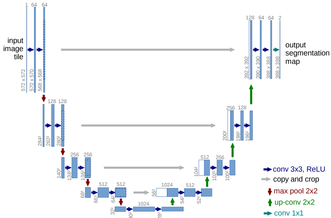
Figure 2.2 – Original U-Net architecture. The number of channels is denoted above the box, different colors mean different operation.
