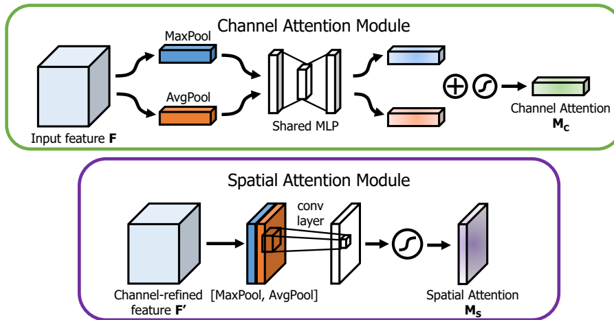
Figure 2.11 – Attention mechanism in computer vision. The figure is obtained from [Woo et al., 2018].
