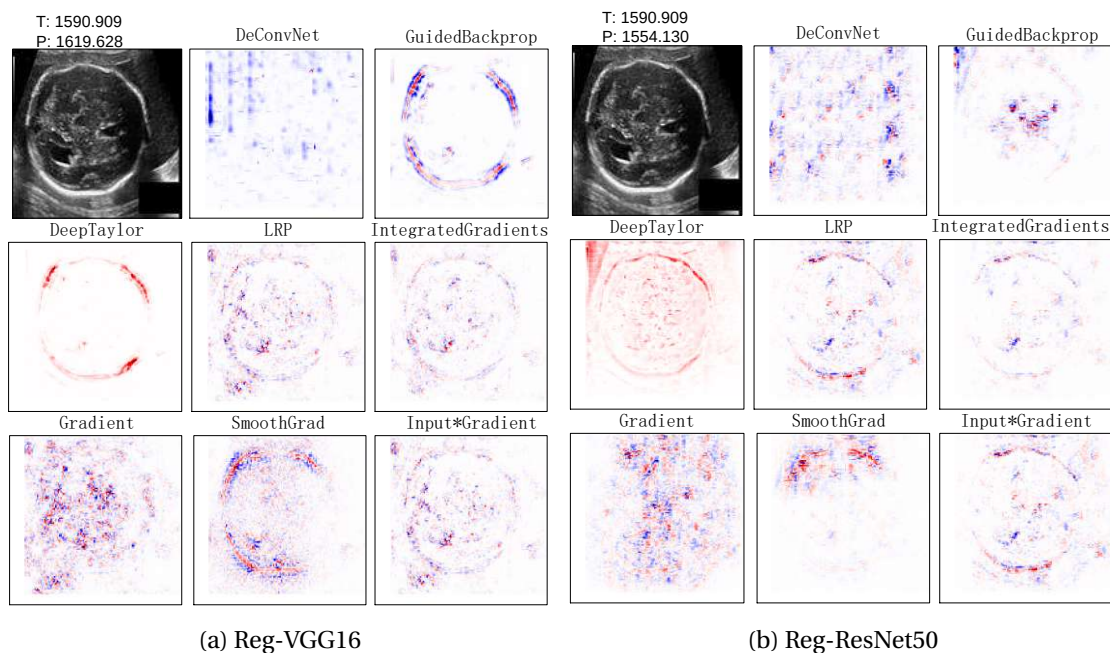
Figure 4.11 – Comparison of different saliency maps with Reg-VGG16 and Reg-ResNet50. P: predicted HC value, T: ground truth HC value (in pixels).
