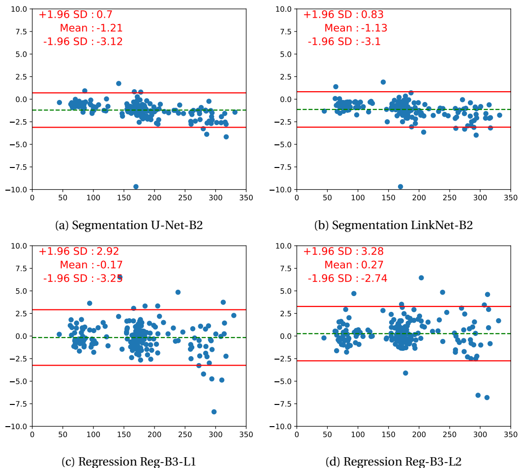
Figure 4.6 – Bland–Altman plots of the segmentation and regression CNN models. The x-axis represents the average value of ground truth and predicted HC; the y-axis, the difference between ground truth and predicted HC (in mm). The horizontal red solid lines represent the upper and lower limits of 95% consistency. The middle dotted green line represents the mean of the difference.
