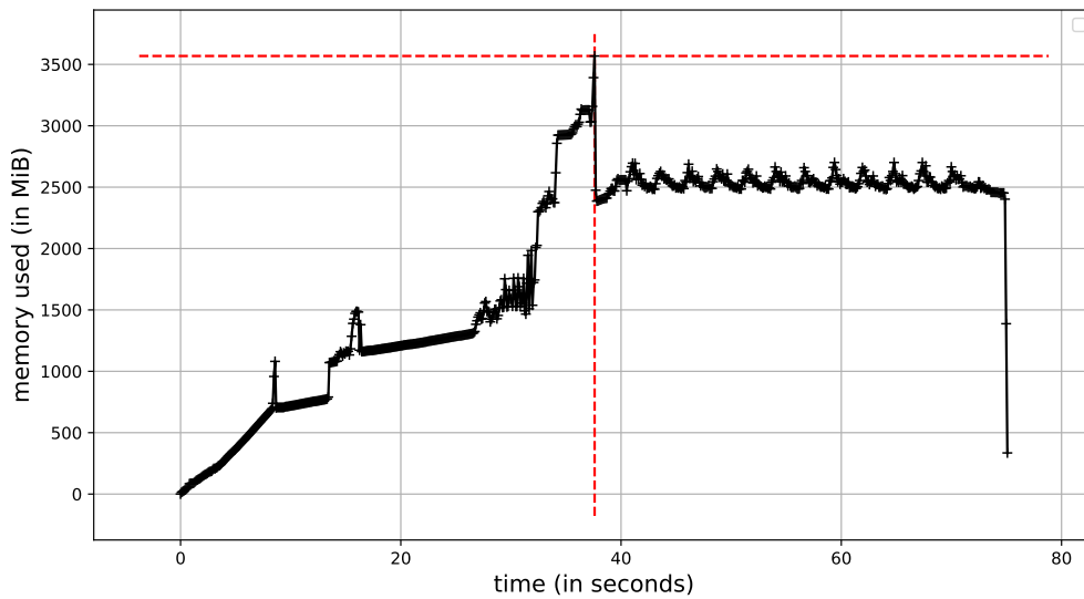
Figure 4.8 – Memory cost of Regression B3=EfficientNet, L1=MAE during prediction stage. The maximum used memory of models is after the red vertical line.
