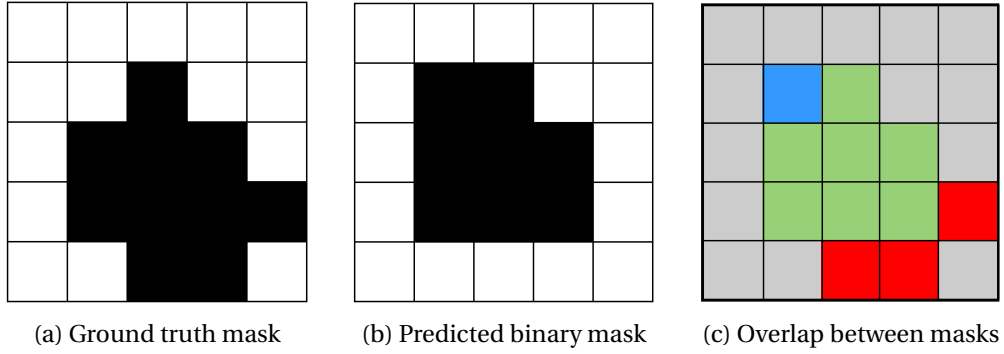
Figure 2.4 – A diagram of Ground truth image (a), predicted image (b) and the overlap between two masks (c). In (c), green pixels are TP, blue ones are FP, red ones are FN, grey ones are TN. The figure is adapted from [Taghanaki et al., 2021].
