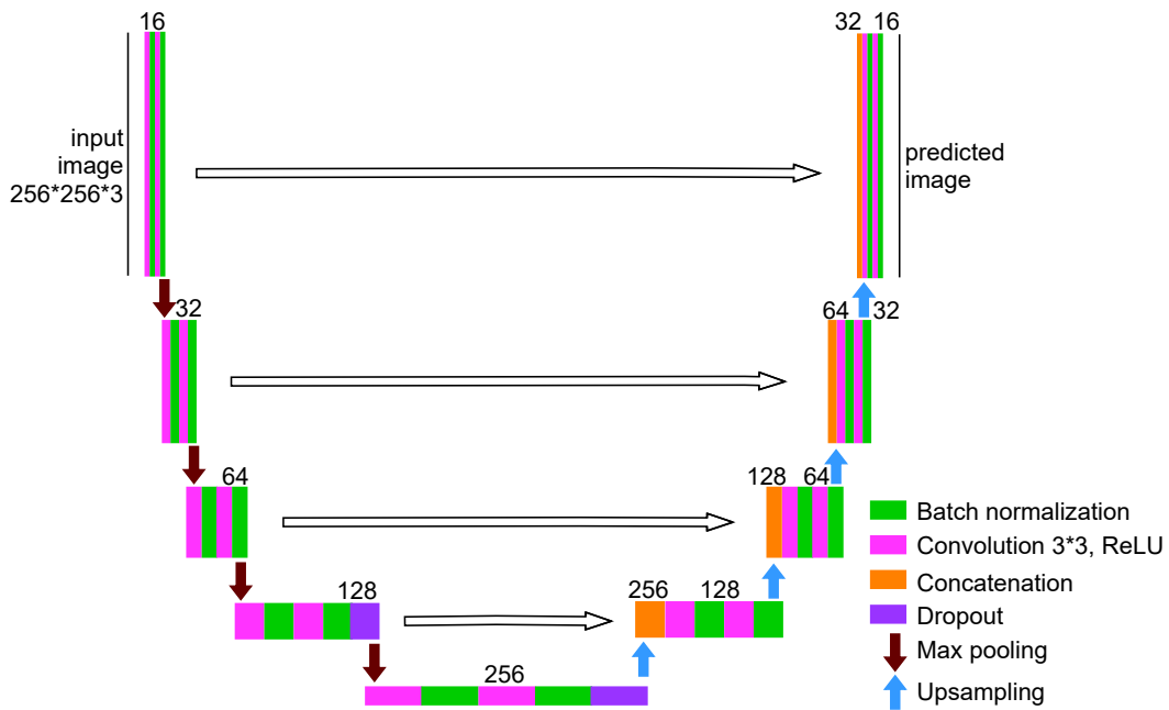
Figure 3.3 – Architecture of customized U-Net. Each box corresponds to a multi-channel feature map. The number of channels is denoted above the box, different colors mean different operation.
