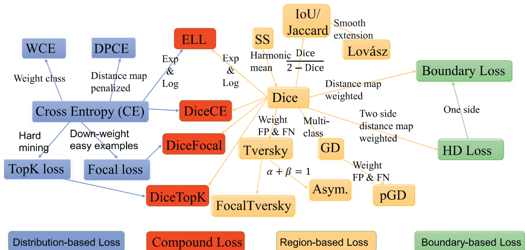
Figure 2.3 – A review of loss functions. The figure is obtained from [Ma et al., 2021].
