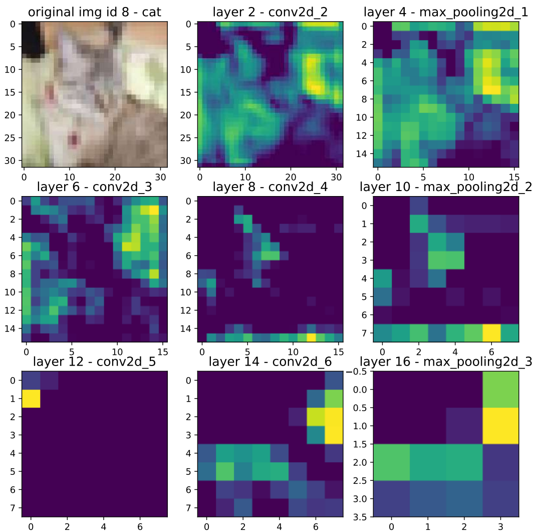
Figure 2.13 – A test image (a cat) from CIFAR dataset and feature maps of different layers of a customize CNN model.
