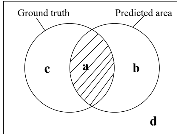
Figure 3.2 – Venn diagram of ground truth and predicted area. Ground truth contour vs predicted contour, with a , b , c the number of pixels included in both contours, only in the predicted area, only in the ground truth, respectively.
