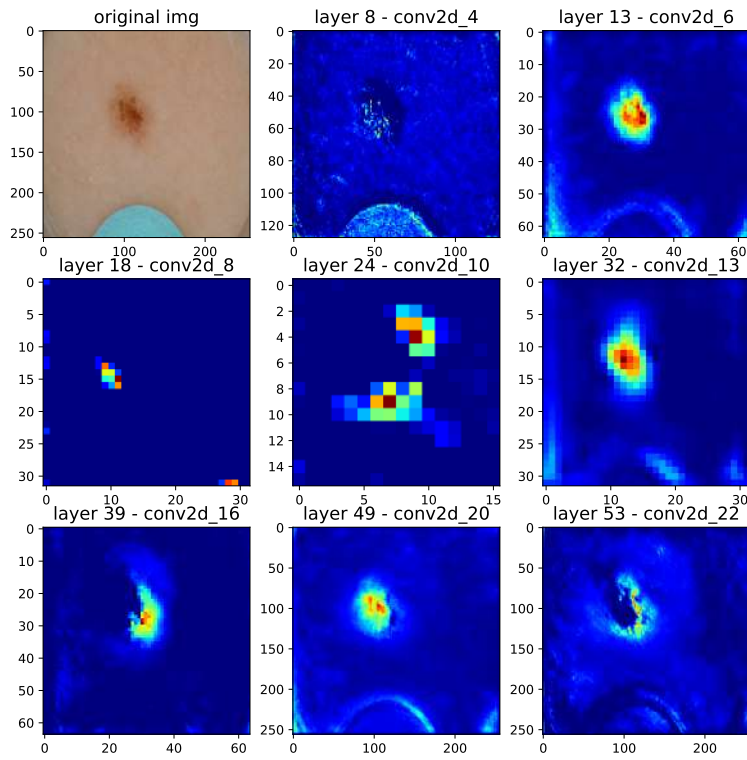
Figure 3.8 – Feature maps of U-Net with Kappa loss on a noisy skin lesion image.
