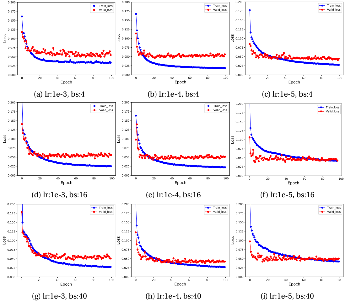
Figure B.2 – Learning curves (loss changing) of different learning rates (ls) and batchsize (bs) during training stage. Blue dotted line is training loss, red dotted line is valid loss.
