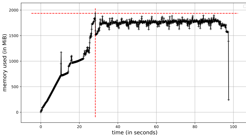
Figure 4.7 – Memory cost of U-Net, B2=ResNet during prediction stage. The maximum used memory of models (when the inference is stable) is after the red vertical line.
