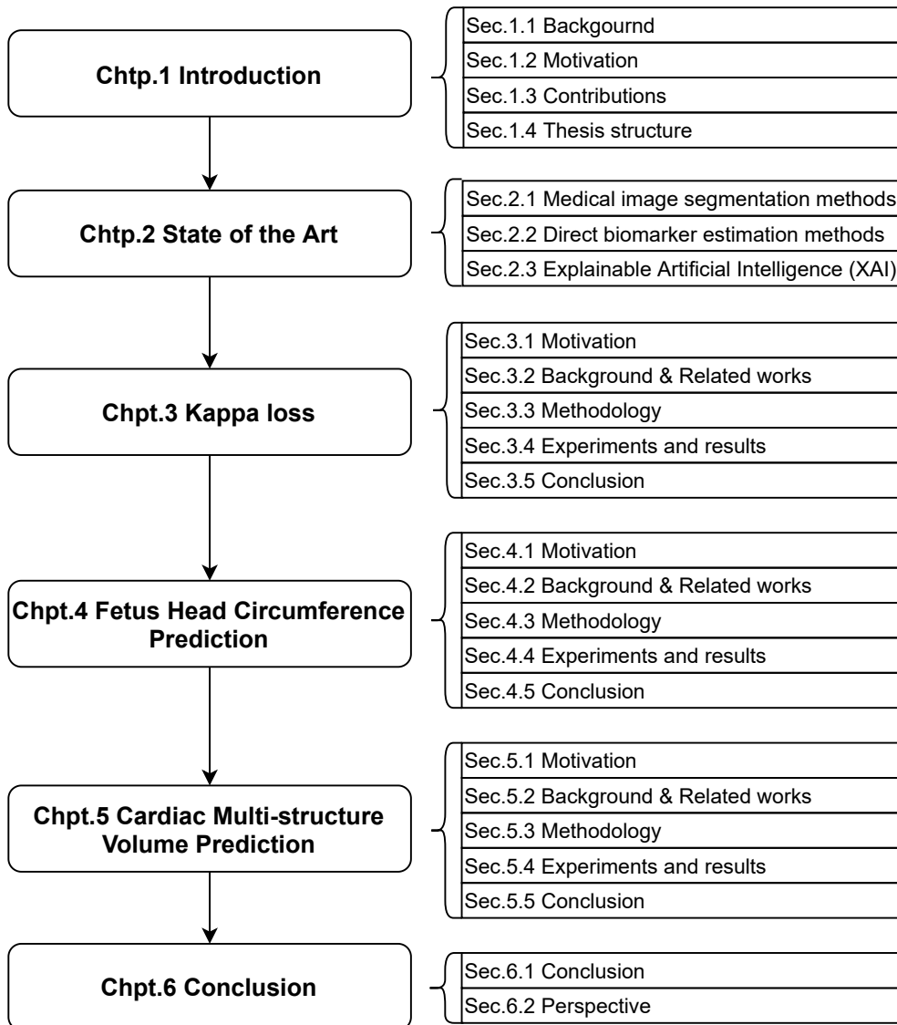
Figure 1.6 – Thesis structure.
