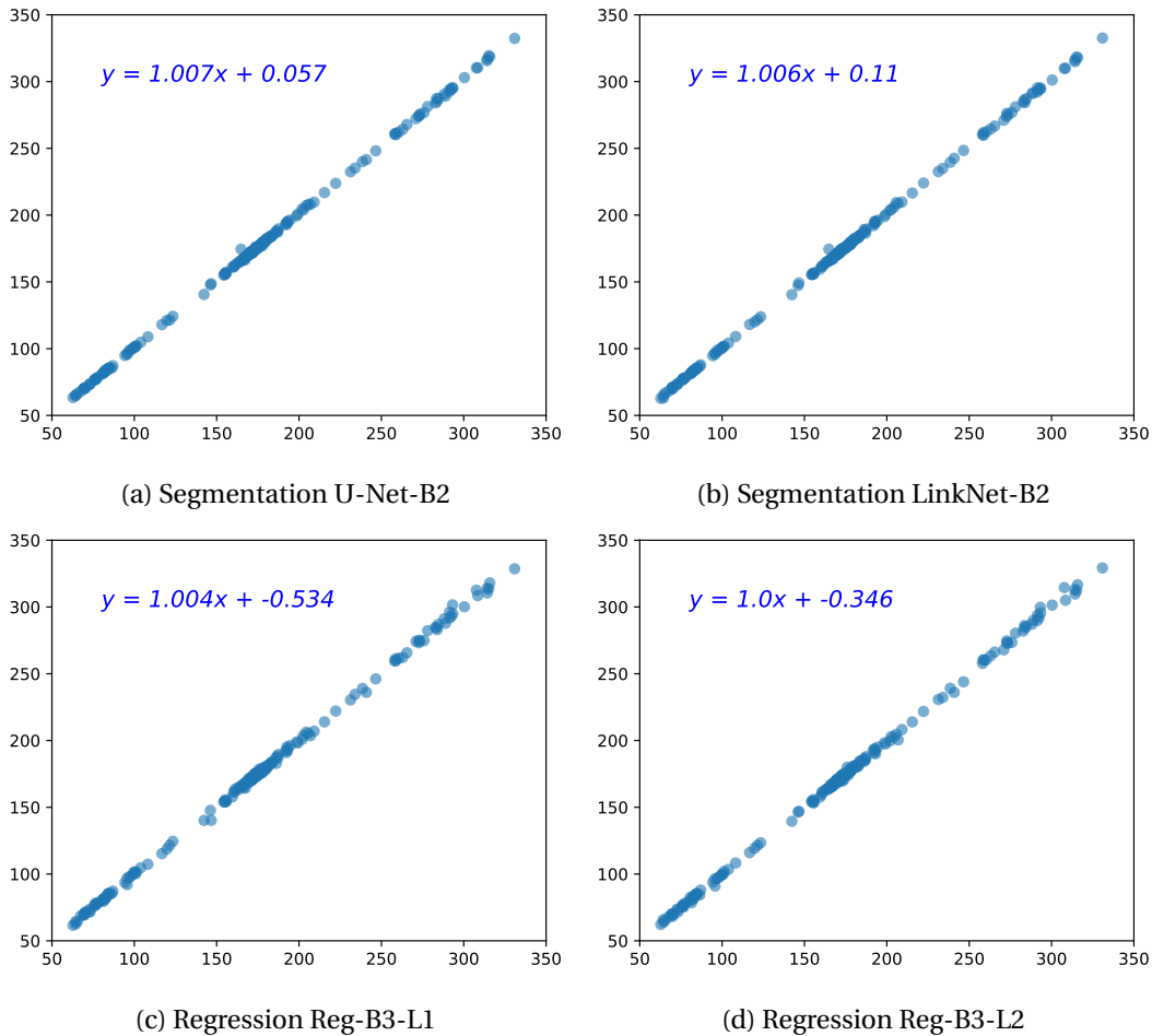
Figure 4.5 – Scatter plots of the 2 best segmentation models U-Net-B2 and LinkNet-B2, and regression models (L1 = MAE loss, L2 = MSE loss). The x-axis represents the ground truth HC and the y-axis the predicted HC (in mm).
