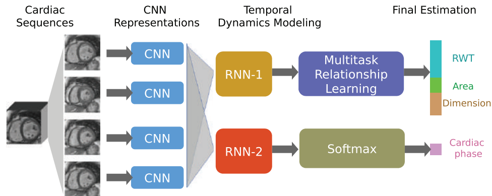
Figure 2.7 – Multi-task learning with different neural networks, the figure is obtained from [Xue et al., 2018]
