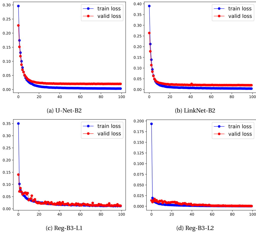
Figure 4.4 – Learning curves of segmentation (U-Net-B2, LinkNet-B2) vs. segmentation-free method (Reg-B3-L1, Reg-B3-L2) in training and validation stage. The x-axis represents the training epochs; the y-axis is the loss.
