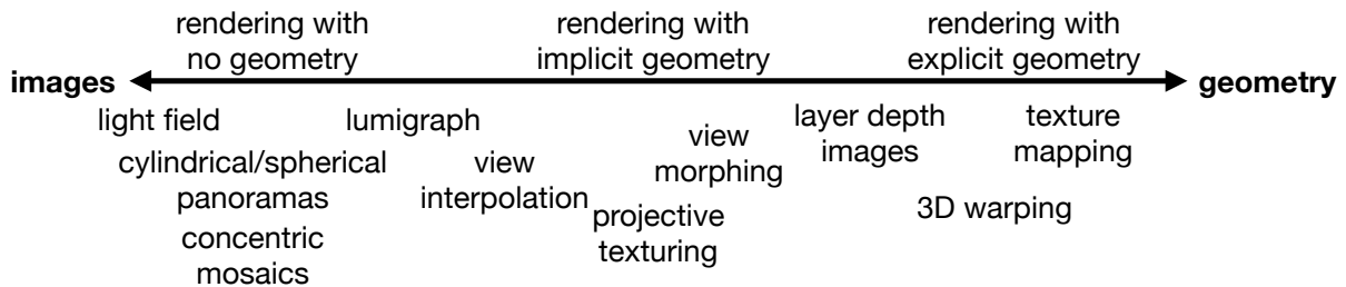
Figure 2.36: Image-Based Rendering techniques classified in the image-geometry spectrum. Diagram is adapted from Oliveira (2002) and Shum and Kang (2000).
