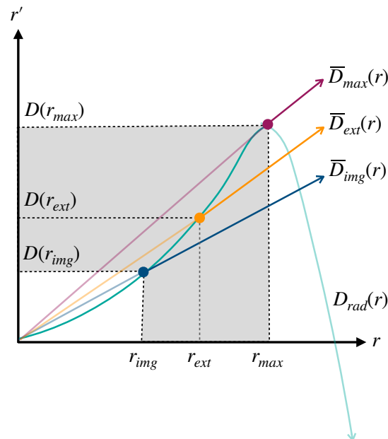
Figure 4.9: Sample behavior of the distortion model.
