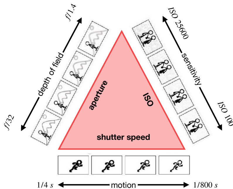
Figure 2.6: The exposure triangle: aperture, shutter speed, and ISO must be balanced in the photographic process. The diagram has been adapted from Verhoeven (2016).
