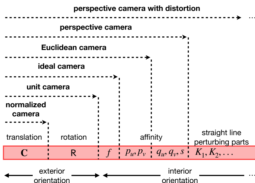
Figure 4.1: Overview of different camera models used to map 3D space points into a 2D image. Diagram is adapted from Förstner and Wrobel (2016).
