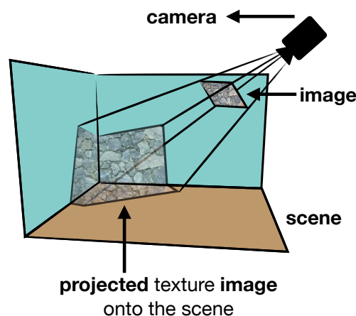
Figure 2.37: Projective texturing over a 3D scene, adapted from Segal et al. (1992).
