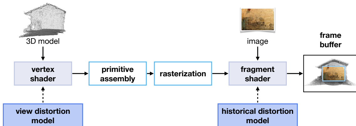
Figure 4.6: One-pass rendering, where the distortion is applied to the vertices of the scene and the reprojection of the image.
