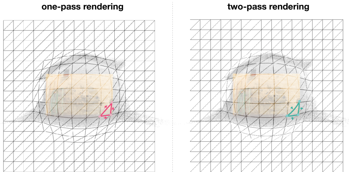
Figure 4.13: One-pass vs. two-pass Rendering. Comparison between the two rendering pipelines. A wireframe tessellated plane has been put in front of the view for illustrative purposes.
