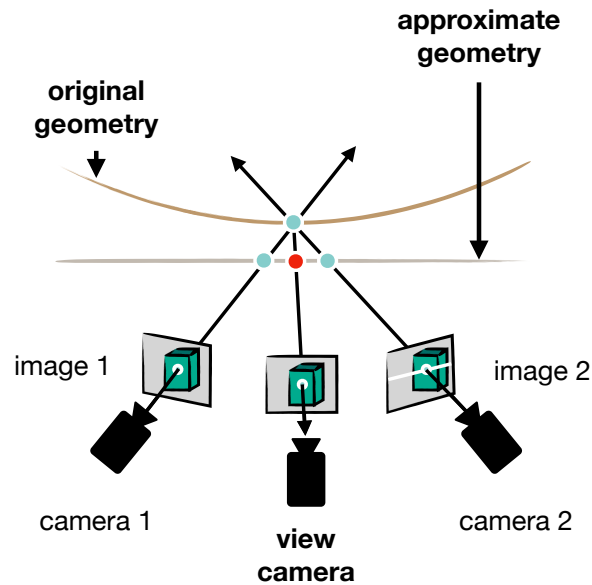
Figure 2.43: Uncertainty in multi-view projective texturing with approximate scene geometry. Figure adapted from Eisemann, De Decker, et al. (2008).
