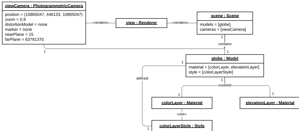
Figure 6.16: UML object diagram of HISTOVIS from the initial state. It depicts the configuration of the system’s engine (presenting the 3D environment to the user in the GUI).
