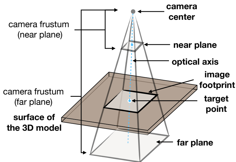
Figure 3.7: Geometrical components defined in the projection of a 2D image on the top of a 3D model.
