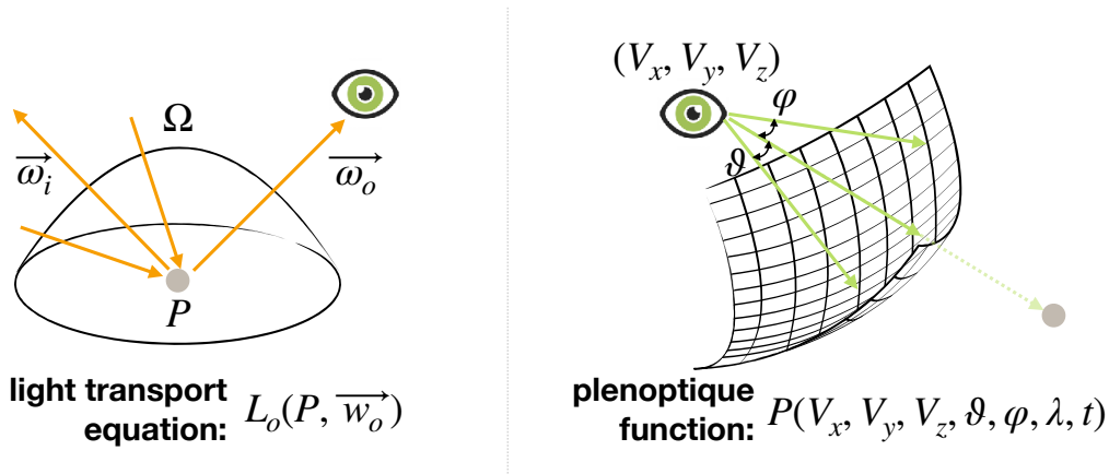
Figure 2.35: Different rendering equations. Left: Light transport equation. The radiance at a specific point P from a view direction w_o is defined by the outgoing light L_o (Immel, Cohen, and Greenberg 1986). Right: Plenoptic function. It describes all of the image information visible from a particular viewing position (McMillan and Bishop 1995).
