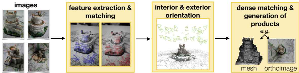
Figure 2.10: Process of photogrammetry (main steps): (i) feature extraction & matching; (ii) interior & exterior orientation; (iii) dense matching & generation of products. Images depicting Tvrdava Minčeta tower (Dubrovnik).
