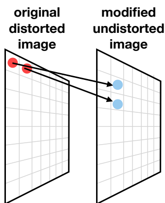
Figure 2.46: The mapping of the distorted and undistorted version of the image (Vass and Perlaki 2003).
