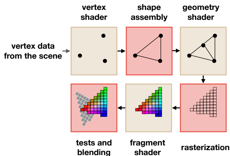
Figure 3.5: Shading process. Three shaders are applied: vertex, geometry, and fragment. The diagram is adapted from Vries (2020).
