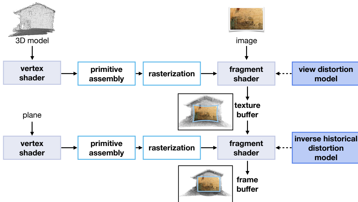
Figure 4.7: Two-pass rendering, where in the first pass, the image is undistorted. In a second pass, the inverse distortion is employed to distort the whole view.
