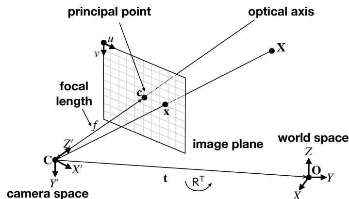
Figure 2.11: The pinhole camera model (geometric representation). Diagram adapted from Moulon (2014).
