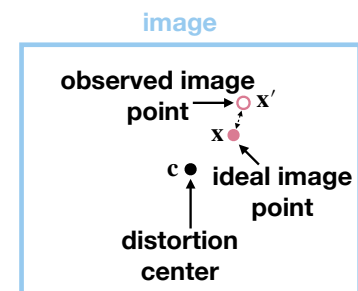
Figure 4.3: Depiction of an ideal image point and its distorted variant.
