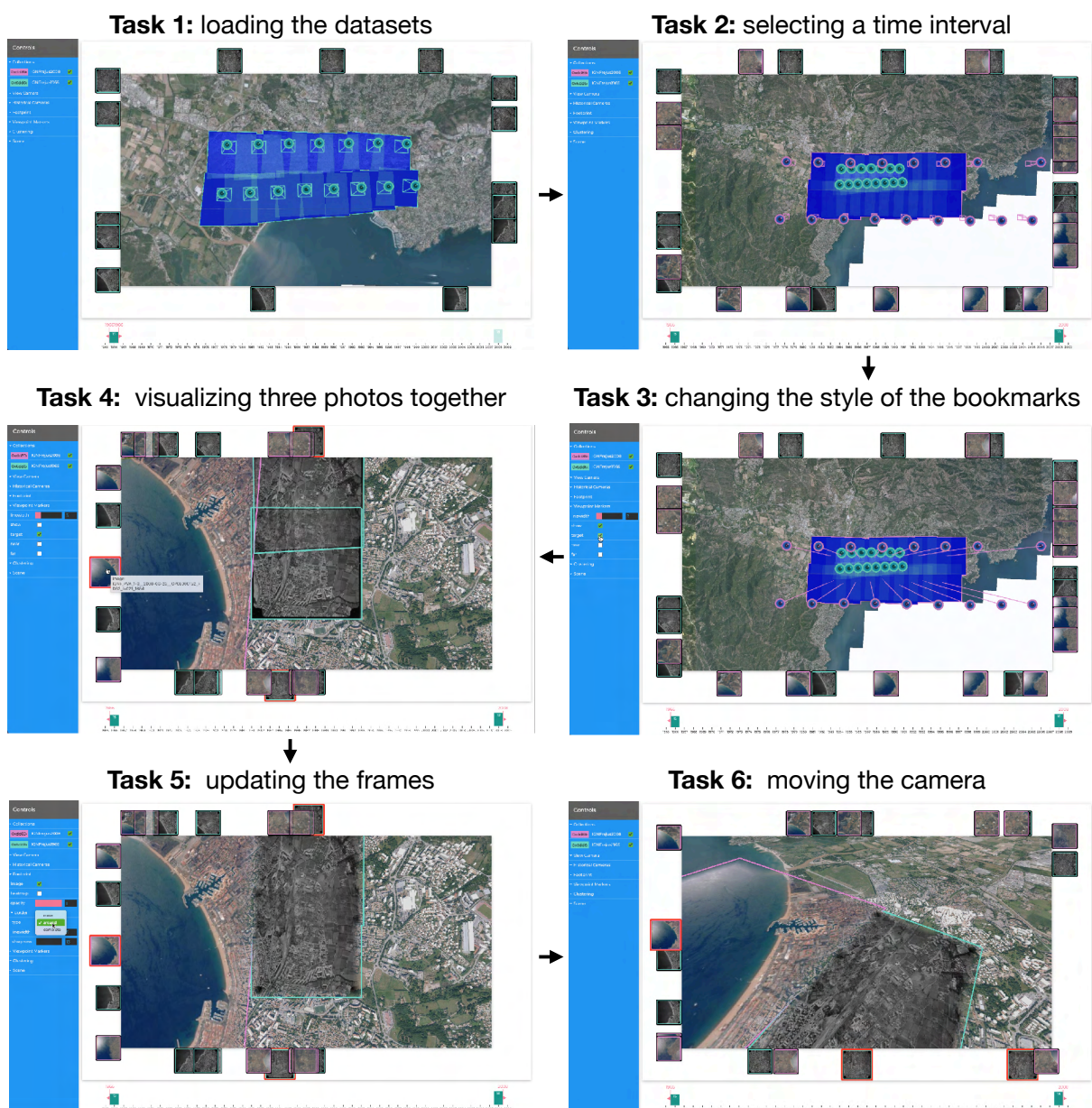
Figure 6.26: Use case scenario 1: visualization of two photo collections. Credits to IGN/Frejus collection.
