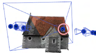
frustum + projection
