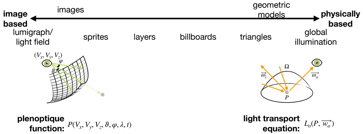
Figure 3.6: Rendering spectrum, adapted from Akenine-Möller, Haines, and Hoffman (2019). It reveals a progression in the rendering techniques that increasingly decouples itself from geometry (right to left).
