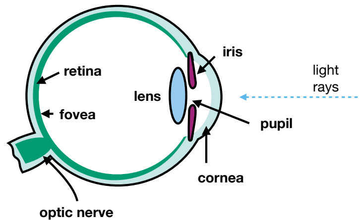
Figure 2.51: Elements inside the human eye. The light enters through the pupil and forms an image in the retina. Figure adapted from Snowden, Thompson, and Troscianko (2011).
