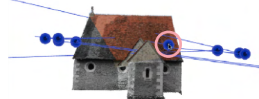
ray + projection
