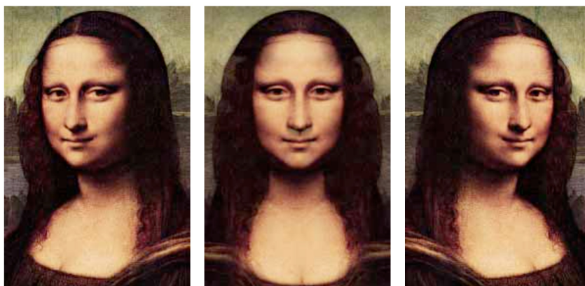
Figure 2.41: Mona Lisa View Morphing. The morphed view (center) is halfway between the original image (left) and its reflection (right) (S. Seitz and Dyer 1996).
