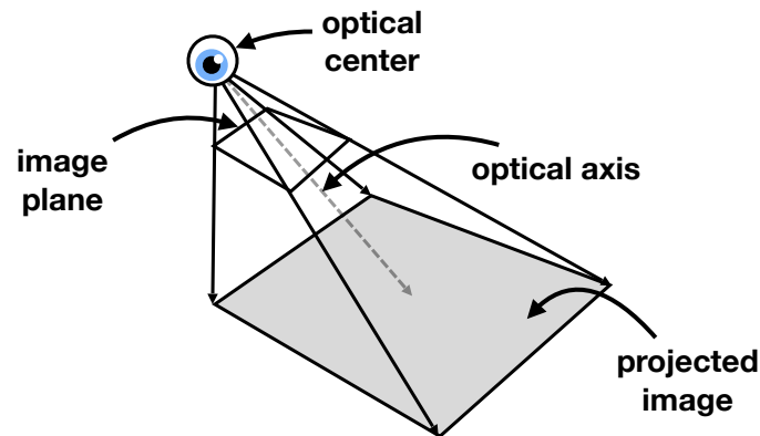
Figure 5.6: Our bookmark having: optical center, optical axis, image plane, etc.
