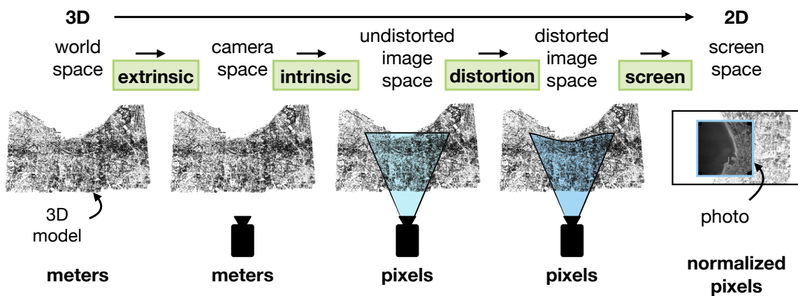
Figure 4.5: Rendering with distortion. Our desired mapping from 3D to 2D for the view camera. It follows a camera model with distortion.
