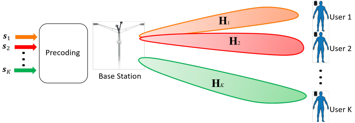
Figure 3.1: Single cell broadcast channel system model.
