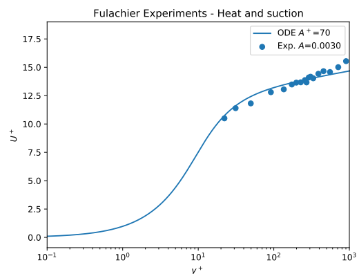
(f) U^+ as function of y^+ , A = 0.0030 , A^+ = 75
