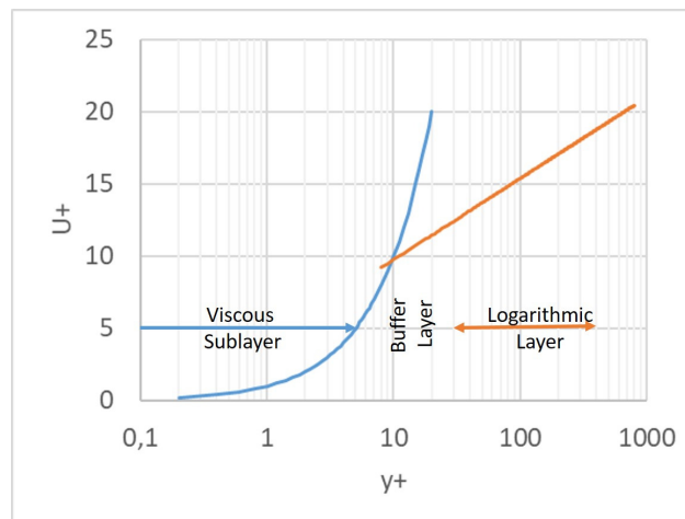
Figure 2.2: Wall function for an incompressible, isothermal flow with no pressure gradient.
