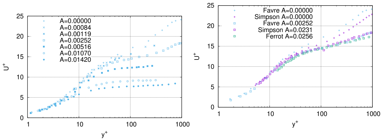
(a) Wall law measured in [Favre et al., 1966] with different suction rate. (b) Wall law measured in [Favre et al., 1966; Simpson, 1968; Ferro, 2017] for similar suction rates.
