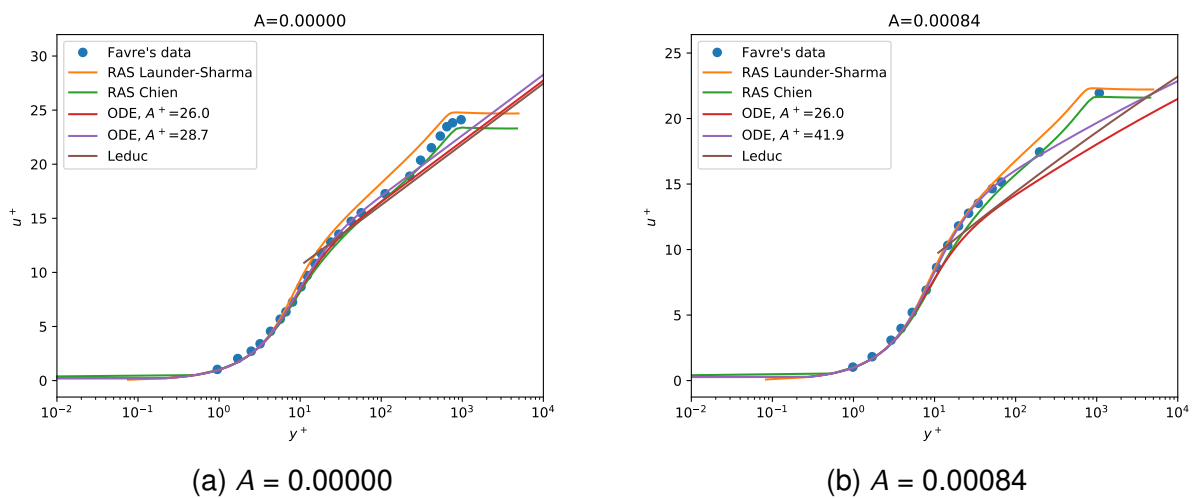
Figure 5.2: Velocity profiles for Favre's experimental data, RAS results using Launder-Sharma and Chien's model, Leduc's analytical model in inertial sub-layer and ODE solution with the no-suction A^+ = 26 and the best-fit damping factor constants: part 1
