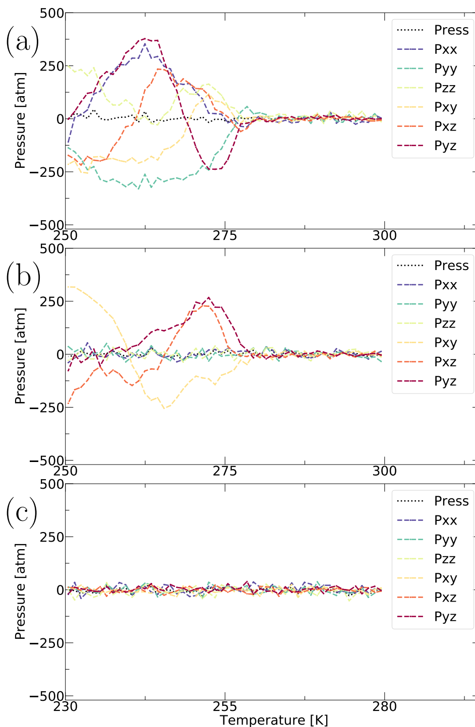
Figure 4.21: The pressure tensor components as function of the imposed temperature during the constant cooling at the rate 2 K/ns for the chain length of 400 beads. The plots corresponds to: (a) isotropic, (b) anisotropic and (c) triclinic methods to control the pressure components.
