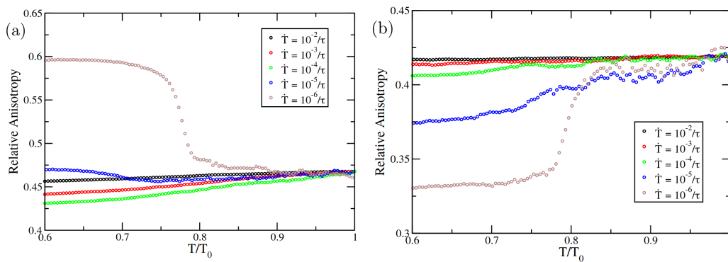
Figure 3.9: The relative shape anisotropy for polymers of (a) 100 and (b) 1000 monomers during cooling.
