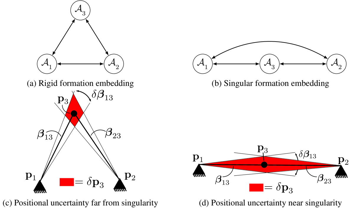
Figure 7.3 – Rigid and singular configurations of a 3-robot bearing-based formation, with their corresponding constraints and region of uncertainty. For simplicity, agent \mathcal{A}_1 and \mathcal{A}_2 are fixed in position.
