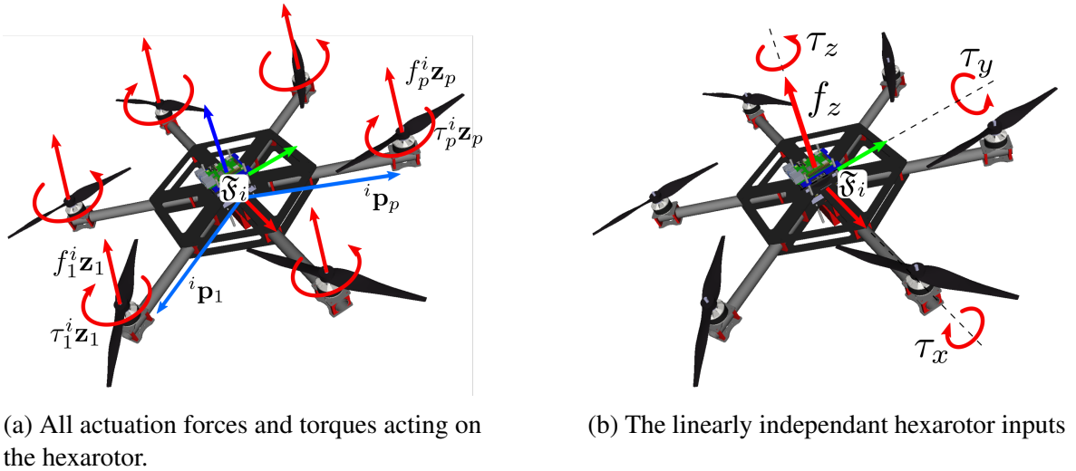
Figure 2.7 – The actuation of an underactuated hexarotor.
