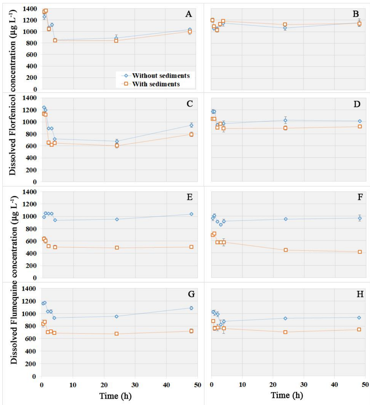
Figure 1. Florfenicol and flumequine dissolved concentrations (average \pm SD) in batch experiments with (orange square) and without (blue diamond) added marine sediments: A) and E) eutrophic water at 8°C; B) and F) pure water at 15°C; C) and G) Seawater at 8°C and D) and H) Seawater 15°C.
