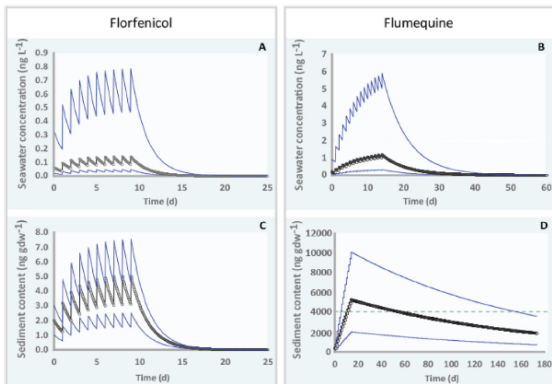
Fig. 3. Simulation of consecutive treatments with florfenicol and flumequine in salmon cages with predicted water column concentrations (A, B) and sediment content (C, D) after addition of antibiotics. Black lines show average values predicted by the scenario of average salmon density of 14 \text{ kg m}^{-3} within the minimum and maximum permitted salmon density in cages (blue lines, 11 and 17 \text{ kg fish m}^{-3} ). The horizontal green dotted line shows sub-MIC threshold in surface sediment. (For interpretation of the references to colour in this figure legend, the reader is referred to the Web version of this article.)
