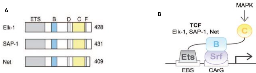
Figure 36: Srf co-factors.
