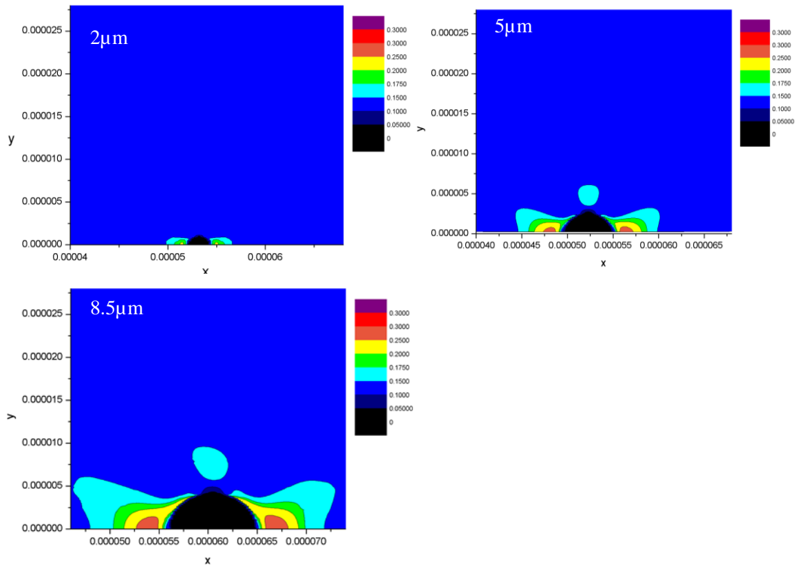
Figure 1130: Repartition of the plastic strain around SiO 2 inclusions with different sizes
