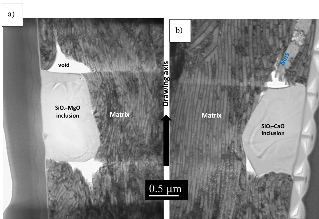
Figure 974: Overview of the inclusion into the deformed microstructure ( \epsilon \approx 1 ) observed with TEM a) \text{SiO}_2\text{-MgO} b) \text{SiO}_2\text{-CaO}
