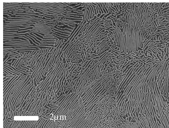
Figure 2 : SEM images of a fully pearlitic structure in a hypereutectoid steel
