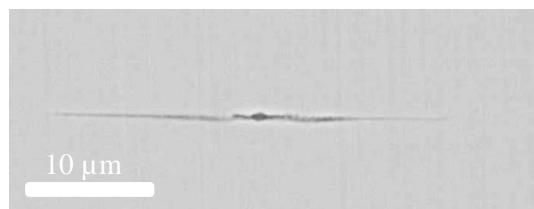
Figure 895: Example of a micro-crack longer than 15µm
