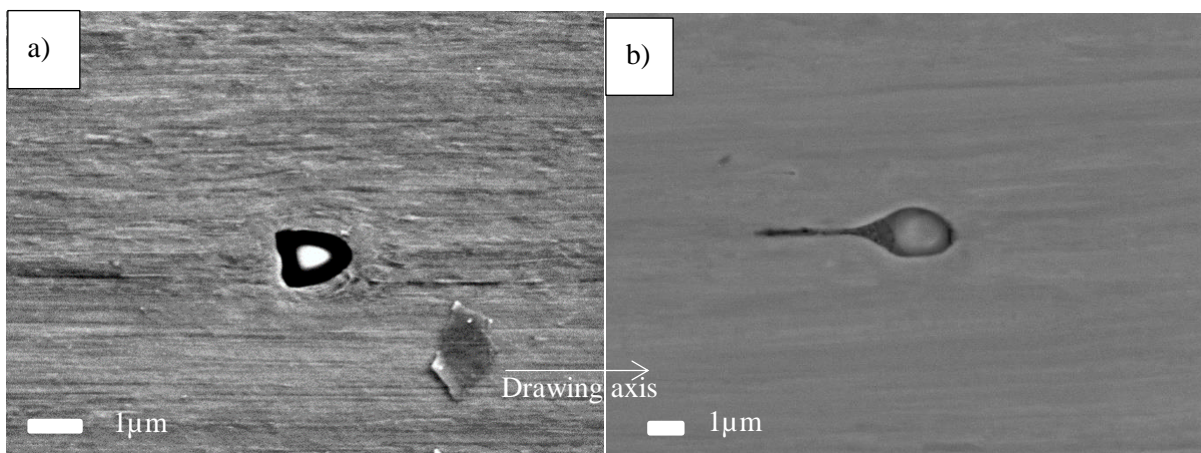
Figure 89: SEM picture of inclusions a) embedded in the matrix without cracking b) inducing a micro-crack
