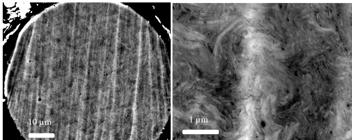
Figure 1218: BSE images of the cross section of a 60\mu\text{m} filament showing heavily deformed microstructure
