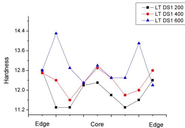
Figure 88 Influence of drawing speed on hardness profile of LT filament
