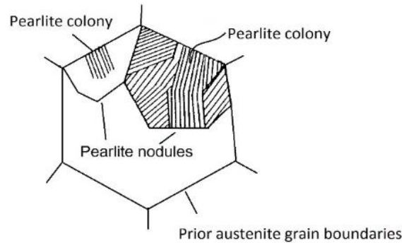
Figure 3 : Schematic of pearlitic structure[6]
