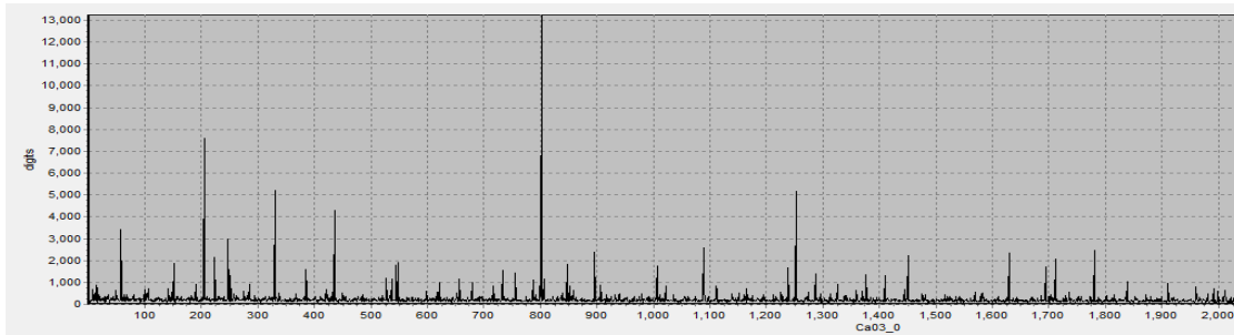
Figure 40: Example of Ca spark-by-spark chart
