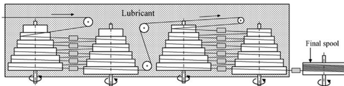
Figure 9: Schematic of a wet wire drawing machine [13]
