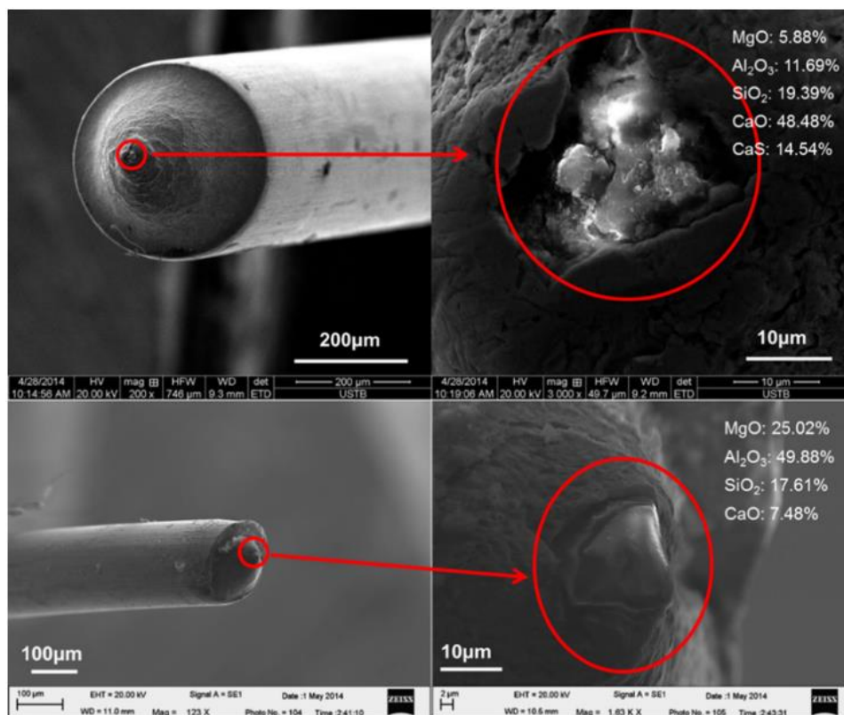
Figure 25 : Example of fracture due to inclusions on Ø0.20mm wires [27]
