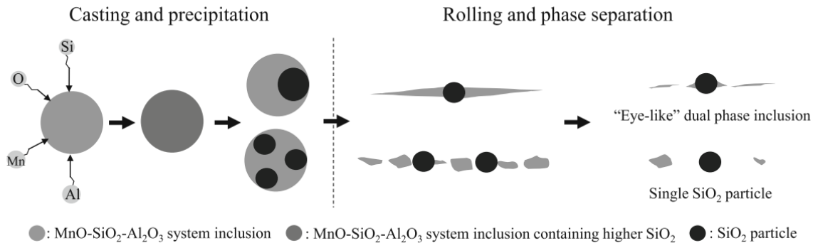
Figure 18 : Schematic diagram of formation mechanism of \text{SiO}_2 -type inclusions in wire rods [25]
