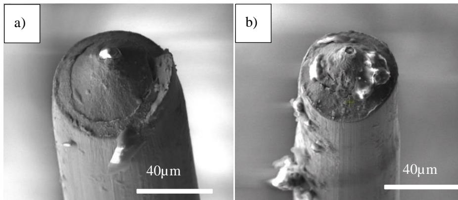
Figure 63 : Fracture presenting a necking a) with inclusion b) with a hole due to the presence of an inclusion
