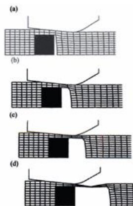
Figure 32 : coalescence and growth of defect during wire drawing as the draw length increases [67]
