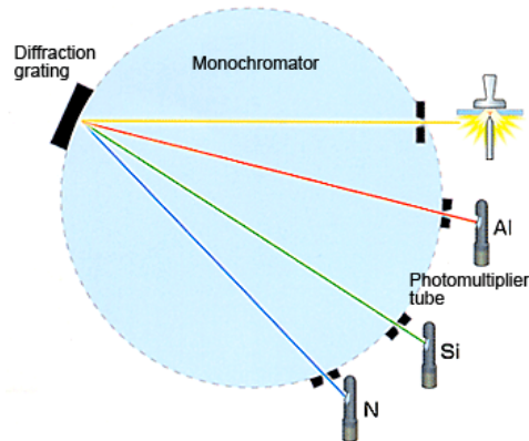
Figure 36 : Schematic illustration of OES/PDA [70]
