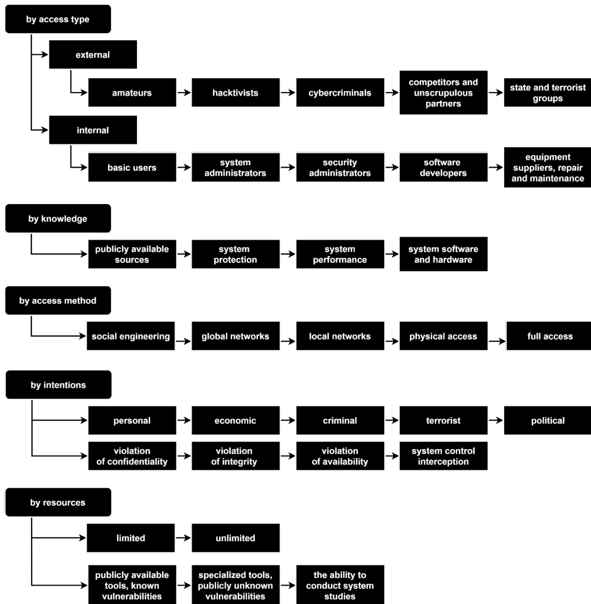
Figure 3. Classification of the attacker
