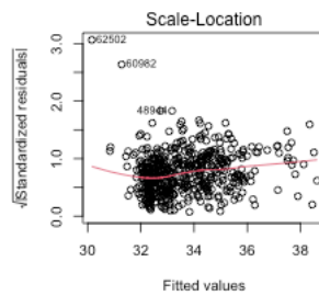
Figure F2. Diagnostic plots of linear model for the sampled climate experiment at Nouragues, with each summary statistics as dependent variables and the three climatic variables (temperature, irradiance and VPD) as independent variables. The four graphs represent, respectively, residual linearity, residual normality, residual homoscedasticity, and presence or absence of leverage points (influential points).
