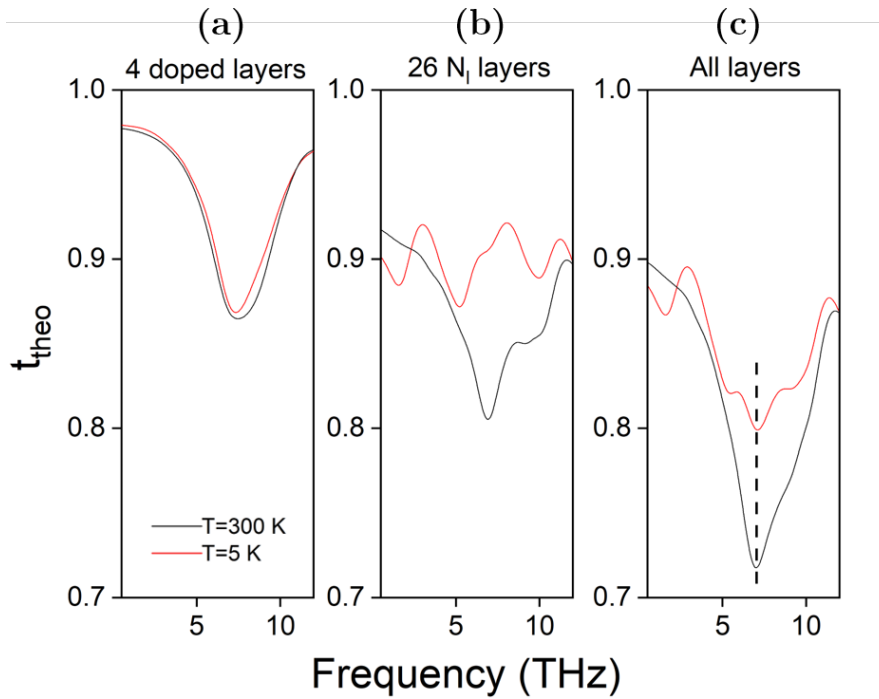
Figure 2.41: Computed transmittance t_{\text{theo}} at T=5\text{K} (red curves) and T=300\text{K} (black curve) for different compositions of the GQD: (a) only 4 doped layers, (b) only 26 layers with E_F = 20\text{ meV} and (c) full stacking: sample C2.
