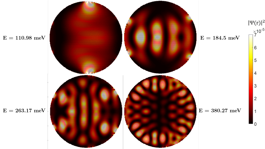
Figure 1.18: Probability density (right color bar) for few states lying in the quasi-continuum of energy levels above the dashed line in Figure 1.9, for GQD of radius 25 nm with their respective energy. |\Psi(\mathbf{r})|^2 is high for some armchair borders and extends from these parts into the bulk part of the dot.
