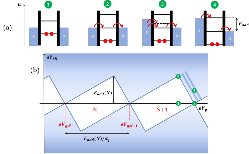
Figure 3.13: Scheme of four different configurations of the GQD (a) corresponding to different points in the stability diagram (b). Red arrows indicate an electron flux. (1)-(2) When source and drain electrochemical potentials are aligned ( V_{SD} = 0 ), a tunnelling transport occurs only if an empty single-energy level crosses \mu_{S/D} . (3) Different transport channels lie within the transport window \mu_S - \mu_D , resulting in lines of enhanced current (4) The bias equals to the addition energy.
