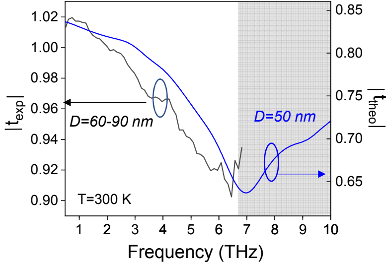
Figure 2.35: Comparison between experimental t_{exp} (black curve, left y-axis) and computed t_{theo} (blue curve, right y-axis) transmittance of Sample C1, at T = 300 K. For t_{theo} , \Gamma is fixed to 1 THz = 4.1 meV.
