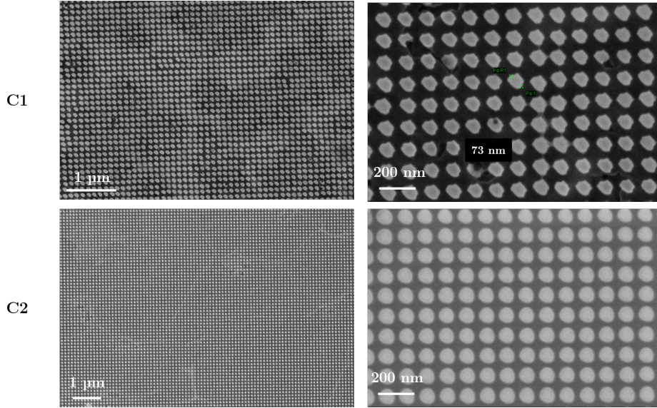
Figure 2.27: SEM images of Sample C1 and C2 on large (left) and lower scale (right), on different areas. At large and low scale, no defect is observed in the structure, and the GQDs are uniform in size and well defined for both samples.
