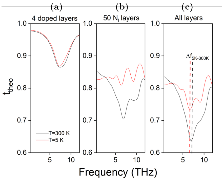
Figure 2.40: Computed transmittance t_{\text{theo}} at T=5\text{K} (red curves) and T=300\text{K} (black curve) for different compositions of the GQD: (a) only 4 doped layers, (b) only 50 layers with E_F = 0\text{ meV} and (c) full stacking: sample C1.
