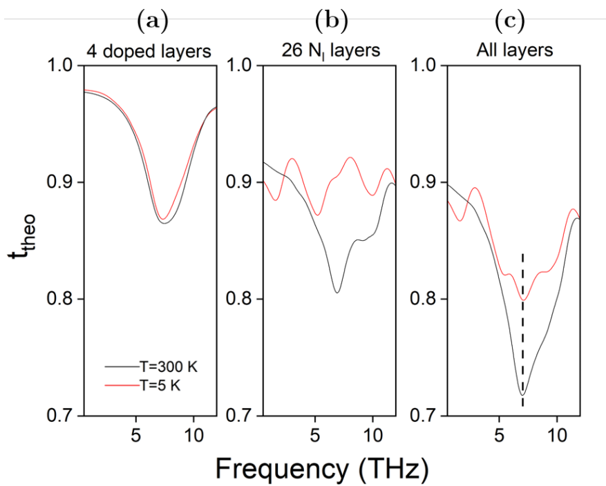
Figure 2.41: Computed transmittance t_{\text{theo}} at T=5\text{K} (red curves) and T=300\text{K} (black curve) for different compositions of the GQD: (a) only 4 doped layers, (b) only 26 layers with E_F = 20\text{ meV} and (c) full stacking: sample C2.
