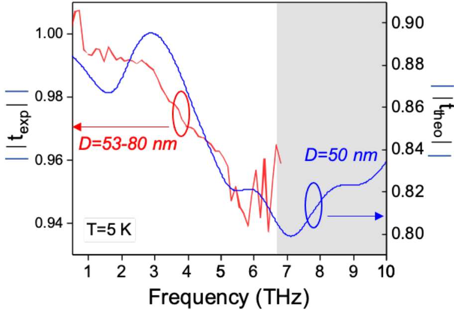
Figure 2.39: Comparison between experimental t_{exp} (red curve, left y-axis) and computed t_{theo} (blue curve, right y-axis) transmittance of Sample C2, at T = 5 K. For t_{theo} , \Gamma is fixed to 1 THz = 4.1 meV.
