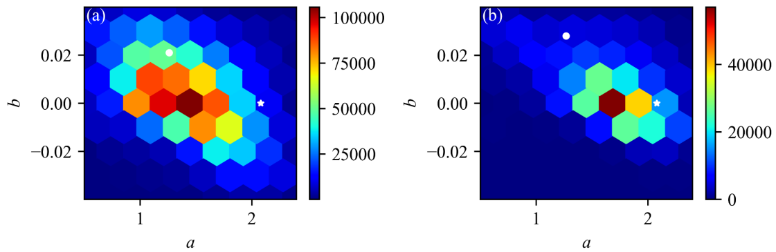
Figure 6.7 Distribution of the linear regression coefficients ( i.e. slope a and intercept b ) in Eq.(6.5) from (a) Sentinel-2; (b) Landsat-8. Coefficients are calculated pixel-wise, and the mean value is aggregated over the whole image. A white circle highlights the spectral correlation coefficient c derived from the field measured data, and a white star highlights the c of the original EVI2 [106]. The range of a and b is limited at [0.5, 2.4] ( x -axis) and [-0.04, 0.04] ( y -axis) for a better visual effect.
