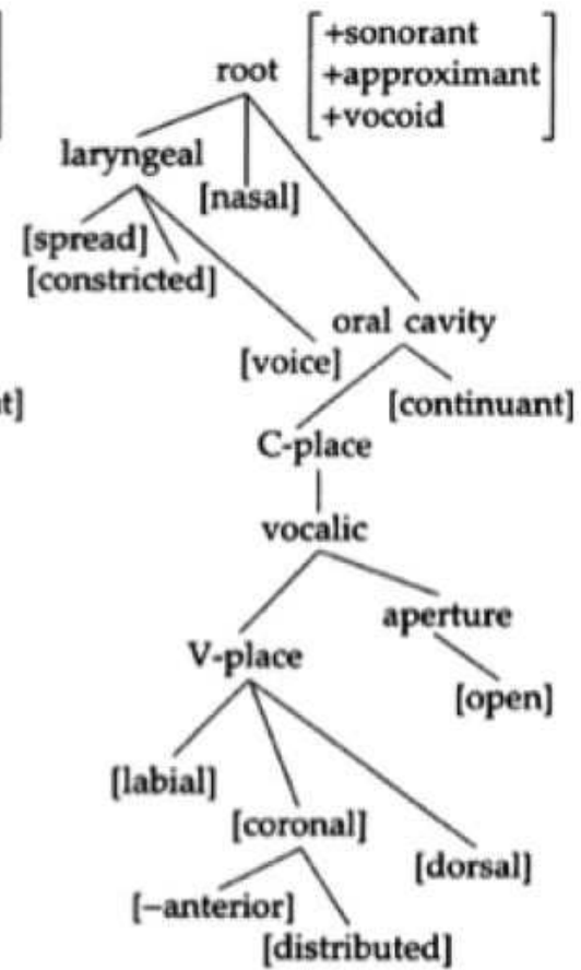
(b) Vocoids:
