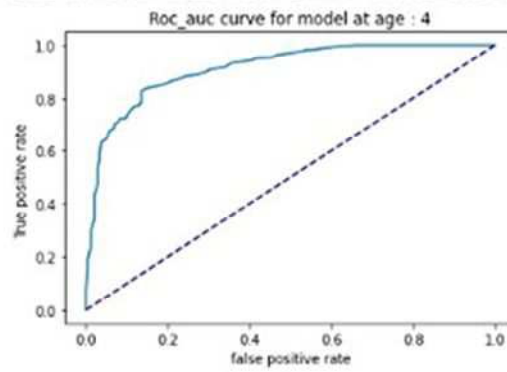
Figure 52 : Correctness's measure of the model at different ages
