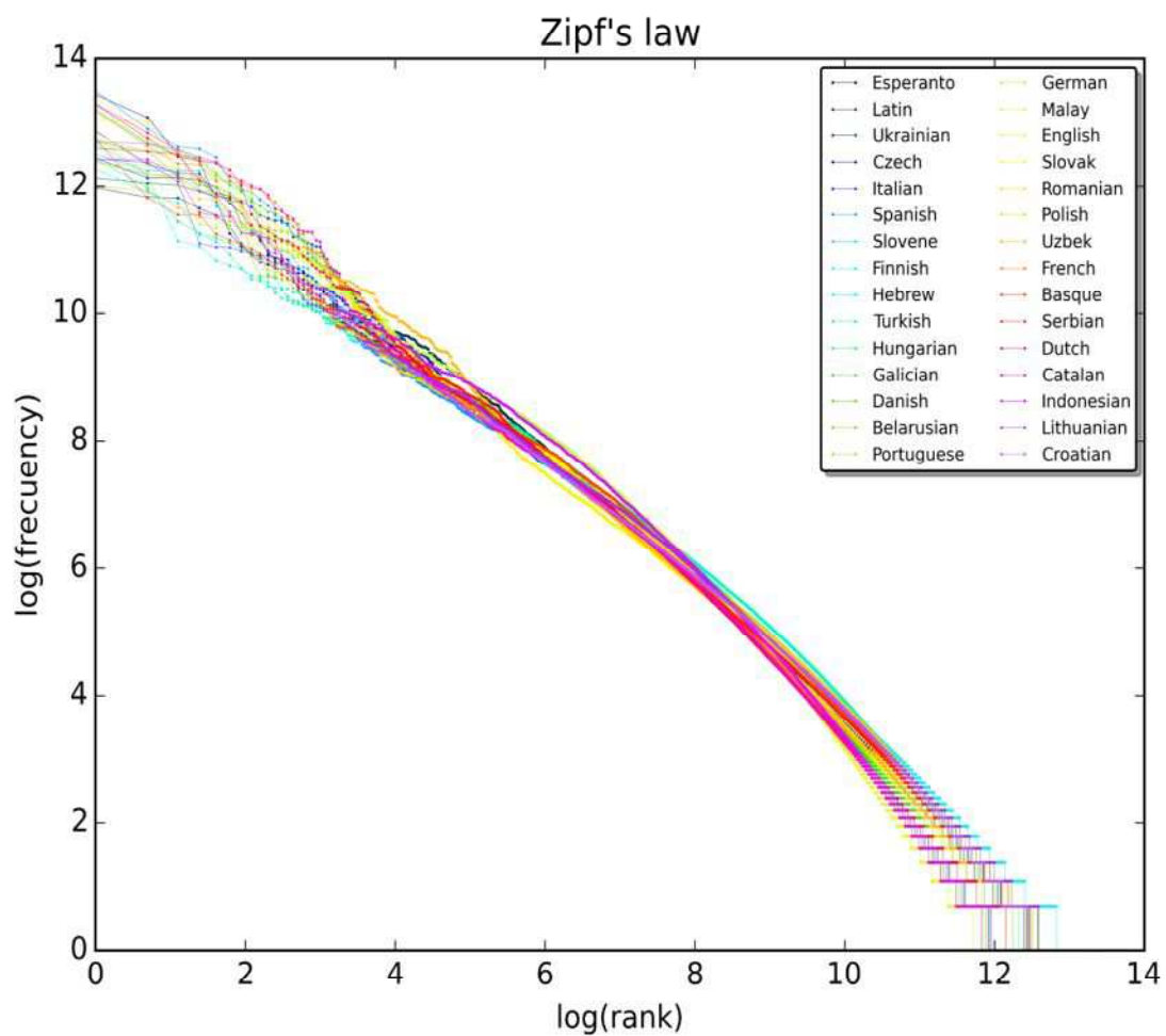
Figure 2 16 : Zip's law
