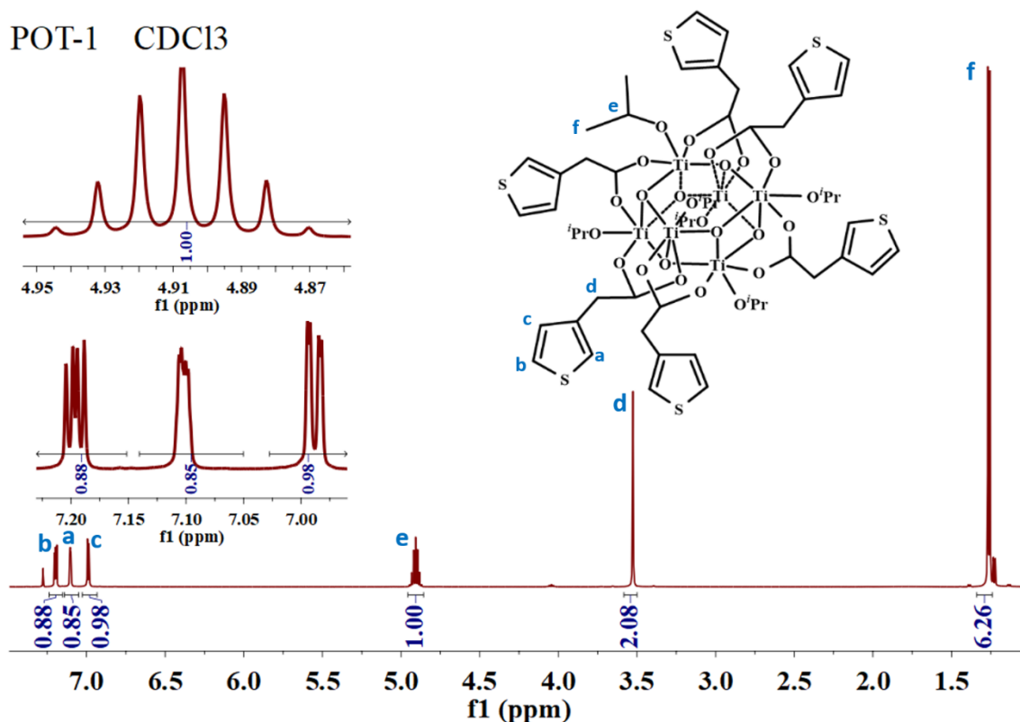
Figure 18. The 1 H NMR of POT-1 in CDCl 3 .
