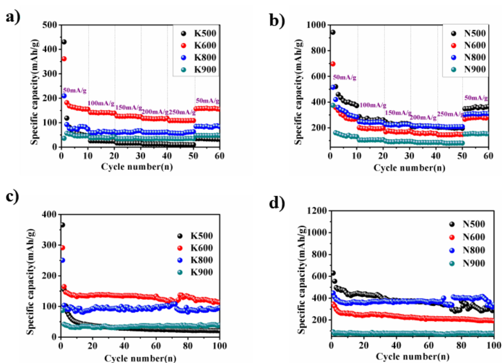
Figure 44. Rate capability diagrams of (a) K500 , K600 , K800 , K900 and (b) N500 , N600 , N800 , N900 at different current densities, cycling stability of (c) K500 , K600 , K800 , K900 and (d) N500 , N600 , N800 , N900 .
