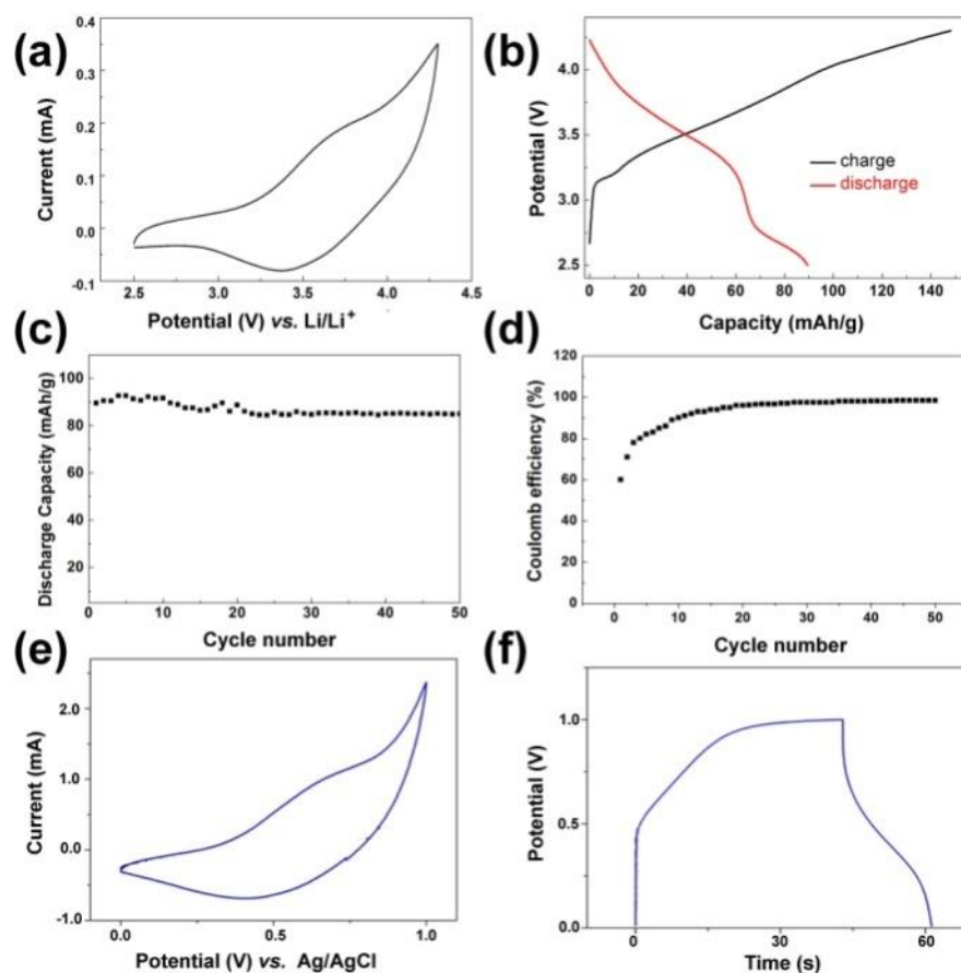
Figure 66. (a) CV curve of the PTEPA electrode in \text{LiPF}_6 EC/DMC (v/v, 1:1) electrolyte versus \text{Li/Li}^+ , at a scan rate of 1 mV/s; (b) Initial charge-discharge curves of the PTEPA electrode at a current density of 20 mA/g; (c) Cycling stability of the PTEPA electrode at a current density of 20 mA/g; (d) Coulombic Efficiency of the PTEPA electrode; (e) CV curve of the PTEPA film in 1 mol/L \text{H}_2\text{SO}_4 aqueous solution versus \text{Ag/AgCl} , at a scan rate of 100 mV/s (f) GCD curves of the PTEPA film in 1 mol/L \text{H}_2\text{SO}_4 aqueous solution at approximately 10 A/g.
