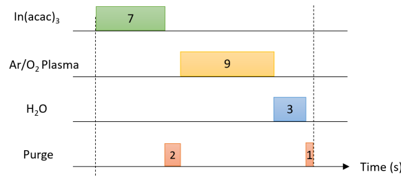
Figure 6.15: ALD cycle used to achieve 34 pm/cycle growth rate with \text{In}(\text{acac})_3 , \text{H}_2\text{O} and \text{Ar}/\text{O}_2 plasma.
