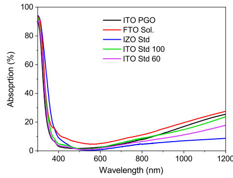
Figure 5.18: Absorption spectra of TEC-7 substrate (FTO) compared to ITO PGO, IZO, ITO Std 100 and 60 on 3 mm soda-lime glass.
