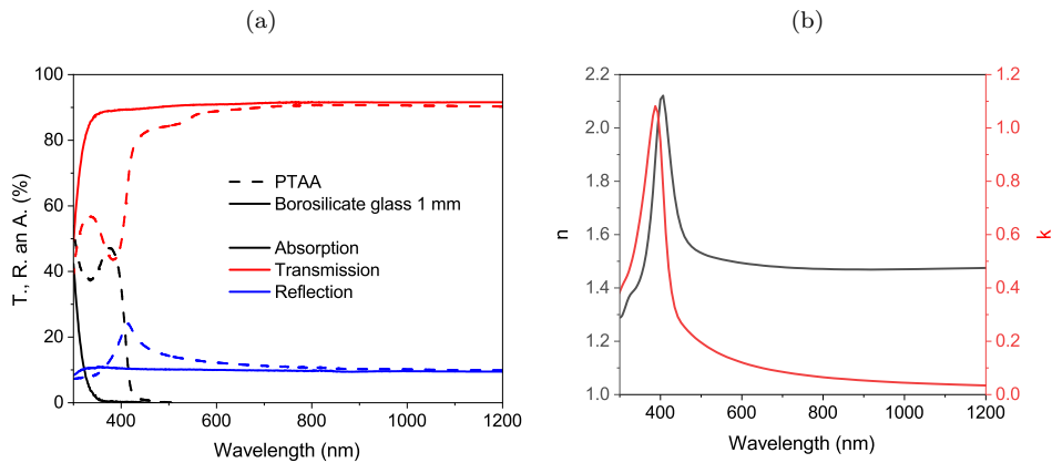
Figure 5.1: (a) Transmission, absorption and reflection spectra of PTAA on a 1 mm thick borosilicate glass, compared to the substrate alone. (a) Optical indices n and k of PTAA.
