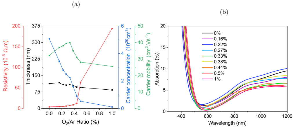
Figure 6.5: Evolution of (a) thickness (black), resistivity (red), carrier concentration (blue), carrier mobility (green) and (b) absorption of IZO layer as function of the ratio between oxygen and argon during sputtering deposition.
