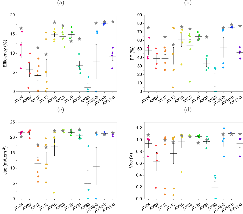
Figure 3.5: Dispersion of the electrical properties (a) efficiency, (b) FF, (c) Jsc and (d) Voc of STPC from different batch. Grey star represents the average of opaque perovskite cell values for the same batch.
