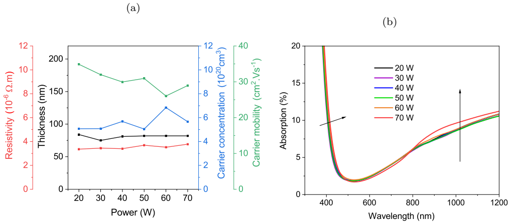
Figure 6.4: Evolution of (a) thickness (black), resistivity (red), carrier concentration (blue), carrier mobility (green) and (b) absorption of IZO layer as function of the power used on the IZO target.
