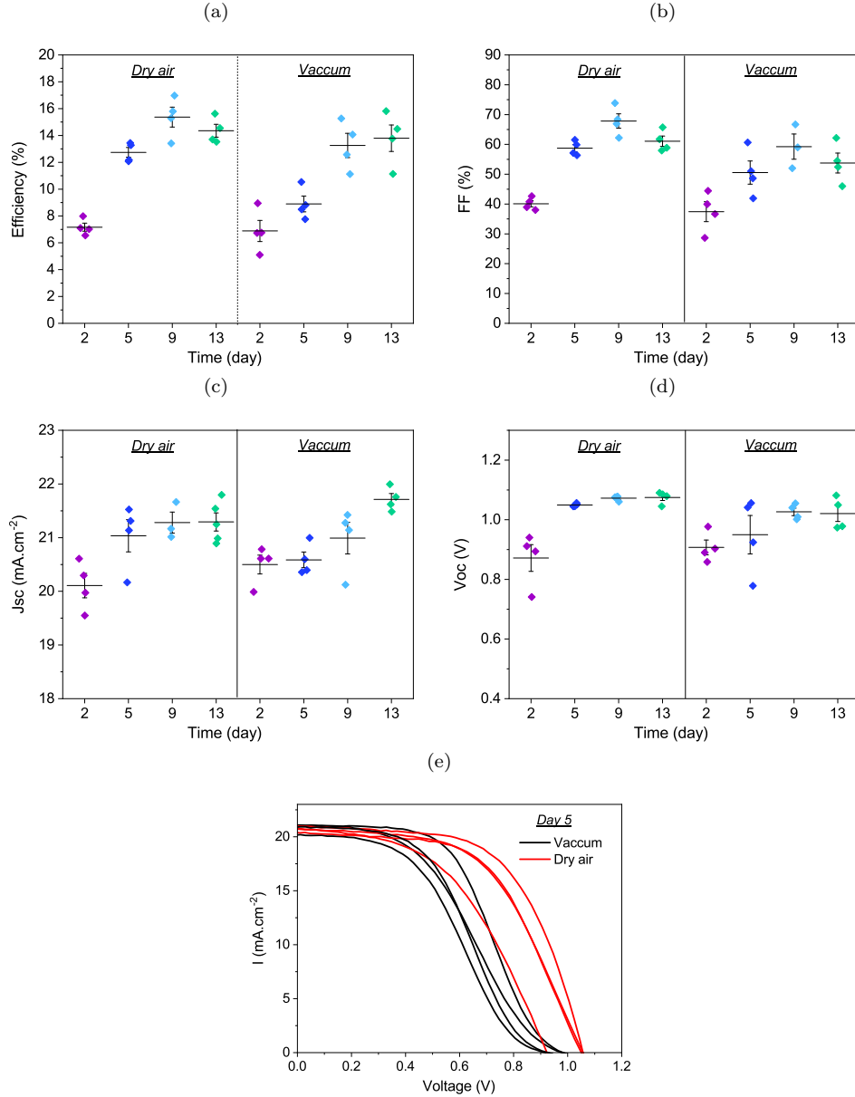
Figure 5.10: Dispersion of the electrical properties ((a) efficiency, (b) FF, (c) Jsc and (d) Voc) of AY45 STPC with PTAA as HTL, stored under vacuum or in dry air after ITO deposition, second day after the synthesis, 5, 9 and 13 days later. (e) IV RV curves of AY45 STPC with PTAA as HTL, stored under vacuum or in dry air after ITO deposition, 5 days after the synthesis.
