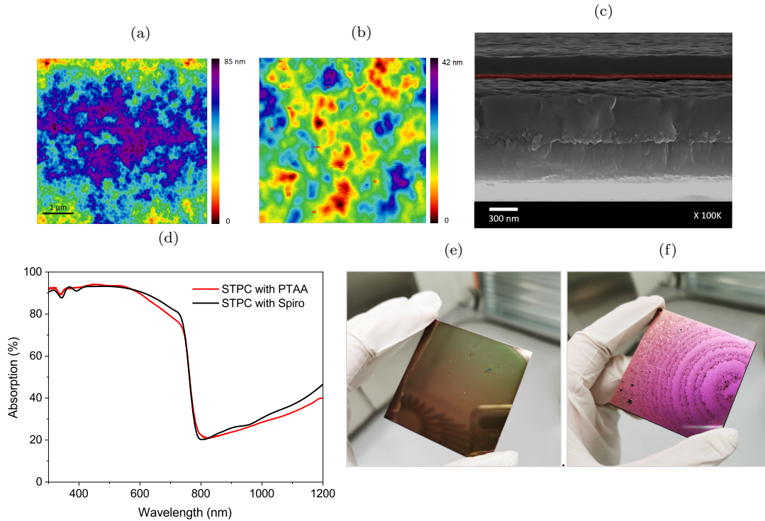
Figure 5.2: AFM of the ITO surface of a STPC with (a) PTAA and (b) Spiro-OMeTAD as HTL. (c) SEM cross-section image of a STPC with PTAA as HTL (red area). (d) Absorption spectra of two STPC with PTAA or Spiro-OMeTAD as HTL. Pictures of complete STPC stacks on 16 cm 2 just after ITO deposition with (e) PTAA and (f) Spiro-OMeTAD as HTL.
