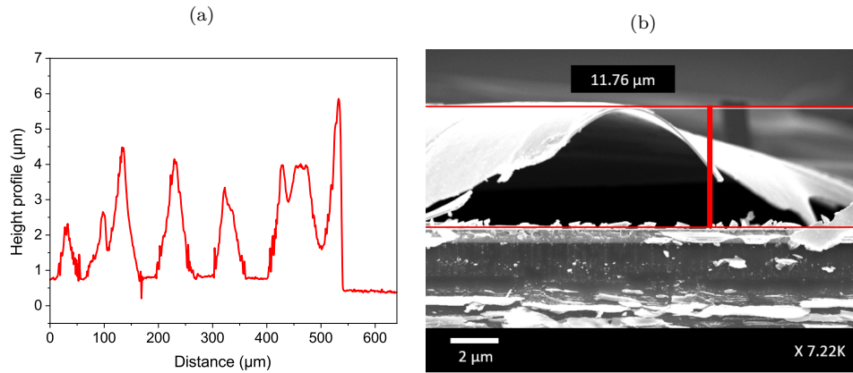
Figure 3.9: (a) Confocal Microscopy measurement of roughness at the ITO surface of STPC after annealing. (b) SEM cross-section of a STPC after annealing.
