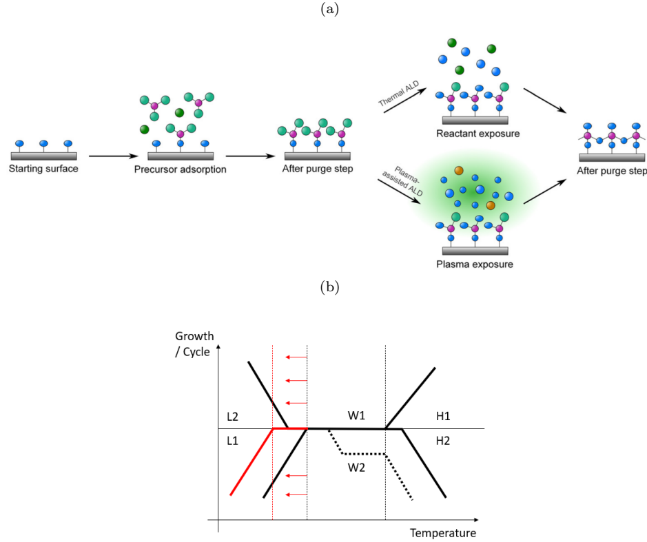
Figure 2.7: (a) Schematic representation of thermal ALD and plasma enhanced ALD. During the co-reactant step of the cycle, the surface is exposed to a reactant gas or vapor, or to species generated by a plasma [211]. (b) Comparison of the temperature windows of the PEALD and ALD processes. The red dotted line indicates the lower limit of the PEALD window, and the solid black lines the ALD window. [212].
