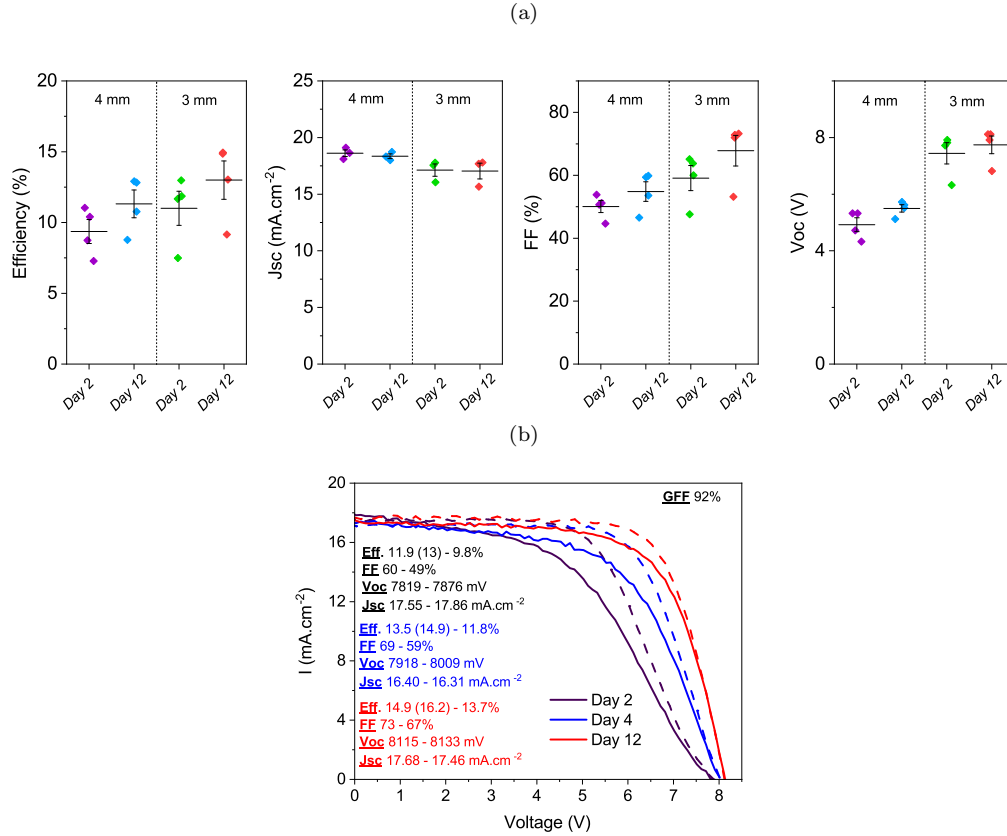
Figure 7.19: Dispersion of the electrical properties of MA19 STPM with sub-cell widths of 4 or 3 mm. (b) IV curves of the best 4.2 \text{cm}^2 STPM obtained (MA19-14), 2, 4 and 12 days after the synthesis.
