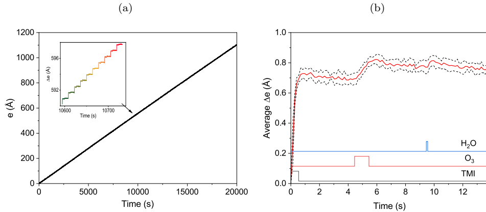
Figure 6.23: (a) Thickness determined by QCM, of ALD \text{In}_2\text{O}_3 films deposited with \text{O}_3 and \text{H}_2\text{O} as reactants during 1000 cycles. Zoom is made on 10 cycles in the middle of the deposit. (b) Average on the 10 cycles presented in (a) of the evolution of the thickness in red plot, dashed black plot represents the standard deviation.
