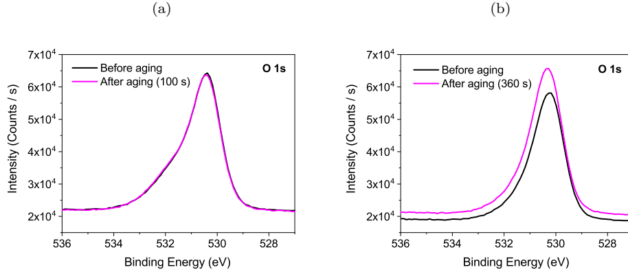
Figure 5.14: XPS spectra of O1s (a) in the ITO layer and (b) at the ITO-PTAA interface (corresponding to 360 s on Fig. 5.12b) first day after the synthesis and 6 days later.
