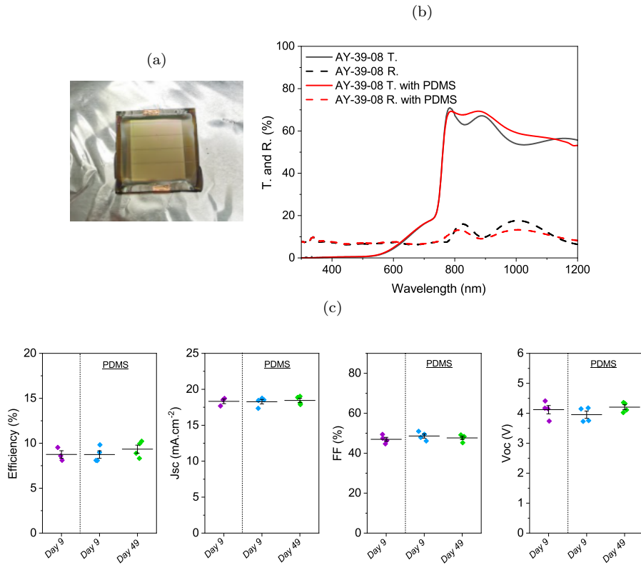
Figure K.1: (a) Photo of a 4 \text{ cm}^2 AY39 STPM, covered by PDMS. (b) Transmission and reflection spectra of AY39-08 STPM before and after the PDMS covering. (c) Dispersion of the electrical properties of AY39 4 \text{ cm}^2 STPM with 4 sub-cell with widths of 5 mm, before and after the covering of PDMS.
