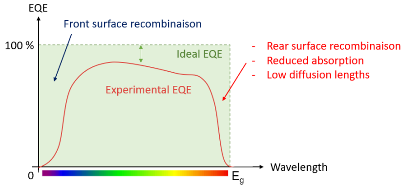
Figure 2.10: Schematic representation of EQE measurement on a solar cell.
