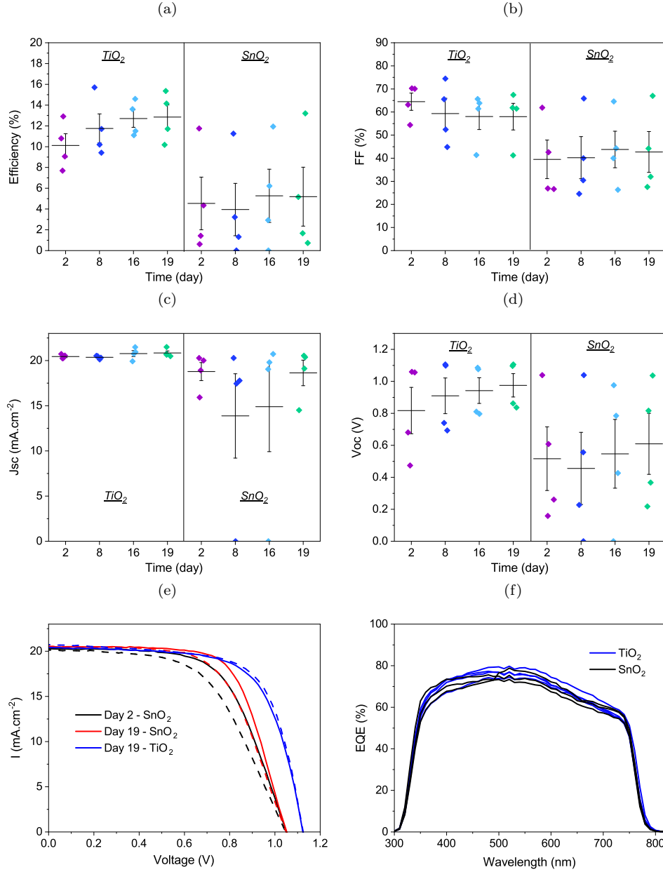
Figure 5.21: Dispersion of the electrical properties ((a) efficiency, (b) FF, (c) J_{sc} and (d) V_{oc} ) of MP39 STPC with \text{TiO}_2 or with \text{SnO}_2 as ETL, second day after the synthesis, 8, 16 and 19 days later. (e) IV curves of MP39-12 STPC with \text{SnO}_2 as ETL, second day after the synthesis, and 19 days later, compared to MP39-08 STPC with \text{TiO}_2 as ETL. (f) EQE spectra of MP39 STPC with \text{TiO}_2 or with \text{SnO}_2 as ETL, made the second day after synthesis.
