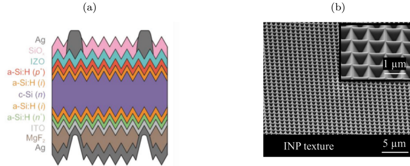
Figure 1.10: (a) Schematic of the infrared-enhanced SHJ cell [66]. (b) Periodic INP gratings of 800 nm pitch were fabricated by NIL [70].
