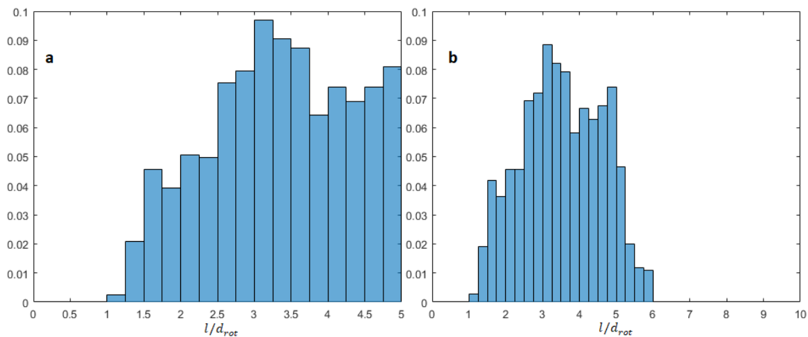
Figure 5.8. Distribution of the interparticle spacing in the case of PNT57 particles for Re = 116 and X/H = 1000 , for two different values of the critical interparticle spacing ((a) 5d_{rot} and (b) 10d_{rot} ). The y-axis represents the number of spacings over the total number of spacings. The x-axis corresponds to the normalized interparticle spacing ( l/d_{rot} ).
