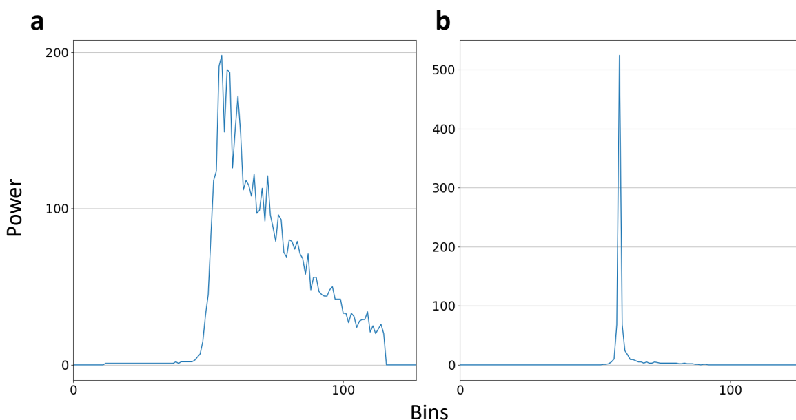
FIGURE II.4: Examples of waveforms from AltiKa altimeter (a) Brownian echo from open ocean. (b) Peak (specular) echo from a lead.
