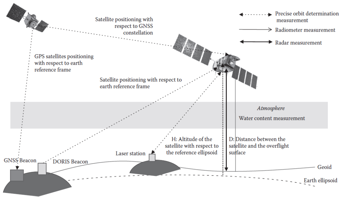
FIGURE .10: Satellite radar altimetry measurement principle : The main sensor used to compute the distance between the satellite and the targeted surface is a radar ; however, to obtain the appropriate measurement accuracy, one needs a radiometer to measure the quantity of water that impacts the atmospheric propagation of the radar signal. To compute the altitude of the satellite with respect to an in situ network that constitutes the Earth reference, sensors onboard the satellite are used in combination with modelling of satellite trajectory to perform the Precise Orbit Determination (POD) of the spacecraft. Figure and caption from Stammer and Cazenave (2018)
