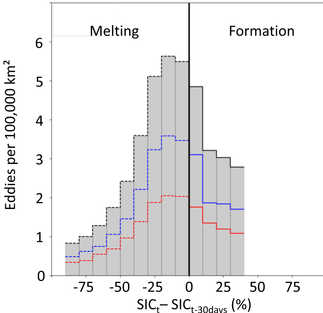
FIGURE IV.7: Presence of eddies within the northern Marginal Ice Zone (n-MIZ). Mean eddy density over the full observation period as a function of the temporal gradient of SIC. Here, this gradient is defined as \delta_t SIC = SIC_t - SIC_{t-30days} . Blue, red and black curves are respectively the density of cyclones, anticyclones, and all eddies. Dashed (plain) lines are the density of eddies in the melting (formation) season.
