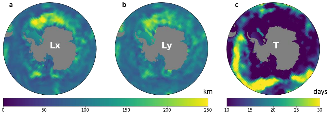
FIGURE II.5: Correlation scales of Sea Level Anomaly computed on GLORYS12 model outputs. (a) Zonal correlation scales. (b) Meridional correlation scales. (c) Temporal correlation scales.
