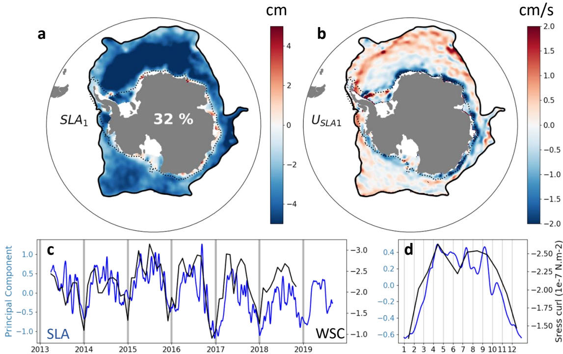
FIGURE III.3: First Sea Level Anomaly (SLA) EOF mode. (a) First SLA EOF mode spatial pattern. The dotted line is the 1000 m isobath; the black line corresponds to the northern boundary of the subpolar sector as defined in Section 2.2. Percentage is the part of total SLA variance explained by this mode. (b) Zonal geostrophic current anomaly associated with SLA mode 1. (c) SLA Mode 1 principal component (blue), and integrated wind stress curl in off-shelf subpolar Southern ocean (black). (d) Same as (c), but for seasonal cycle.
