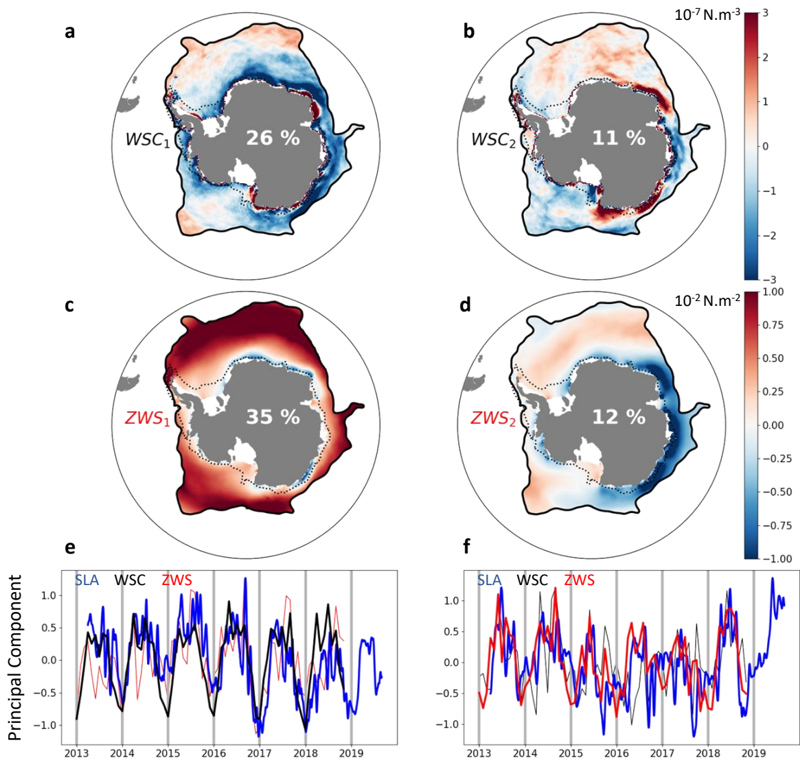
FIGURE III.4: Wind Stress Curl (WSC) and Zonal Wind Stress (ZWS) EOF modes 1 and 2. a,b. Wind stress curl (WSC) EOF modes 1 and 2 spatial patterns. c,d. Zonal wind stress (ZWS) EOF modes 1 and 2 spatial patterns. Percentage is the part of total variable variance explained by this mode. The dotted line on panels a-d is the 1000 m isobath; the black line corresponds to the northern boundary of the subpolar sector as defined in Section 2.2. e. Blue, black and red lines are respectively EOF mode 1 principal components of Sea Level Anomaly (SLA), WSC and ZWS. f. Blue, black and red lines are respectively EOF mode 2 principal components of SLA, WSC and ZWS.
