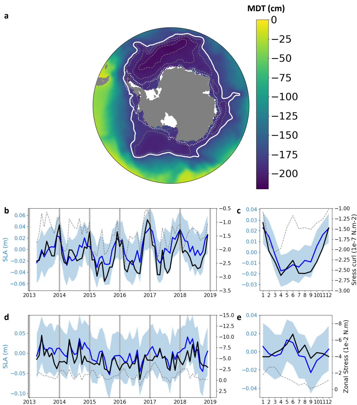
FIGURE III.1: a. Mean Dynamic Topography. The white line is our delimitation of the subpolar Southern Ocean, taken as the northern MDT (Mean Dynamic Topography) contour at -180cm. Black dotted lines are MDT contours of 190, 200 and 210 cm within the subpolar Southern Ocean. The white dotted line is the bathymetry contour at 1000 m and separates on-shelf and off-shelf parts of the subpolar Southern Ocean. b. In blue, time series of integrated off-shelf monthly SLA in the subpolar Southern Ocean. Integrated wind stress curl and ocean stress curl in the same zone are shown in black and dashed grey, respectively. c. Same as a, but averaged over the seasonal cycle. d. In blue, time series of integrated on-shelf monthly SLA in the subpolar Southern Ocean. Integrated zonal wind stress and ocean stress in the same zone are shown in black and dashed grey, respectively. e. Same as c, but averaged over the seasonal cycle. The blue shading shows an upper bound of the error associated with the mean SLA in each sector, derived from the seasonal maps of RMSE between the mapped AltiKa and Cryosat-2 product and independent along-track Sentinel-3A data.
