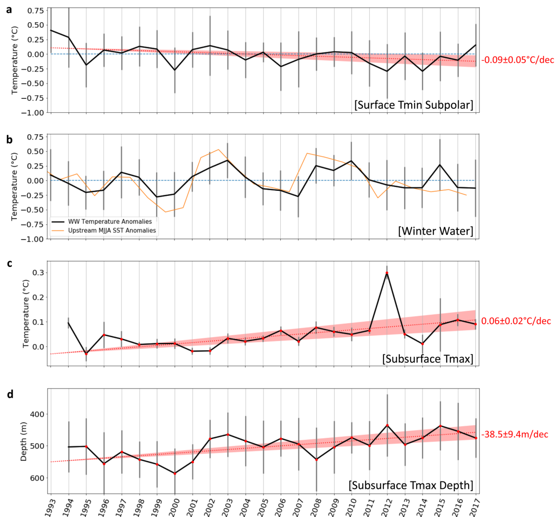
Fig. 4 Time-series of temperature and characteristics of specific water masses. a Zone [B] anomalies, restricted to the gridpoints where the 25 years-mean temperature transect <0 . b Black line is the WW temperature anomalies from SURVOSTRAL XBTs between 54 and 61.5°S, restricted to the Tmin gridpoints where the 25 year-mean temperature transect is less than 2 °C. Yellow line is the MJJA SST anomalies upstream of SURVOSTRAL WW, between (120–145°E and 57–61°S). c CDW maximum temperature evolution (see “Methods”). Red dots are the years the linear trend is computed on; i.e., years when there is at least 2 months with data on average for each grid point for NDJF months. d CDW maximum temperature depth (see “Methods”). Errors bars are the standard deviation of the mean temperature anomalies (depth for panel d ) for each grid point within the zone.
