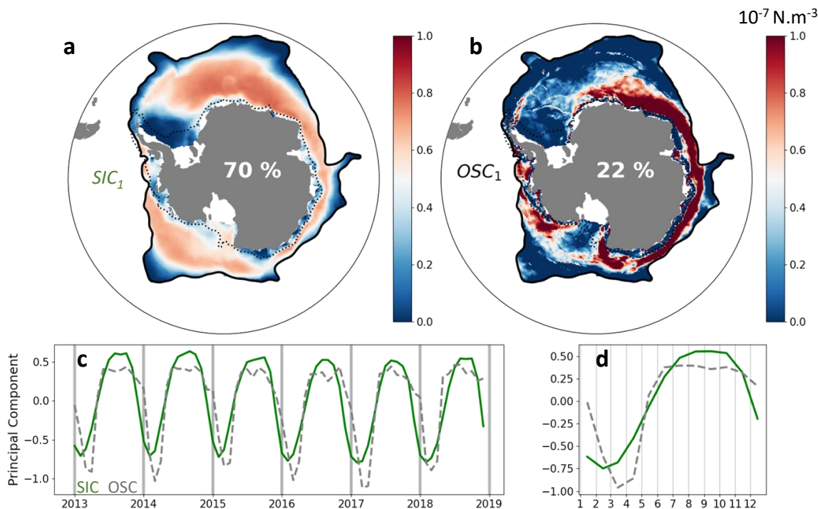
FIGURE III.7: Sea Ice concentration (SIC) and Ocean Stress curl (OSC) first EOF modes. a. SIC EOF mode 1 spatial pattern. Colorbar boundaries are not centered on 0 for a better comparison with Fig. 8. The dotted line is the 1000 m isobath; the black line corresponds to the northern boundary of the subpolar sector as defined in Section 2.2. b. OSC EOF mode 1 spatial pattern. c. In green, SIC mode 1 principal component. In dashed green, OSC mode 1 principal component. d. Seasonal cycles of both principal components.
