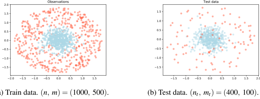
Figure 8.3. Data visualization for the two generating processes. The Gaussian observations are represented in blue. The 'synthetic outliers' samples drawn from the radial law are represented in red. The left figure (a) corresponds to the train dataset, the right (b) to the test dataset.
