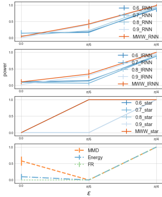
c. (S3), d = 3
