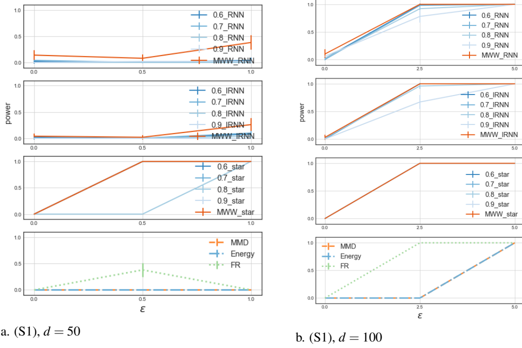
Figure 7.14. Estimation of type-I error and power for the scale model (S1) with n, m = 500, 500 and with d = 50 (a) and d = 100 (b), \pm their standard deviation at 95%. Results for each algorithm are gathered in a same plot, where RTB tests with u_0 \in \{0.6, 0.7, 0.8, 0.9\} are estimated.
