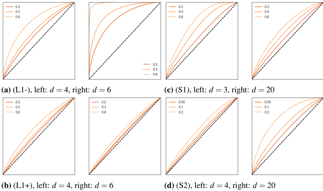
Figure 7.18. True ROC curves (ROC*) for the location and the scale models: (L1+),(L1-),(S1),(S2), depending on the discrepancy parameter \varepsilon \in \{0.2, 0.3, 0.6\} for (L1+) and (L1-), \varepsilon \in \{0.2, 0.4, 0.6\} for (S1) and \varepsilon \in \{0.05, 0.1, 0.2\} for (S2).
