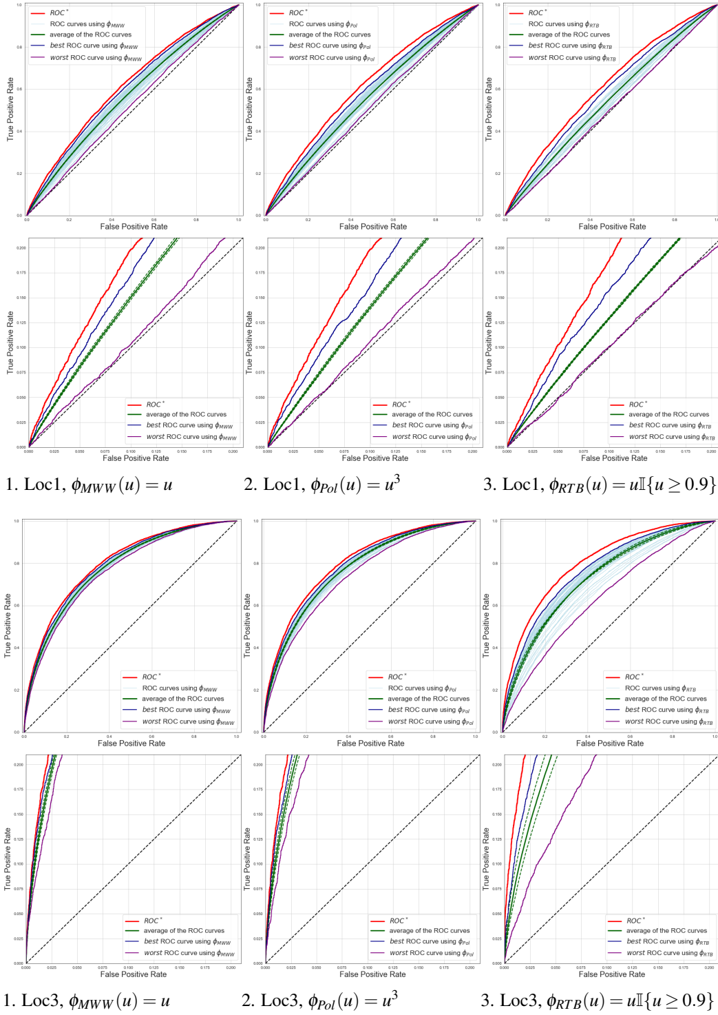
Figure 7.5. Empirical ROC curves and average ROC curve for Loc1 ( \varepsilon = 0.10 ), Loc3 ( \varepsilon = 0.30 ). Samples are drawn from multivariate Gaussian distributions according to section 7.1.2, scored with early-stopped GA algorithm's optimal parameter for the class of scoring functions. Hyperparameters: u_0 = 0.9 , q = 3 , B = 50 , T = 50 . Parameters for the training set: n = m = 150 ; d = 15 ; for the testing set: n = m = 10^6 ; d = 15 . Figures 1,2,3 correspond resp. to the models MMW, Pol, RTB. Light blue curves are the B(= 50) ROC curves that are averaged in green (solid line) with +/- its standard deviation (dashed green lines). The dark blue and purple curves correspond to the best and worst scoring functions over the B Monte Carlo replications. The red curve corresponds to ROC^* .
