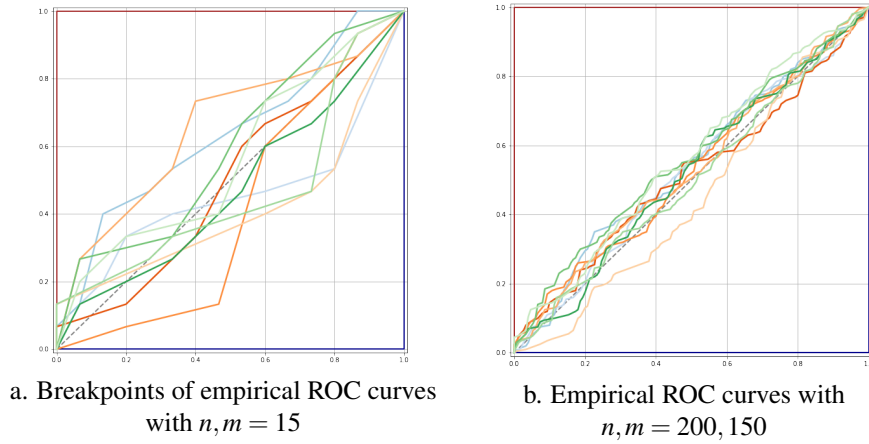
Figure 6.1. Examples of empirical ROC curves simulations under the null hypothesis.
