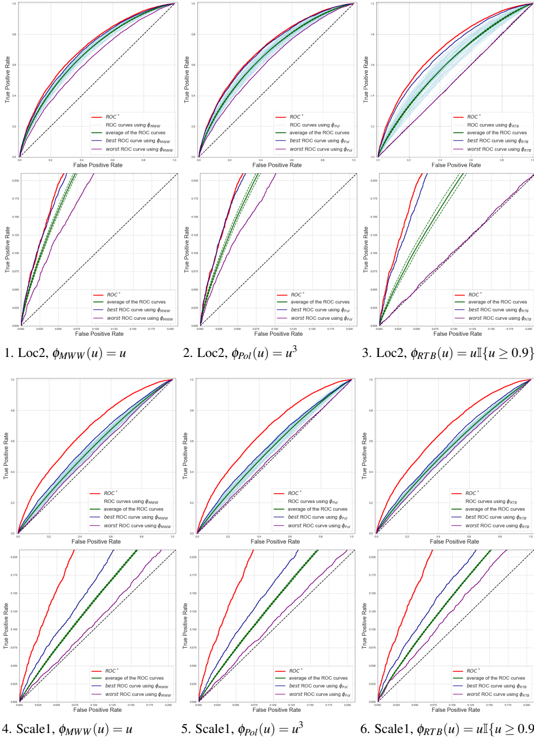
Figure 7.2. Empirical ROC curves and average ROC curve for Loc2 (1-3) ( \epsilon = 0.20 ) and for Scale1 (4-6) ( \epsilon = 0.70 ). Samples are drawn from multivariate Gaussian distributions according to section 7.1.2, scored with early-stopped GA algorithm's optimal parameter for the class of scoring functions. Hyperparameters: u_0 = 0.9 , q = 3 , B = 50 , T = 50 . Parameters for the training set: n = m = 150 ; d = 15 ; for the testing set: n = m = 10^6 ; d = 15 . Figures 1, 2, 3 correspond resp. to the models MMW, Pol, RTB. Light blue curves are the B (= 50) ROC curves that are averaged in green (solid line) with \pm its standard deviation (dashed green lines). The dark blue and purple curves correspond to the best and worst scoring functions in the sense of minimization and maximization of the generalization error among the B curves. The red curve corresponds to ROC^* .
