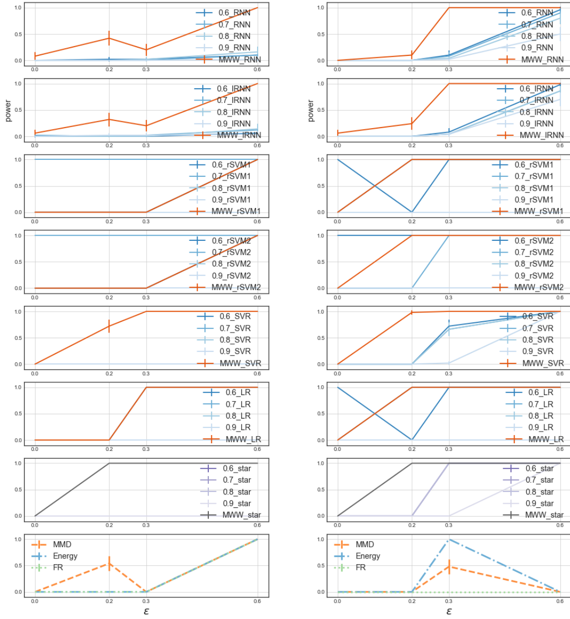
Figure 7.10. Estimation of type-I error and power for the model (L1-) with n, m = 500, 500 , d = 4 (a) and d = 6 (b), \pm their standard deviation at 95%. Results for each algorithm are gathered in a same plot, where RTB tests with u_0 \in \{0.6, 0.7, 0.8, 0.9\} are estimated.
