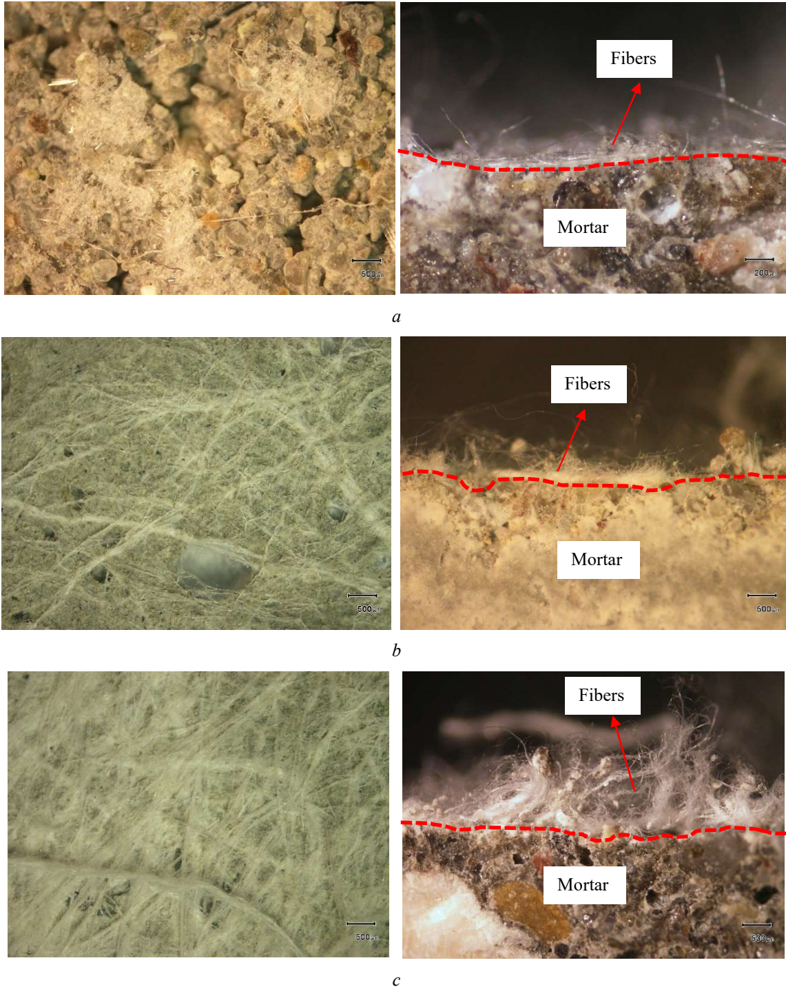
Figure 4- 64: Microscopic analysis of specimens with various w/c ratios; a) w/c=0.40+SP , b) w/c=0.45+SP , and c) w/c=0.50
