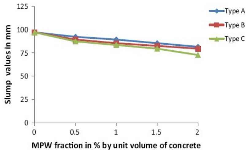
Figure 1- 1: Slump values versus volume fraction of MPW [37]
