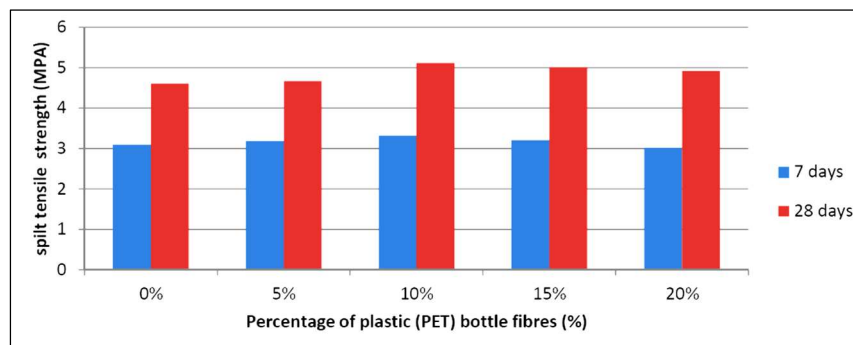
Figure 1- 10: Spilt tensile strength versus percentage of PET plastic fibers [30]
