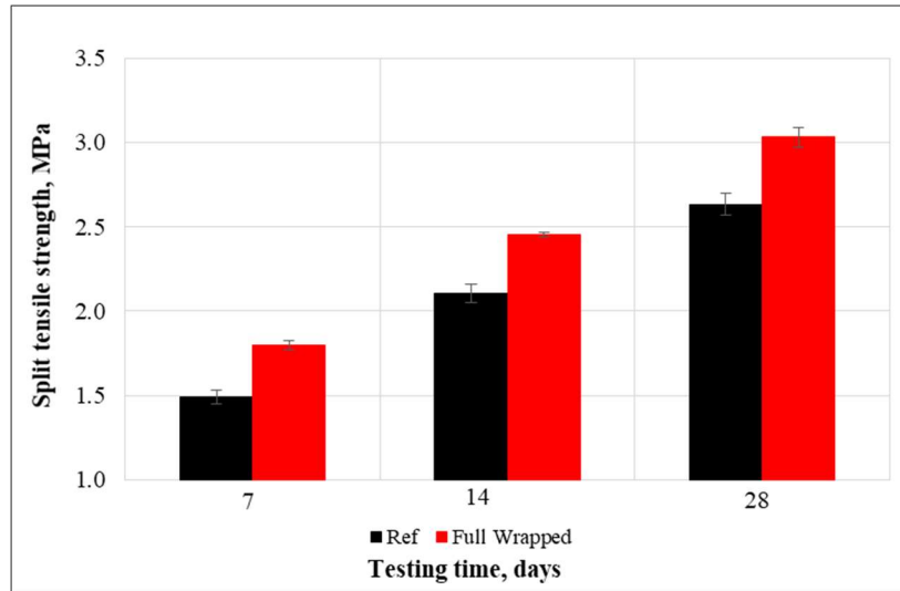
Figure 5- 12: Split tensile strength of concrete specimens
