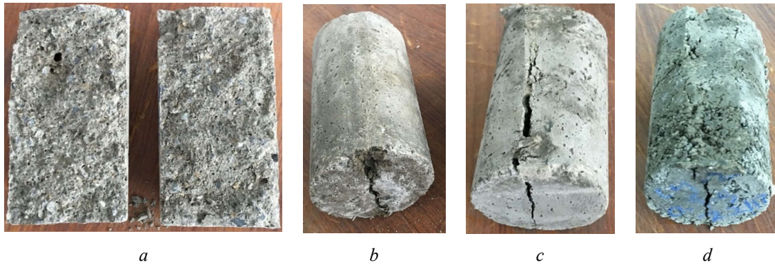
Figure 4- 35: Cracking pattern of mortar cylinders with GHORI cement a) Ref, b) 0.25%, c) 0.50%, and d) 0.75%
