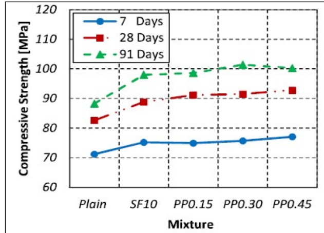
Figure 1- 6: Compressive strength of concrete mixtures with plastic fibers [29]
