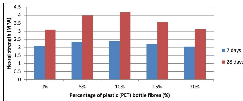
Figure 1- 9: Flexural strength versus percentage of plastic fibres [30]
