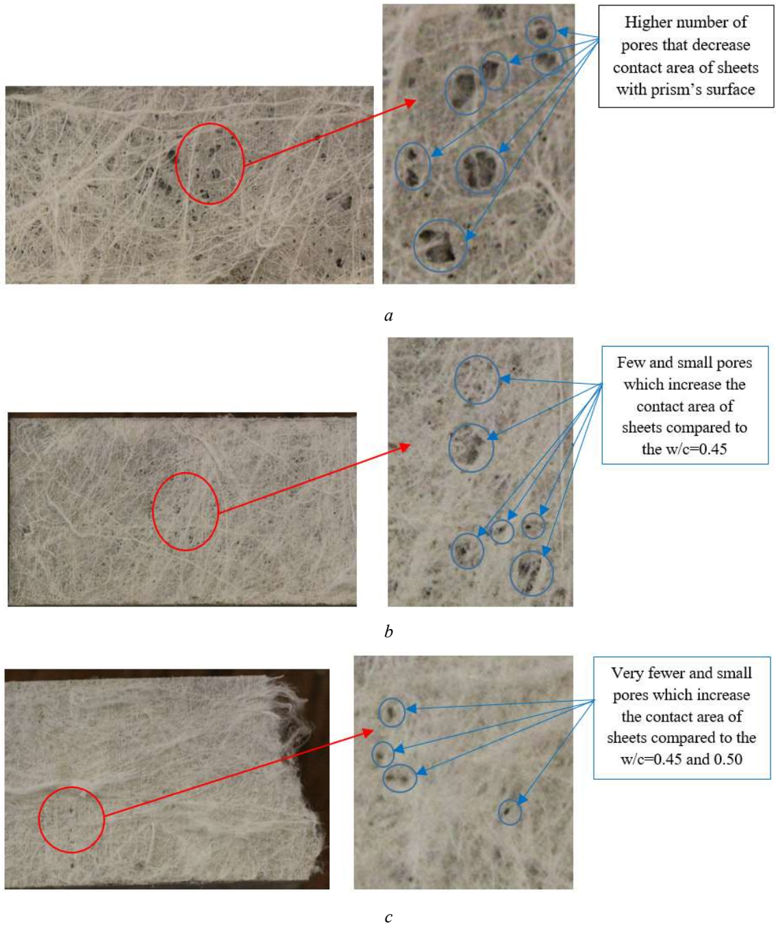
Figure 4- 51: Density of the remaining microfilaments on the surface of specimens with a) w/c=0.45 , b) w/c=0.50 , and c) w/c=0.55
