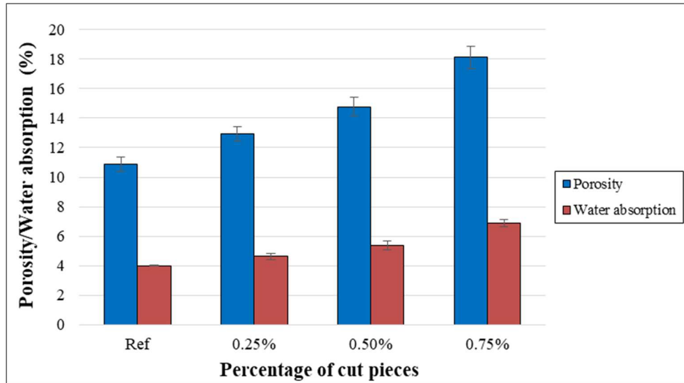
Figure 5- 20: Porosity and water absorption of concrete specimens
