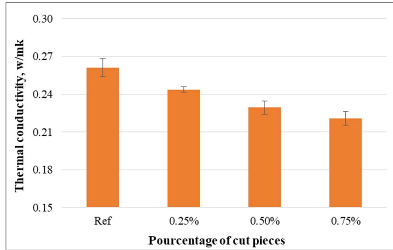
Figure 5- 32: Thermal conductivity of concrete specimens
