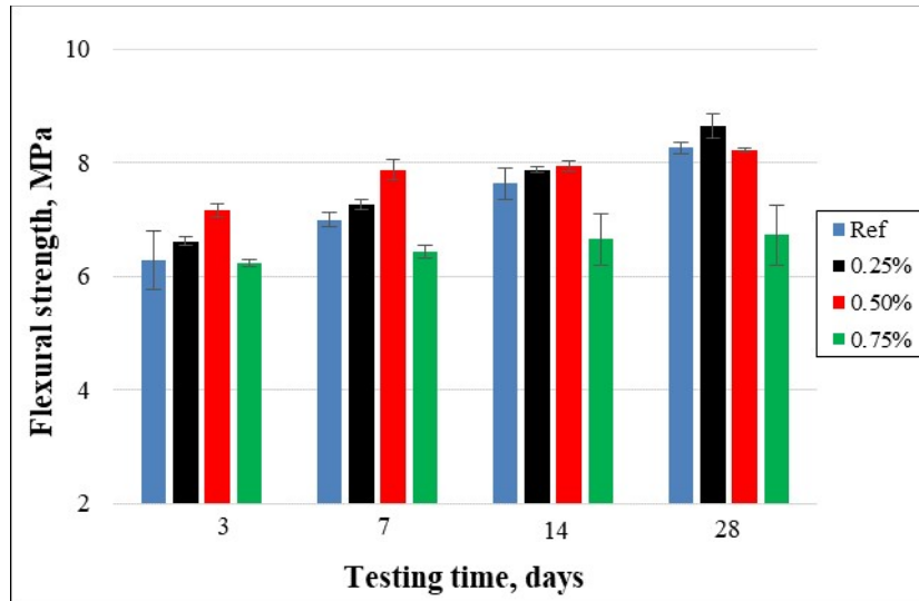
Figure 4- 24: Flexural strength of mortar specimens with CEM I cement
