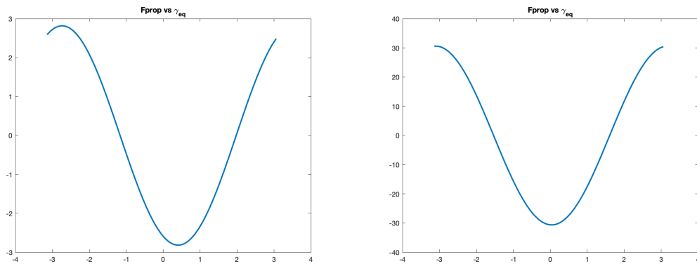
Figure I.3.4: Comparison of F_{prop} for X_M = 3 (left) and X_M = 30 (right). As before, a short tail produces an asymmetry in the propulsion force F_{prop} with respect to the \gamma_{eq} = 0 axis.
