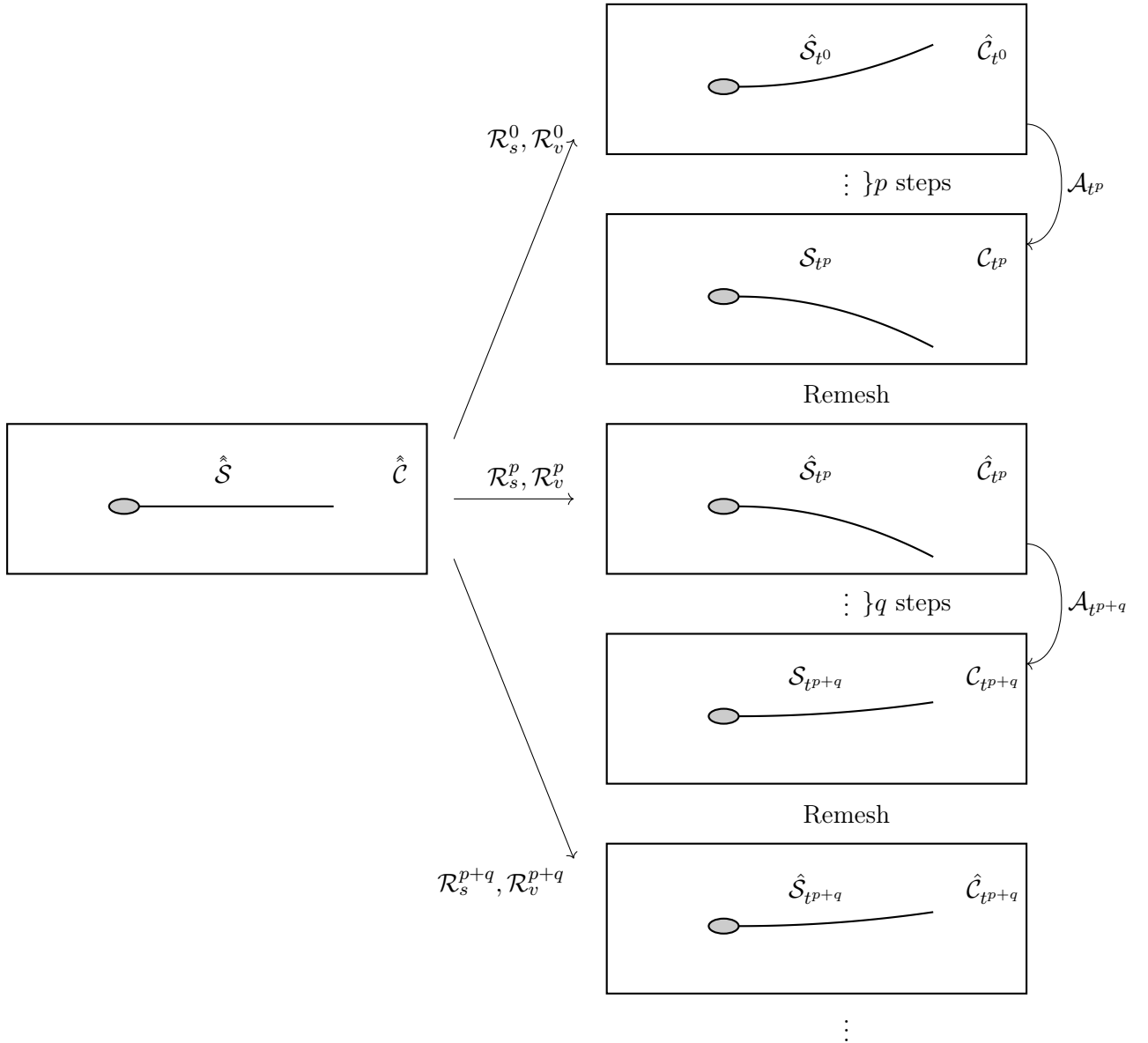
Figure II.2.2: The mesh adaptation procedure alternates remeshing steps with mesh motion. A relationship \mathcal{R}^t between the initial swimmer configuration \hat{S} and the current reference configuration \hat{S}_t allows the evaluation of displacements whose domain coincides with \hat{S} . Between two remeshing steps, the reference configuration of domain \mathcal{S}_{t^{p+1}} is the latest remeshed domain \hat{S}_{t^p} . Depending on the region where the connectivity is preserved, the relationship can be defined on the boundary of the swimmer ( \mathcal{R}_s^t ) or on its volume ( \mathcal{R}_v^t ).
