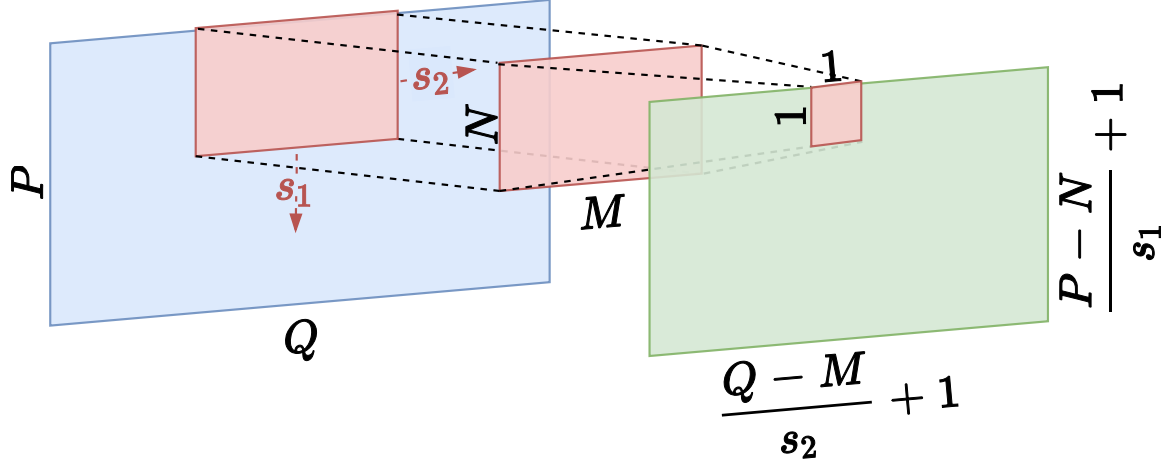
Figure 2.2: Diagram of a convolution mask in two dimensions. The mask (in red) is applied over a matrix (in blue), resulting in the green matrix. Each element of the green matrix is computed by performing the sum of the Hadamard product between the mask and the corresponding window over the blue input matrix. s_1 and s_2 denote the striding factor of the mask in the two dimensions.
