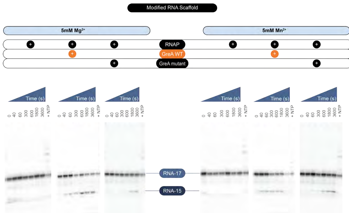
Figure 5.14 – Cleavage Assays comparing Magnesium versus manganese buffers for modified Scaffold U
