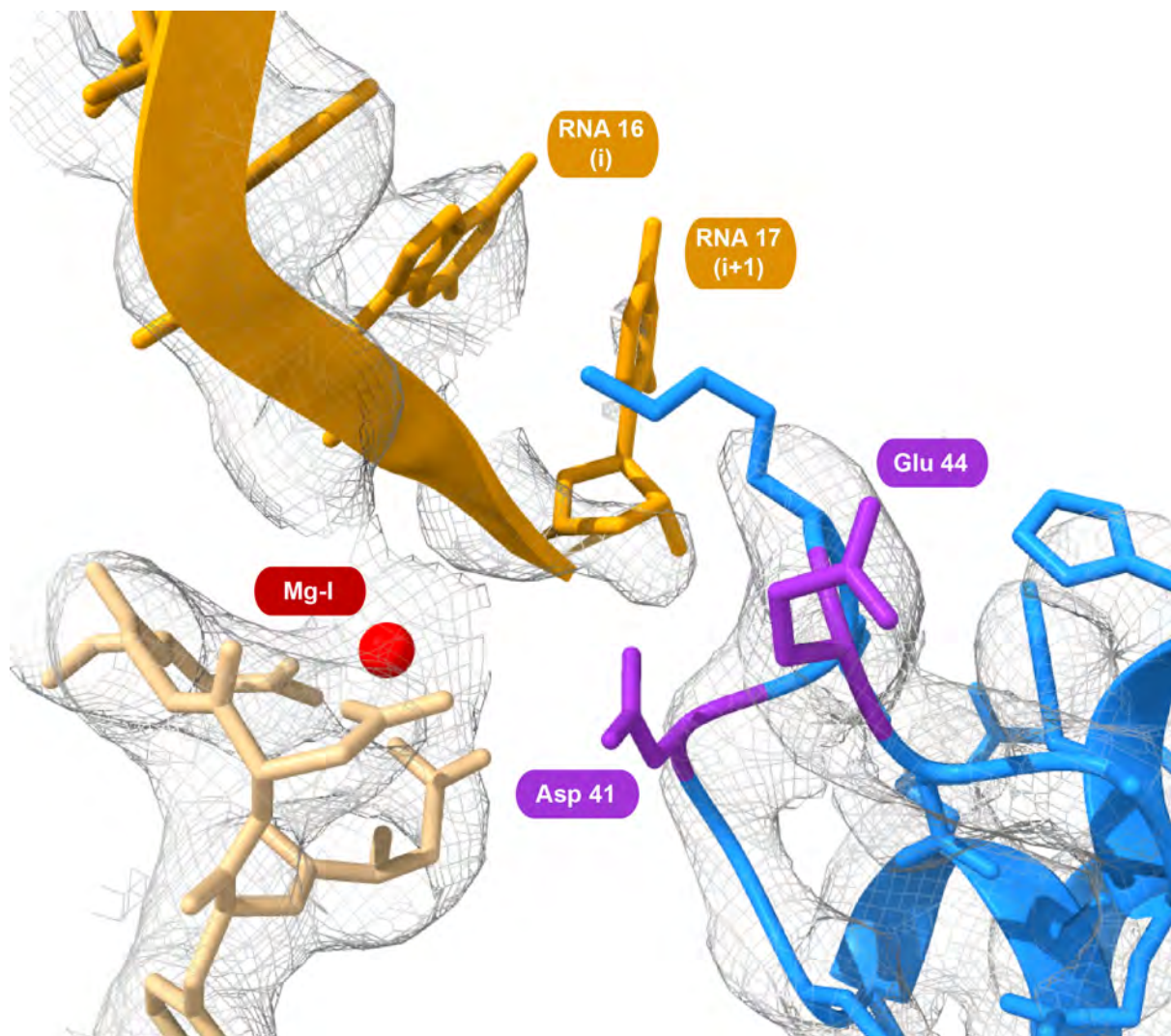
Figure 5.10 – GreA (blue) acidic residues Asp 41 and Glu 44 (highlighted in purple), with Mg-I (red) coordinated by the \beta' aspartate triad (beige).
