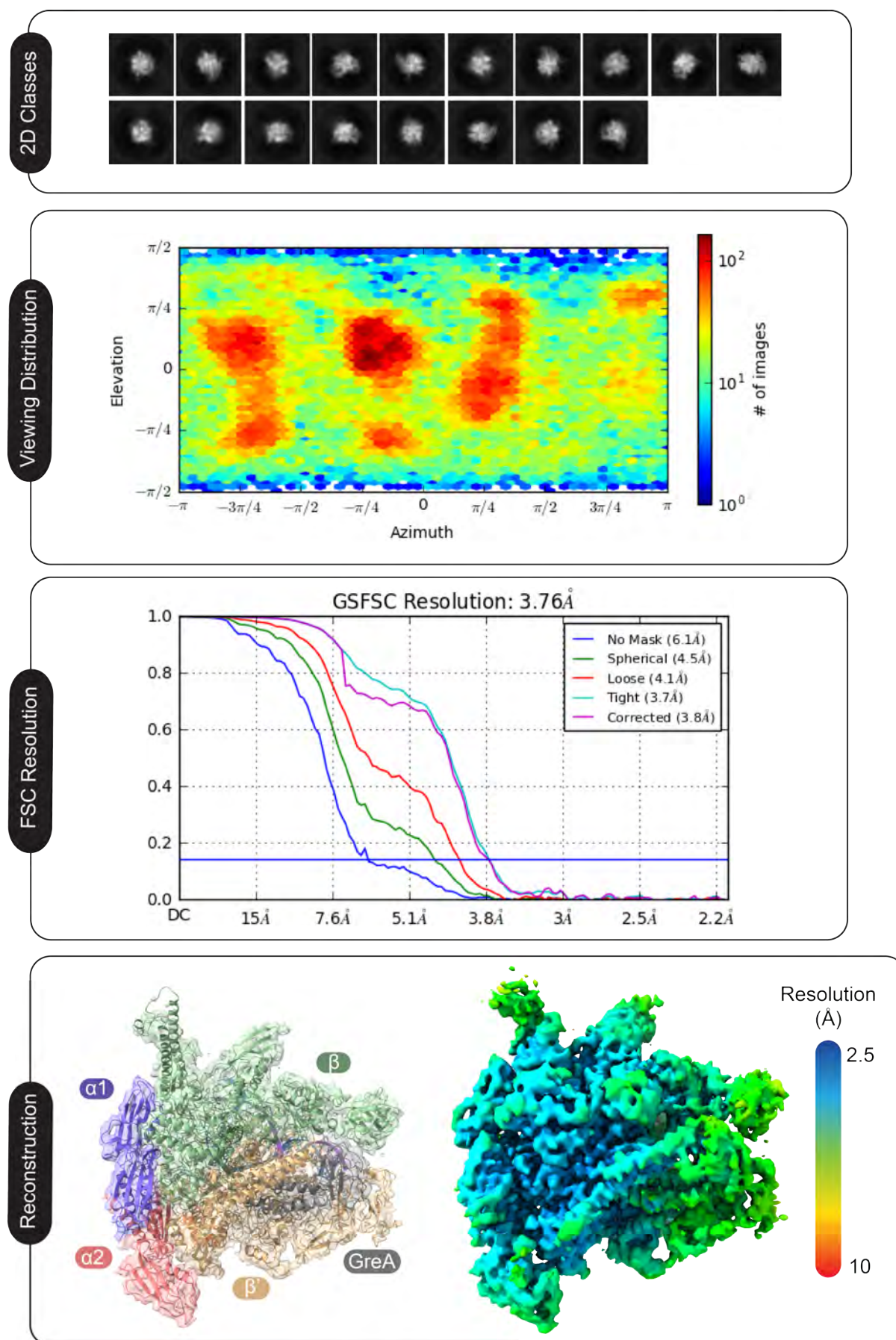
Figure 5.5 – Results of GreA-bound pre-cleavage complex with backtracked base 'A'
