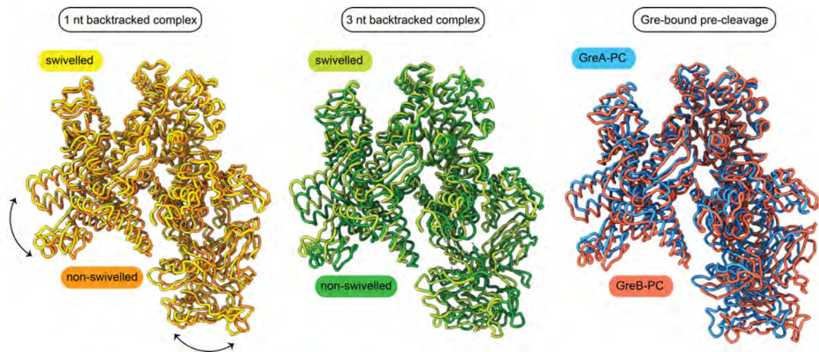
Figure 6.3 – Swivel modules in different complexes aligned to the RNAP core, illustrating that swivelling is seen regardless of the backtracked length, and more importantly that the GreA and GreB backtracked complexes adopt different swivel conformations.
