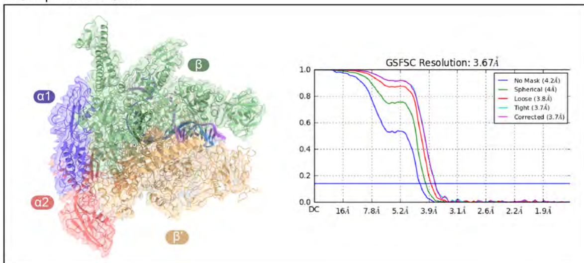
b. Complexe sans GreA
