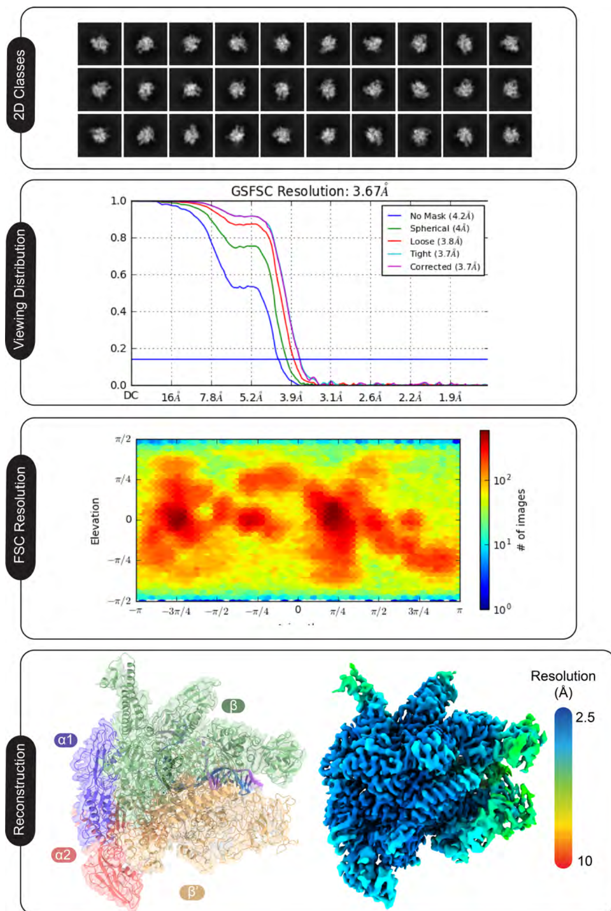
Figure 6.1 – Consensus refinement of the backtracked complex
