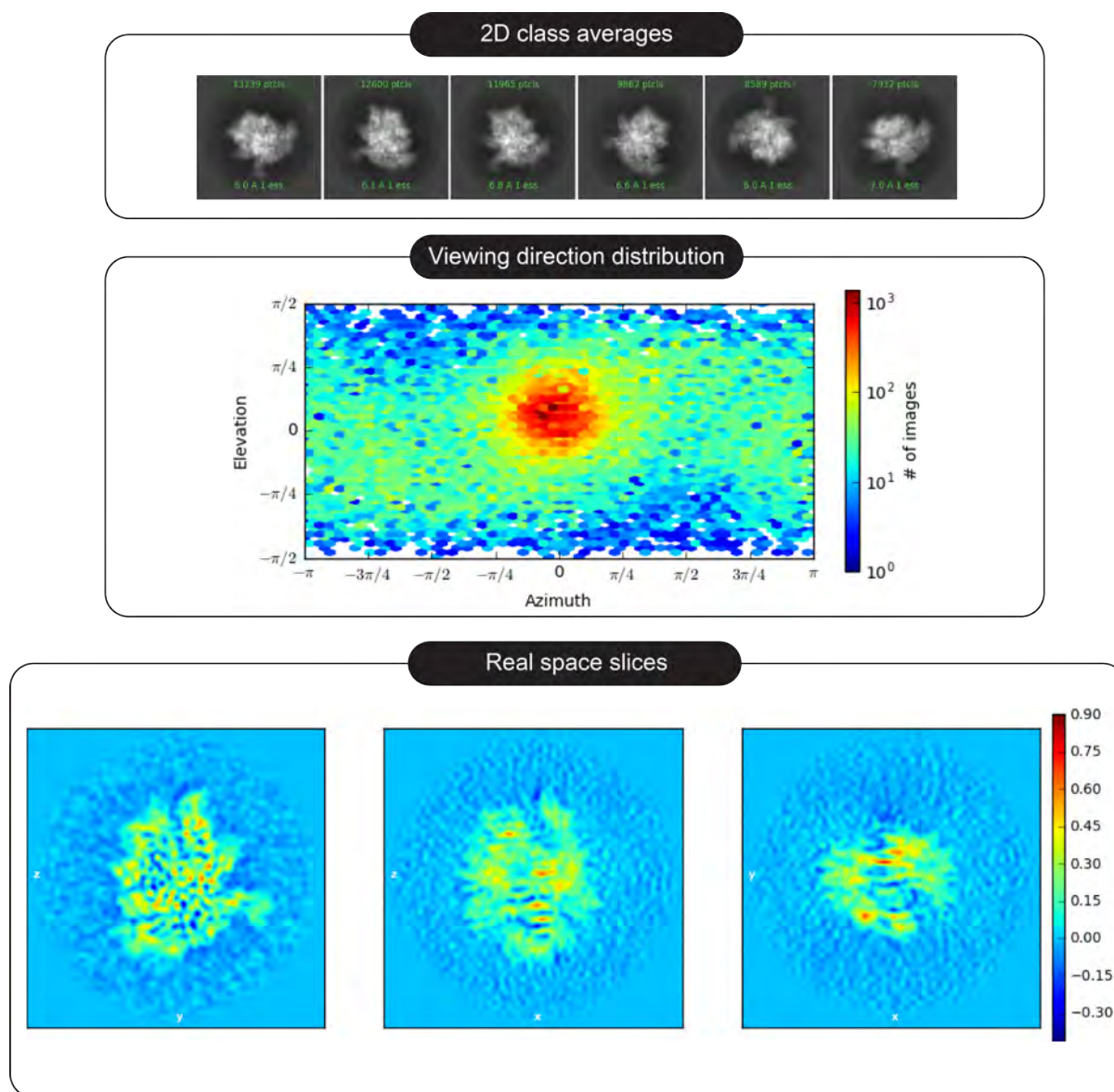
Figure 4.8 – Results for first data collection in September 2018: The 2D class averages after cleanup showed a preference for one orientation of the RNAP complex, which was reflected in the viewing direction distribution plot and real space slices (streaking artefacts) generated from a refinement job containing all of the "clean particles".
