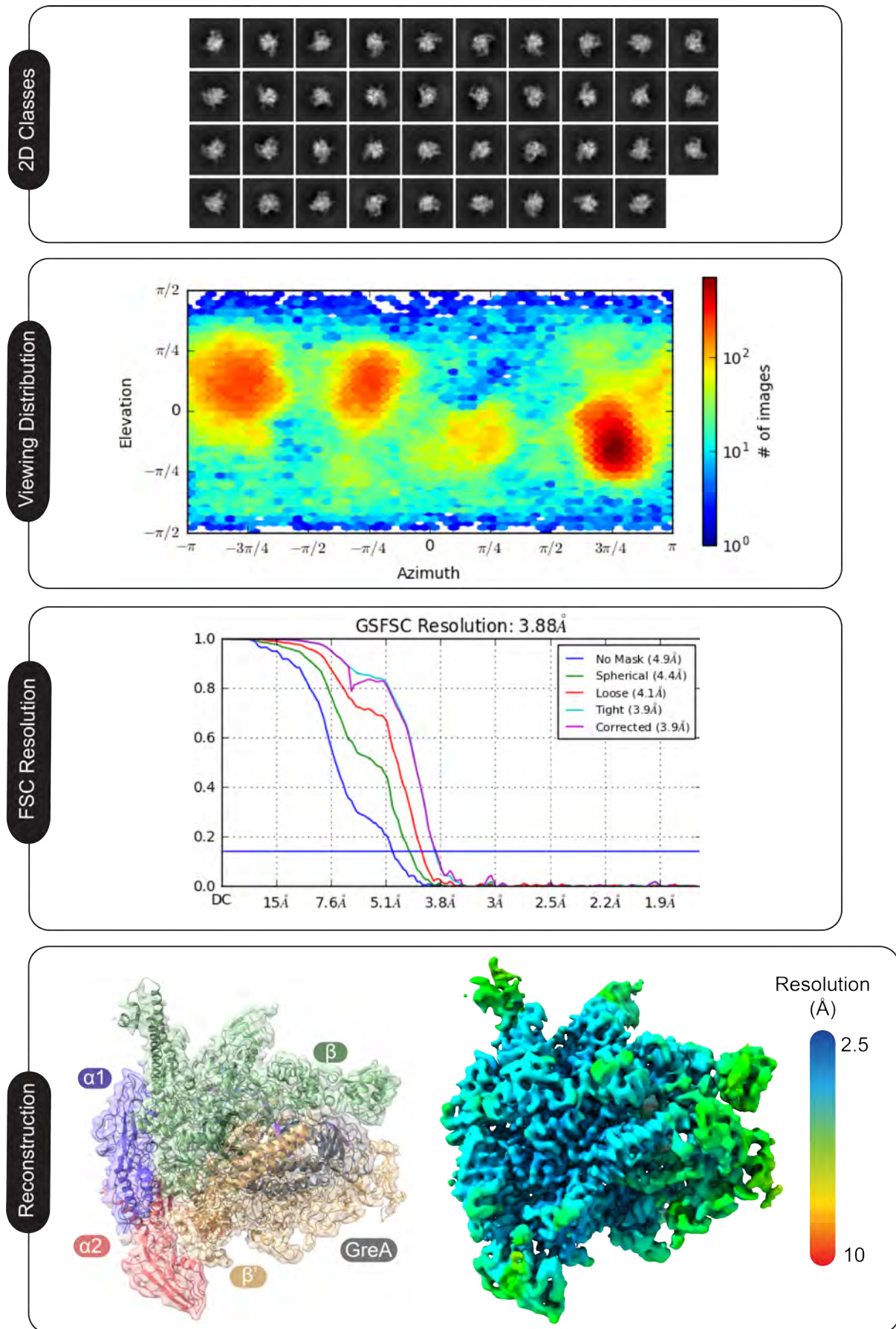
Figure 5.6 – Results of GreA-bound pre-cleavage complex with backtracked base 'G'
