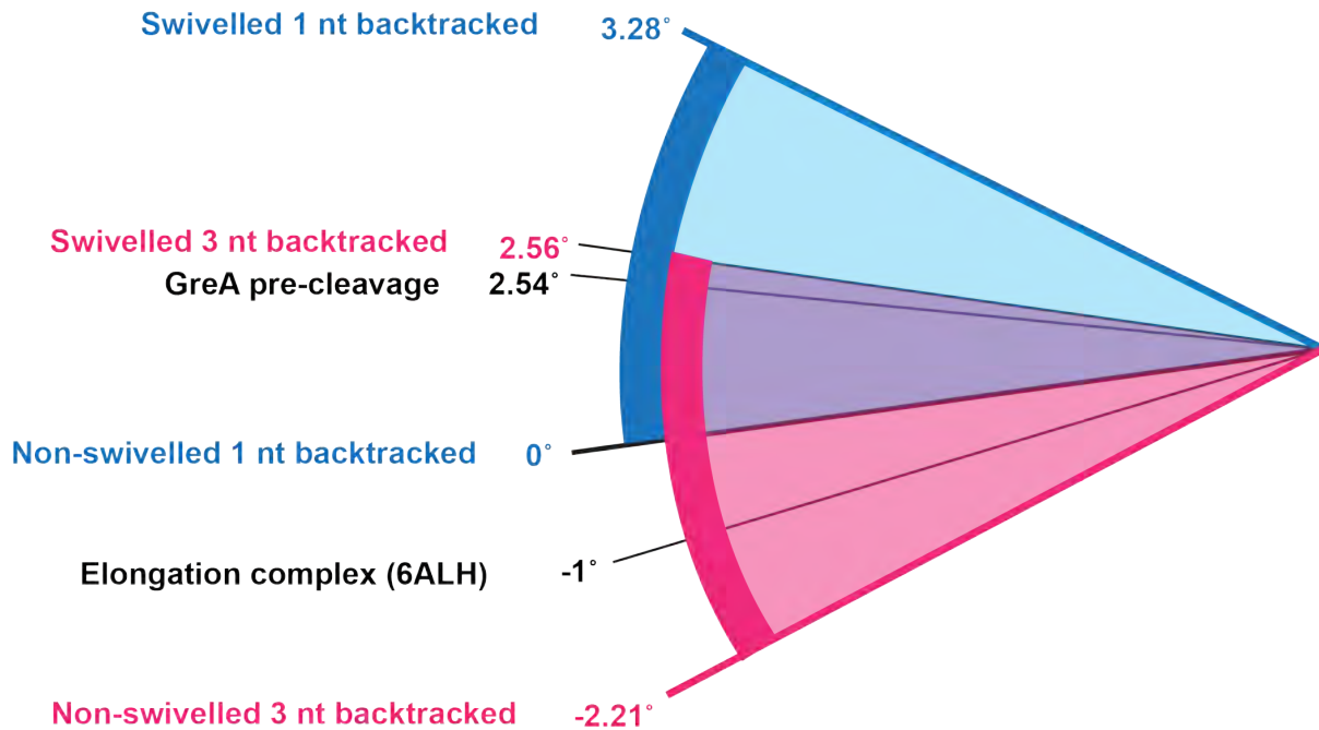
Figure 7.1 – Different rotation angles for swivel modules in different complexes relative to the non-swivelled 1 nucleotide backtracked complex ( 0^\circ ). The swivelling ranges for the 1 and 3 nucleotide backtracked complexes are marked in blue and pink, respectively.
