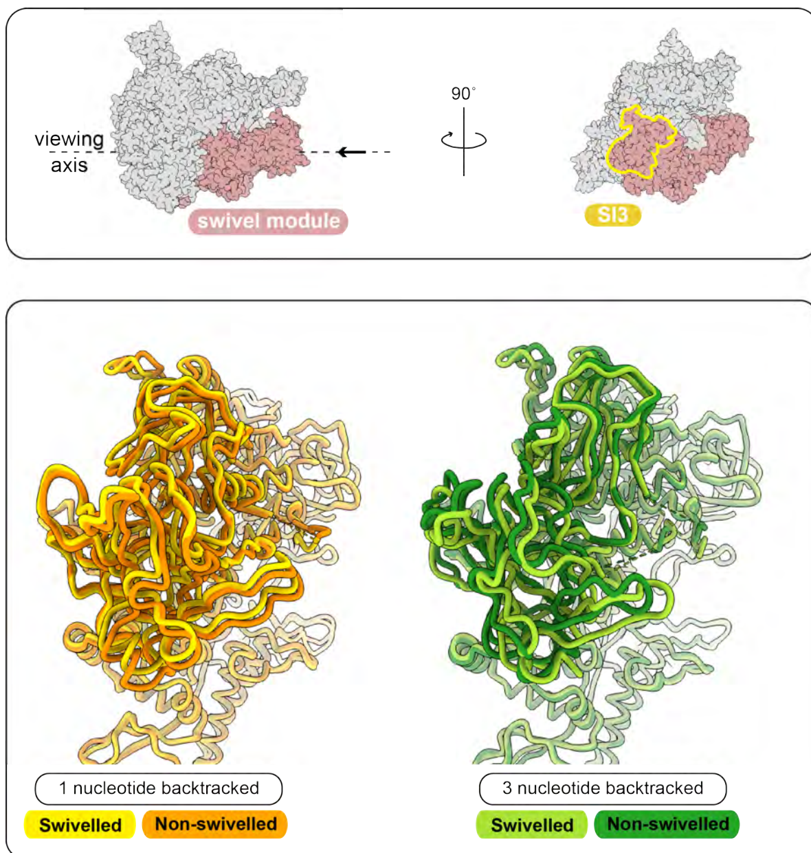
Figure 7.2 – Placement of SI3 domain in different complexes. The SI3 domains for each structure are in the foreground, with the rest of the swivel module in the background. The box on the top shows the viewing direction, which is along the arrow.
