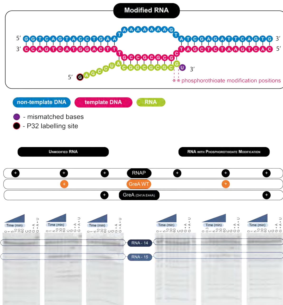
Figure 4.3 – Assays to compare scaffolds with and without RNA modifications
