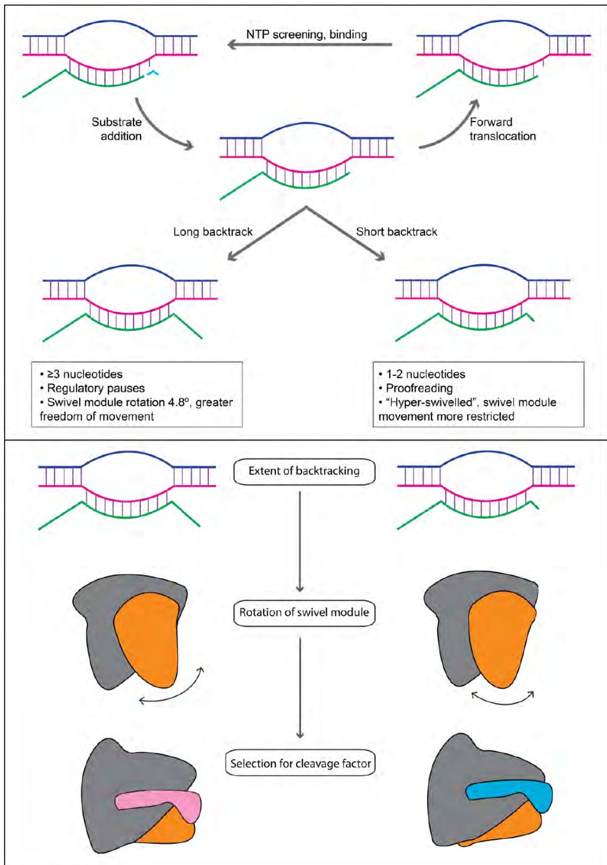
Figure 7.4 – Model for backtrack-dependent factor recruitment. The top half shows the two distinct types of backtracking that can take place during the nucleotide addition cycle (NAC). The bottom half illustrates how the extent of backtracking influences the allowed range of motion of the swivel module (and, by extension, the SI3 domain), which in turn allows for selection of one cleavage factor over another
