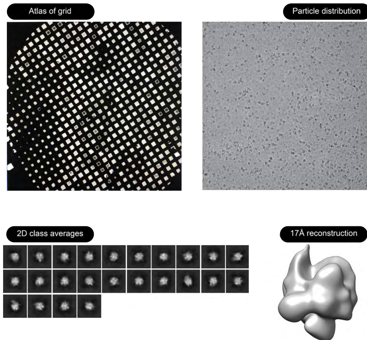
Figure 4.9 – November 2018 Titan data: The image of the EM grid atlas on the top left shows good ice thickness overall, with a representative image of the particle distribution within the grid holes on the top right showing good particle distribution and no contamination. However, analysis of the data yielded a reconstruction with poor resolution which could not be used for structural analysis.
