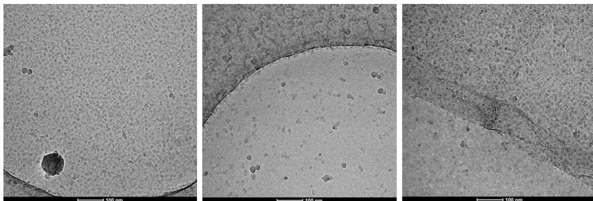
Figure 4.7 – Images of holes within graphene oxide-coated grids. The images on the left shows a hole covered with GO, with a sample concentration of 1 mg/ml RNAP. The hole in the centre is from the same grid, but without GO and hence no particles. The image on the right is from a partially covered hole on a different grid with a sample concentration of 0.1 mg/ml.
