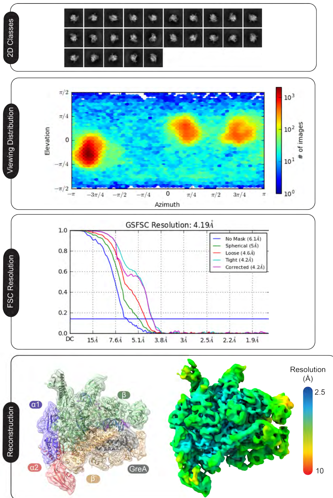
Figure 5.7 – Results of GreA-bound pre-cleavage complex with backtracked base 'C'
