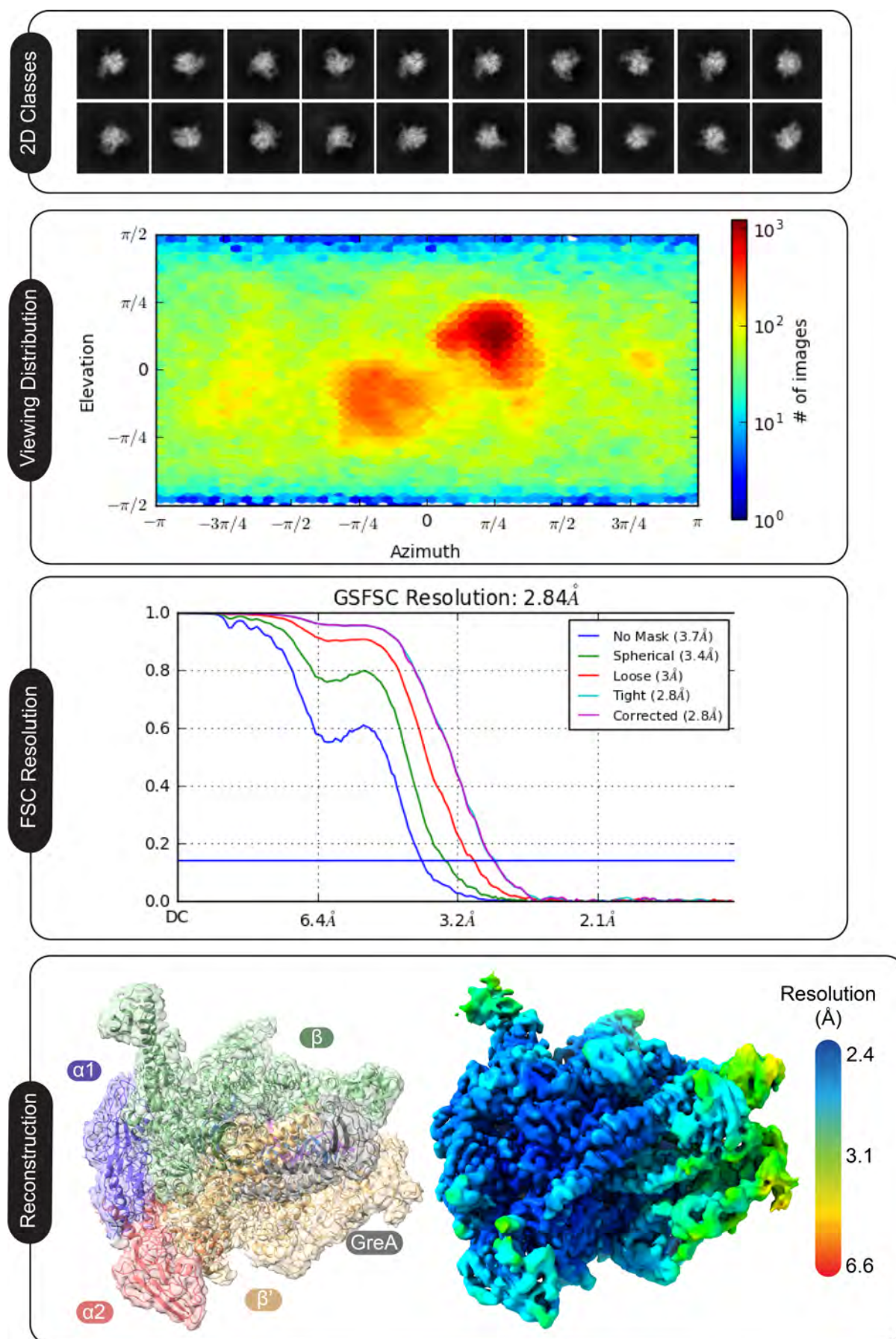
Figure 5.4 – Results of GreA-bound pre-cleavage complex with backtracked base 'U'
