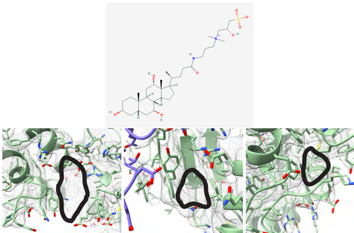
Figure 5.12 – (Top) 2D structure of Chapso molecule 1 ; (Bottom) Chapso binding positions marked in black in the 2.8 Å GreA pre-cleavage map, corresponding to three positions defined in (Chen et al. 2019)
