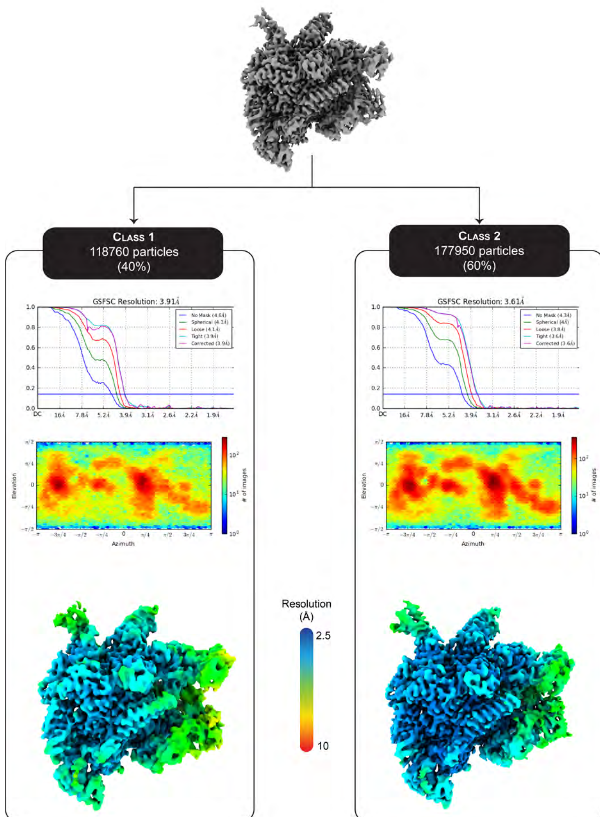
Figure 6.2 – Classification of the backtracked complex
