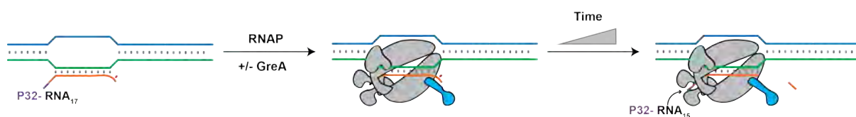
Figure 3.2 – Experimental schematic of the in vitro cleavage assays
