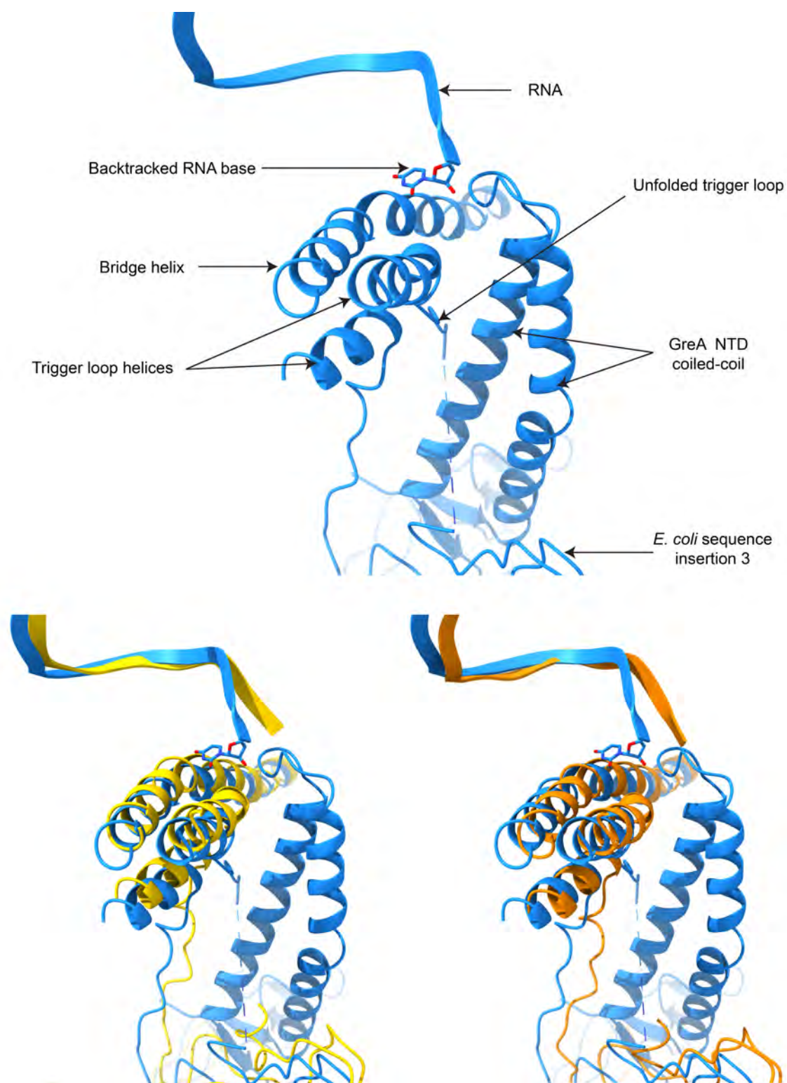
Figure 6.6 – Positions of different active site elements relative to another in the structures with and without GreA. The elements for the GreA pre-cleavage complex are shown in blue, with individual comparisons with the swivelled (yellow) and non-swivelled (orange) backtracked complexes at the bottom.
