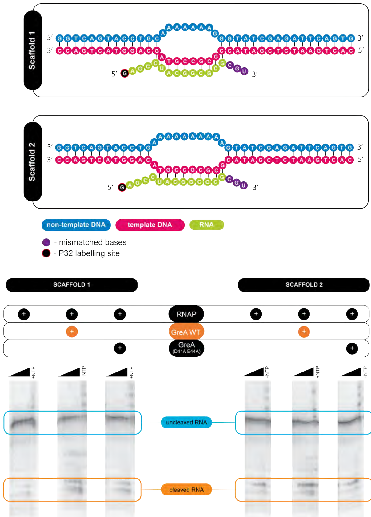
Figure 4.1 – Results of the first set of transcription assays, which were used to assess the functionality of the assembled complex as well as to start testing out scaffolds that would yield a single homogeneous product. The time course used in these was 0/1'/5'/10'/30', followed by a chase of NTP (A+C+G+U).
