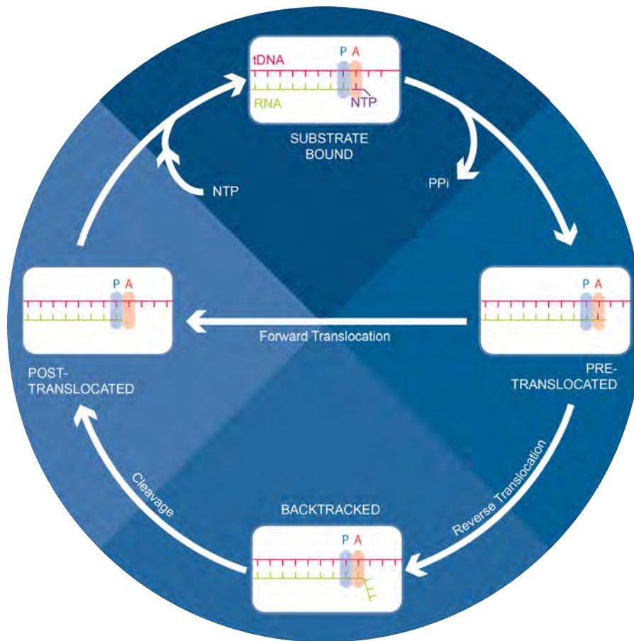
Figure 1.9 – Nucleotide addition cycle during transcription elongation, showing the A- and P-sites
