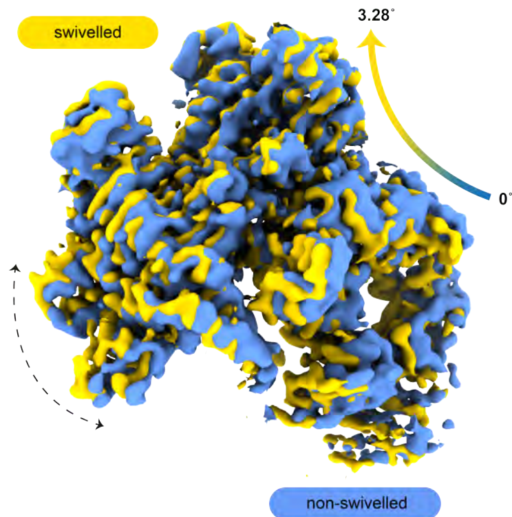
Figure 6.4 – Rotation of the swivel module of the 1 nt backtracked complex
