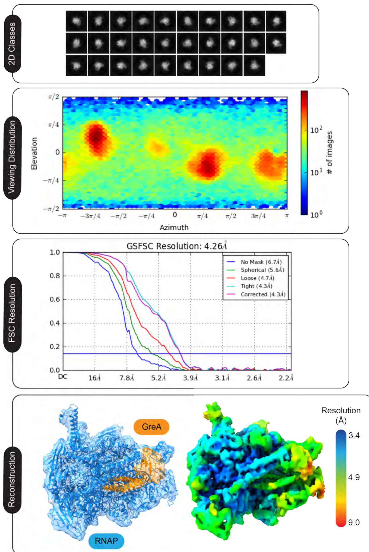
Figure 4.10 – Preliminary reconstruction of the GreA-bound pre-cleavage complex
