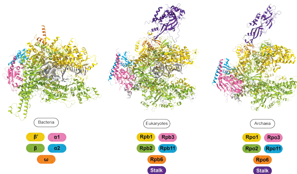
Figure 1.7 – Comparison of RNAP structures of species from all three kingdoms of life, with equivalent subunits coloured similarly. The structures are all oriented with the downstream DNA entering from the right hand side of the page, and the upstream DNA directed outwards from the face of the page. The bacterial structure is from E. coli (6ALH) (Kang et al. 2017), Pol-II from Saccharomyces cerevisiae (1Y1W) (Kettenberger, Armache, and Cramer 2004), and archaeal RNAP from Saccharolobus shibatae (2WAQ) (Korkhin et al. 2009). The archaeal and eukaryotic structures show the stalk (coloured in purple), which isn't present in bacteria
