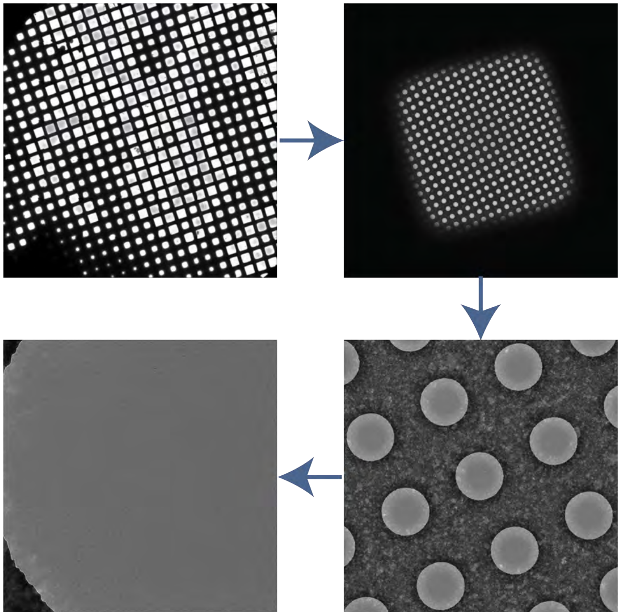
Figure 5.3 – Figures of the grid used for collection of the data shown in Figure 5.4. Clockwise starting from the top left: grid atlas, square map, shot over a hole, and an example of the particle distribution within a hole
