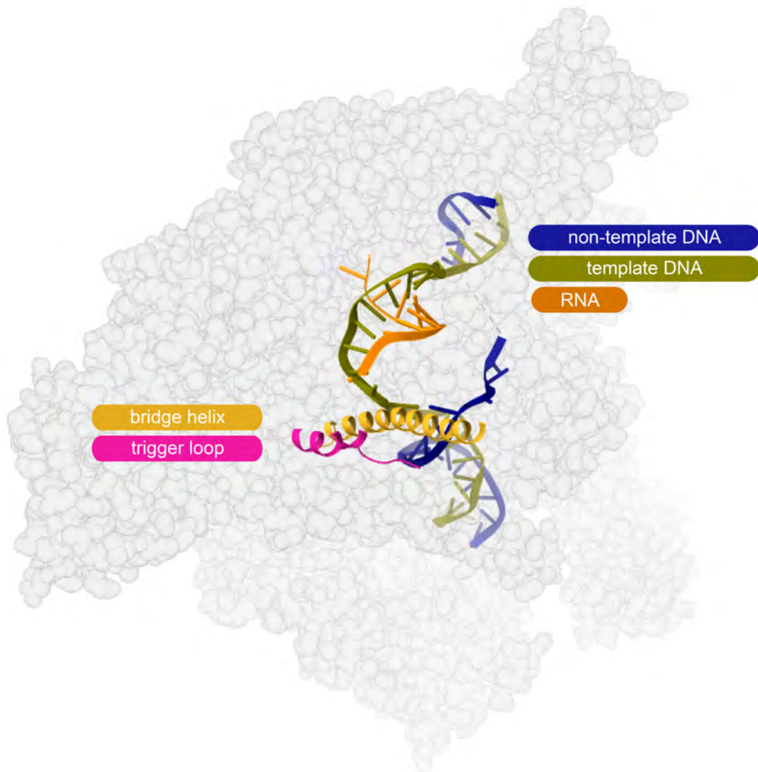
Figure 1.5 – Positions of the bridge helix and trigger loop within the RNAP active site, with respect to the RNA transcript, template and non-template DNA strands.
