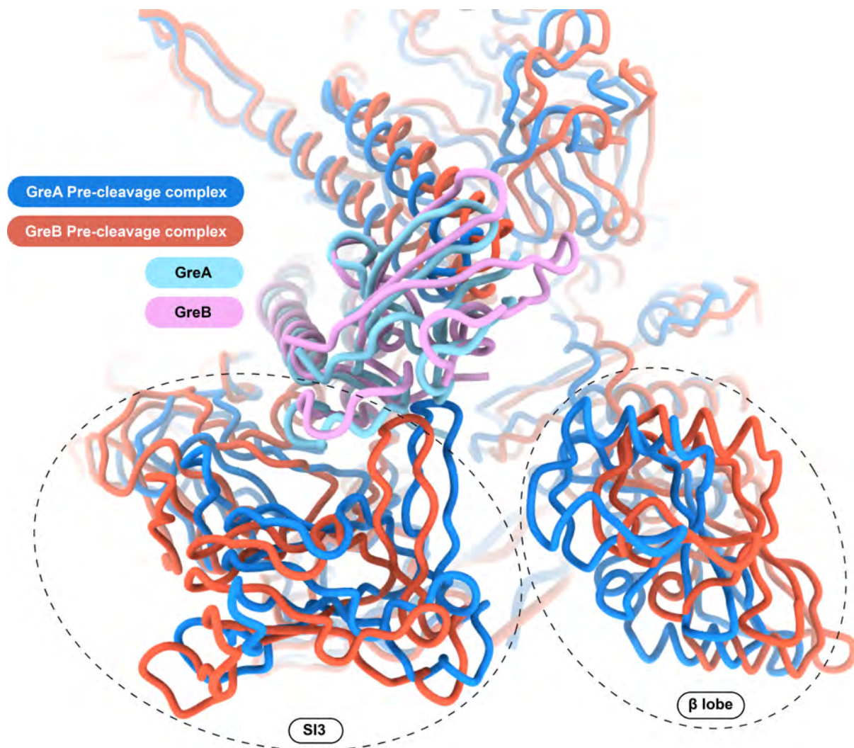
Figure 6.5 – SI3 domain placement in GreA and GreB-bound complexes, aligned by the swivel module excluding the SI3. The SI3 and \beta -lobe, which form the ends of the pincers in the RNAP crab claw, are circled.
