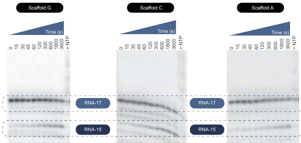
Figure 5.2 – Transcription assays to assess the functionality and GreA-assisted cleavage of remaining 1 nt backtracked complexes
