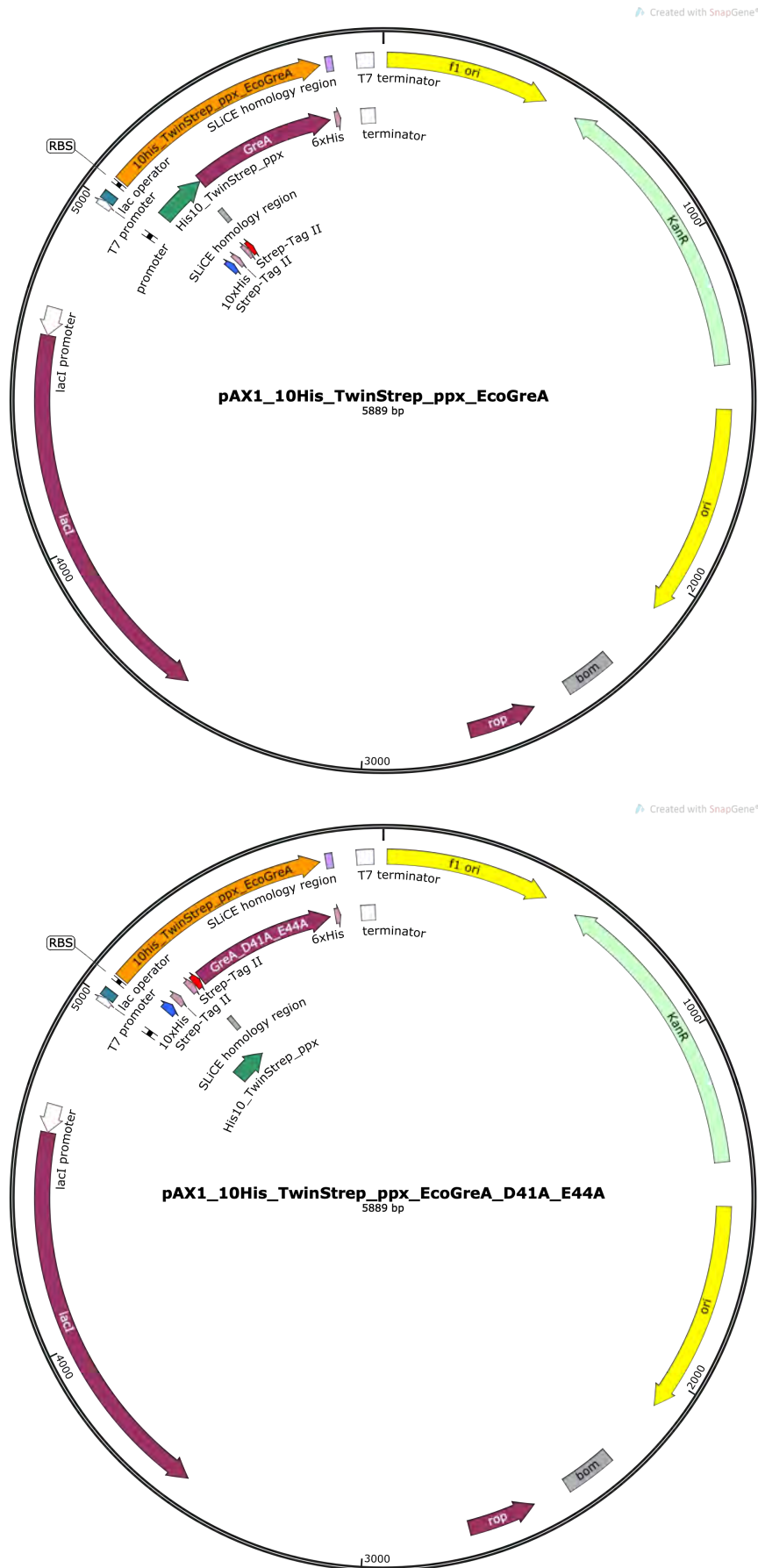
Figure 3.1 – Plasmid maps for GreA wild type (top) and mutant (bottom) expression vectors
