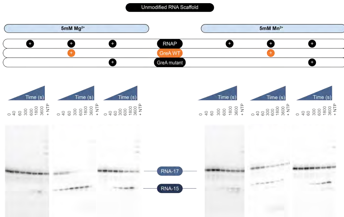
Figure 5.13 – Cleavage Assays comparing Magnesium versus manganese buffers for unmodified Scaffold U
