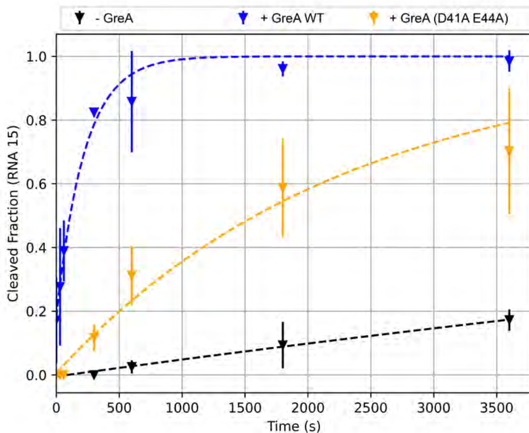
Figure 4.4 – Graph of cleavage fraction versus time for different conditions: RNAP alone, RNAP + WT GreA, and RNAP + mutant GreA. The half life for each fitted curve are (top to bottom) 2.6, 26.6, and 212.8 minutes.
