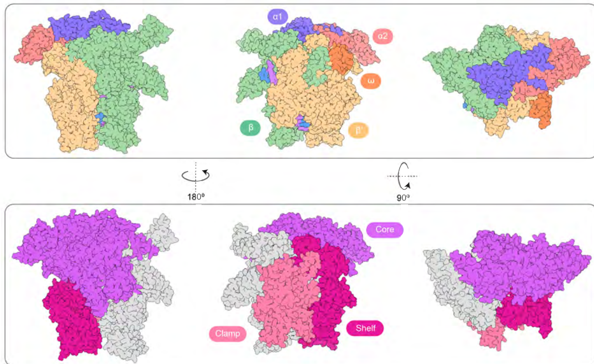
Figure 1.6 – E. coli RNAP subunits and relevant domains
