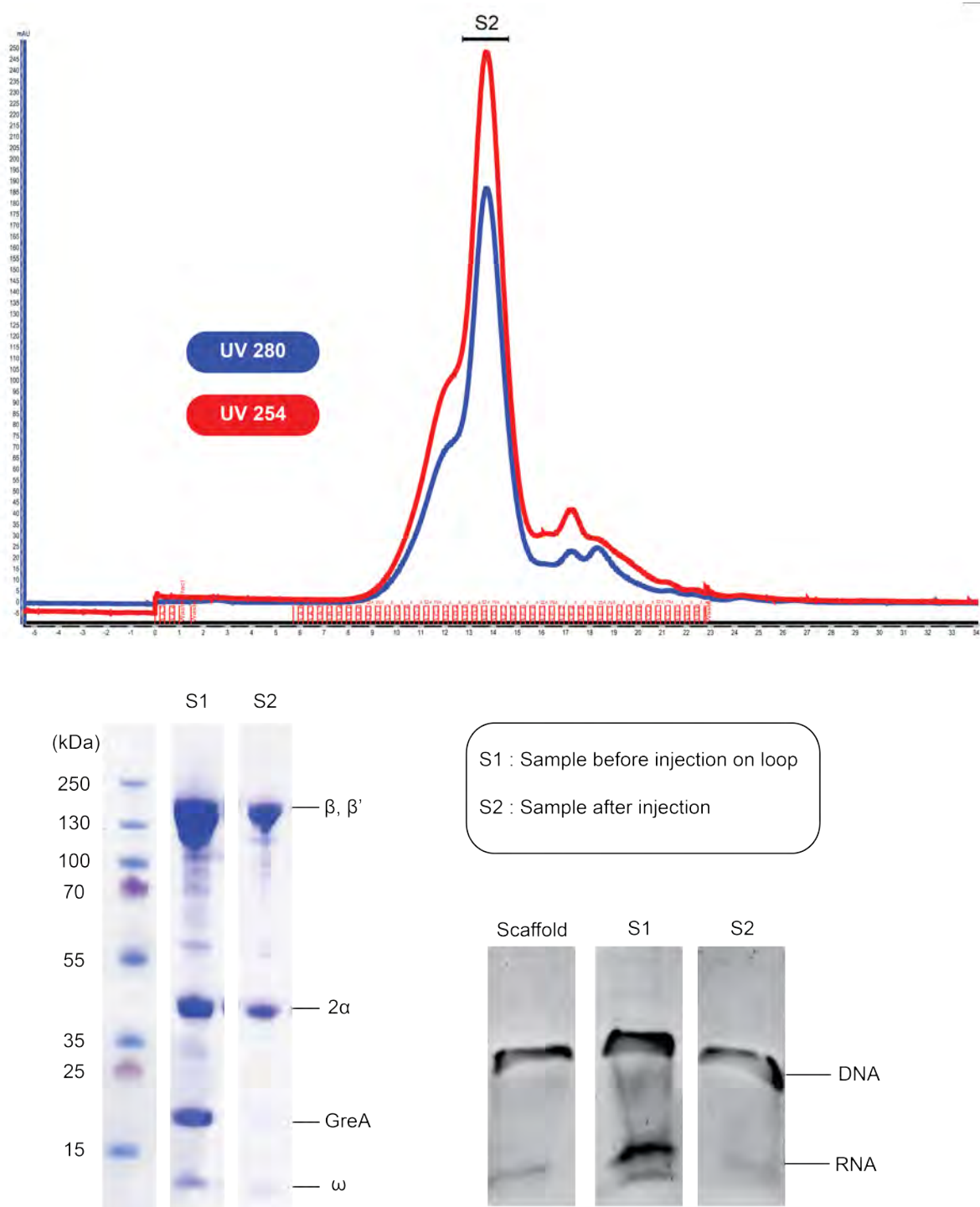
Figure 4.6 – Top : Size exclusion chromatogram of the entire assembled complex (x-axis = mAU, y-axis = collection fractions). Bottom left : SDS-PAGE columns of the protein ladder, the injected sample and the sample contained in the central peak on the chromatogram. Bottom right : Urea gel showing nucleic acid components within the injected sample and the chromatogram main peak, with the complex scaffold used as a reference.
