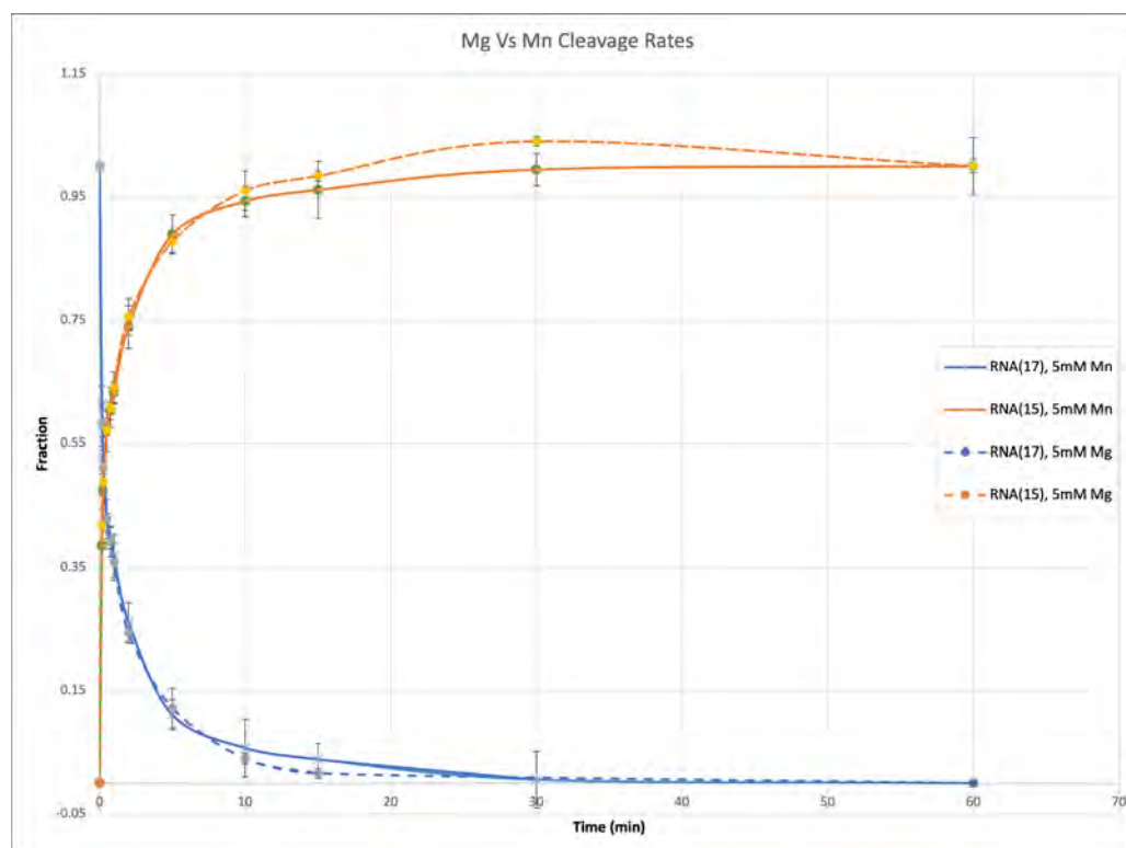
Figure 5.15 – Comparison of cleavage of modified RNA in manganese and magnesium buffers in the presence of WT GreA. The blue lines correspond to the fraction of the uncleaved RNA, with orange corresponding to the cleaved product.
