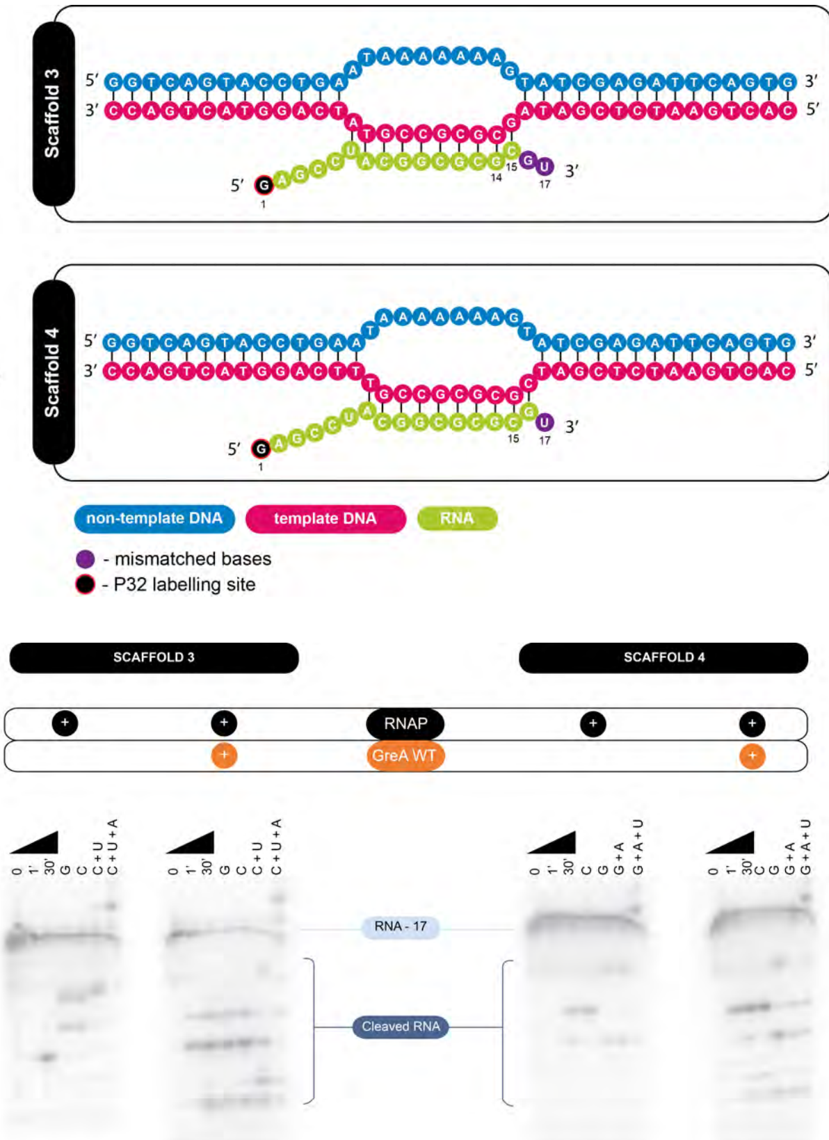
Figure 4.2 – Assays to test homogeneity of tri- versus di-nucleotide cleavage, with RNA positions 1, 15, and 17 labelled in the scaffold diagrams. Uncleaved RNA is 17 nt-long.
