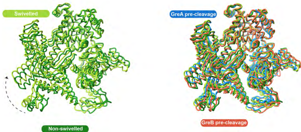
Figure 5.8 – Comparison of swivelling in GreA versus GreB pre-cleavage complexes. Only the swivel modules are shown, and models were aligned to the enzyme core. The two swivelled conformations in the 3 nt backtracked complex (PDB 6RI9 and 6RIP) are shown on the left, with the two Gre-bound pre-cleavage structures on the right (GreB pre-cleavage complex PDB 6RIN)
