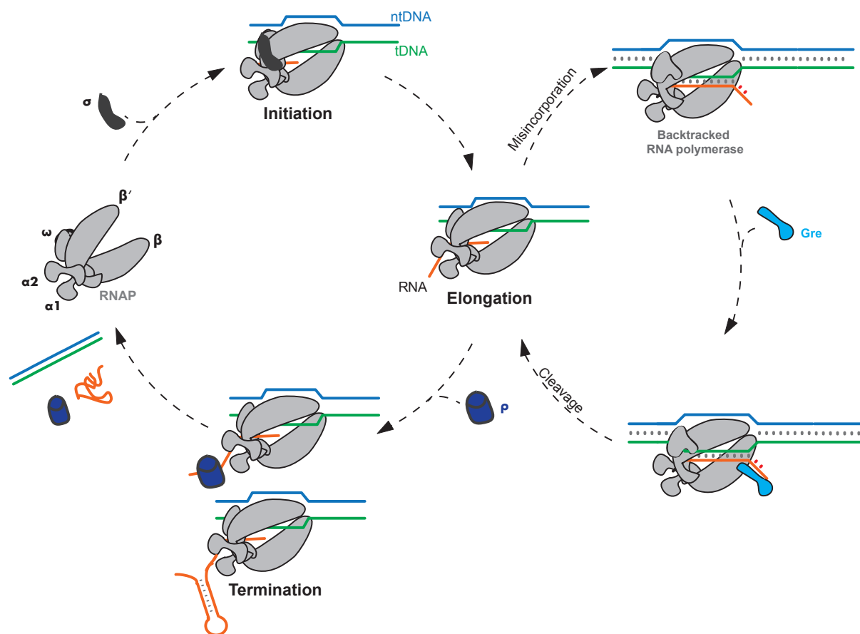
Figure 1.8 – Schematic of the transcription cycle in E. coli , showing the three main phases - initiation, elongation, and termination
