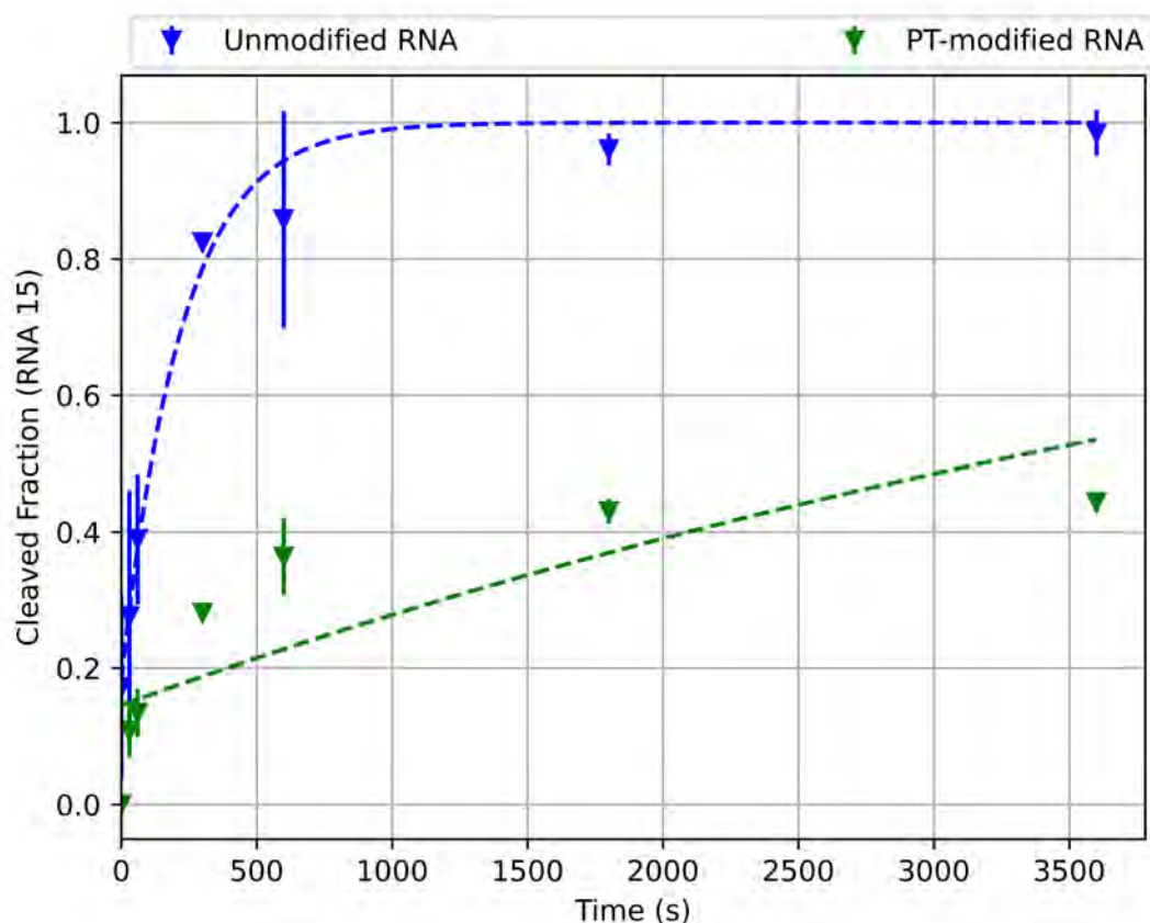
Figure 4.5 – Graph comparing the di-nucleotide cleavage of 1 nucleotide backtracked RNA with and without phosphorothioate modifications in the presence of GreA
