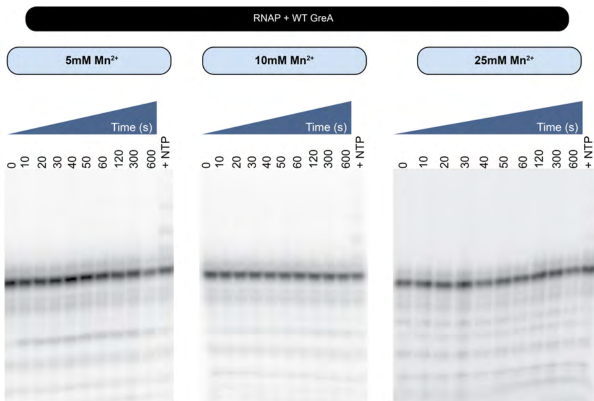
Figure 5.16 – Comparison of different concentrations of manganese on GreA-assisted cleavage of modified RNA
