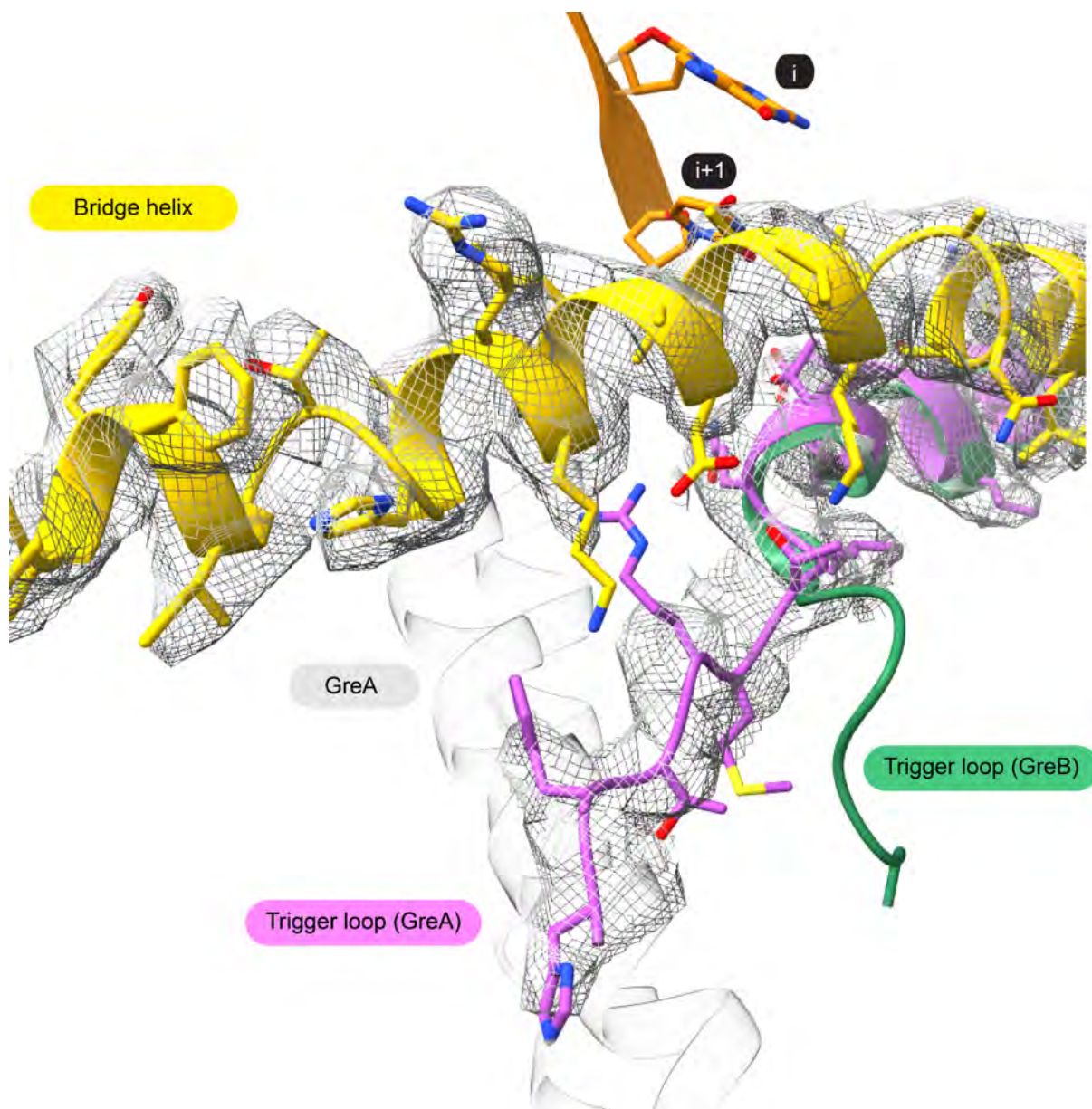
Figure 5.11 – Trigger loop open conformation in GreA pre-cleavage structure
