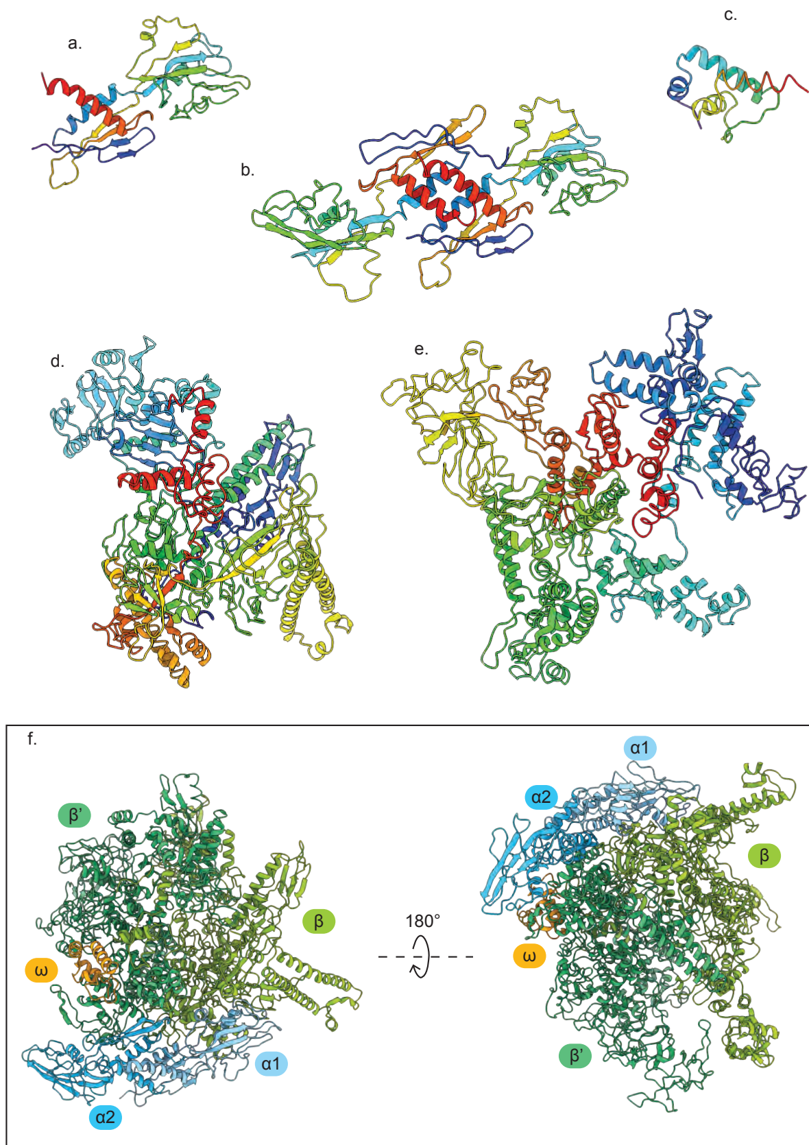
Figure 1.4 – Subunit composition of E. coli RNAP, showing (a) a single \alpha subunit and (b) the \alpha subunit dimer, (c) \omega , (d) \beta , and (e) \beta'
