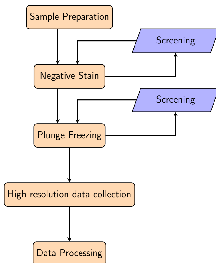
Figure 3.3 – Cryo-EM workflow
