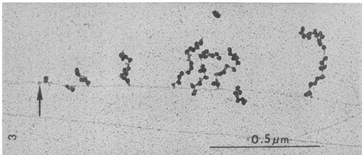
Figure 1.1 – Electron micrograph of an E. coli gene being transcribed by RNA polymerases (marked by arrow), with the transcripts appearing as branches along the DNA—the longer transcripts being further away from the transcription start sites. The darker spots are ribosomes bound to the nascent RNA. (Miller, Hamkalo, and Thomas 1970)
