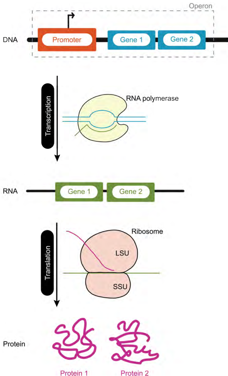
Figure 1.2 – Gene expression in bacteria: starting at a DNA promoter, transcription of one strand takes place to produce an RNA containing the same sequence of the transcribed DNA. This is followed by translation by the ribosome, in which each gene is read out to form the protein that it encodes for.
