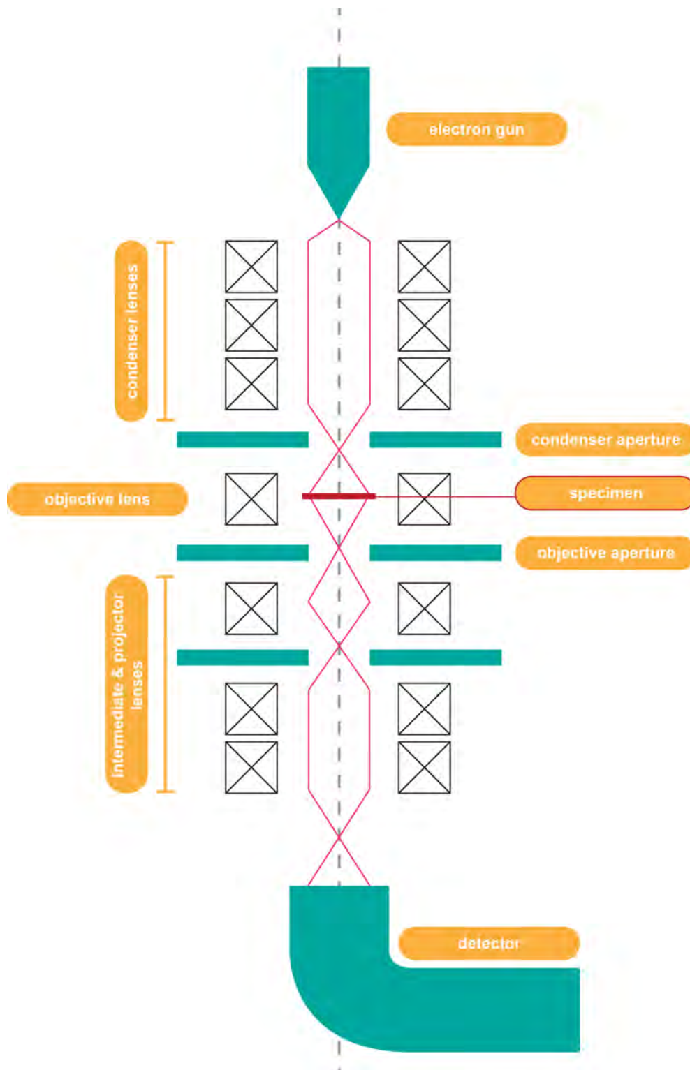
Figure 1.13 – Layout of a transmission electron microscope
