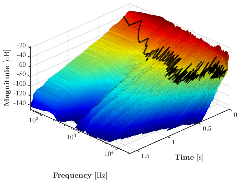
(b) EDR of the omnidirectional component of the same SRIR after the denoising process.
