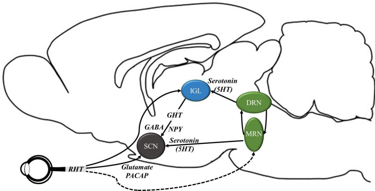
Fig. 5. Schematic representation of direct and indirect pathways from the retina to the SCN, and interconnections among the nuclei involved (IGL, MRN, DRN). The direct pathway, the RHT, results in glutamate and PACAP release into the SCN. The indirect pathway, the GHT, involves the IGL, which release GABA and NPY into the SCN. These two pathways have been described both in the nocturnal rat and in the diurnal Arvicanthis . An additional indirect pathway involves the MRN, which release serotonin in the SCN. This pathway has been described in rats, but not in Arvicanthis .
