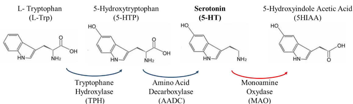
Fig. 9. Serotonin synthesis (blue arrows) and catabolism (red arrow).
