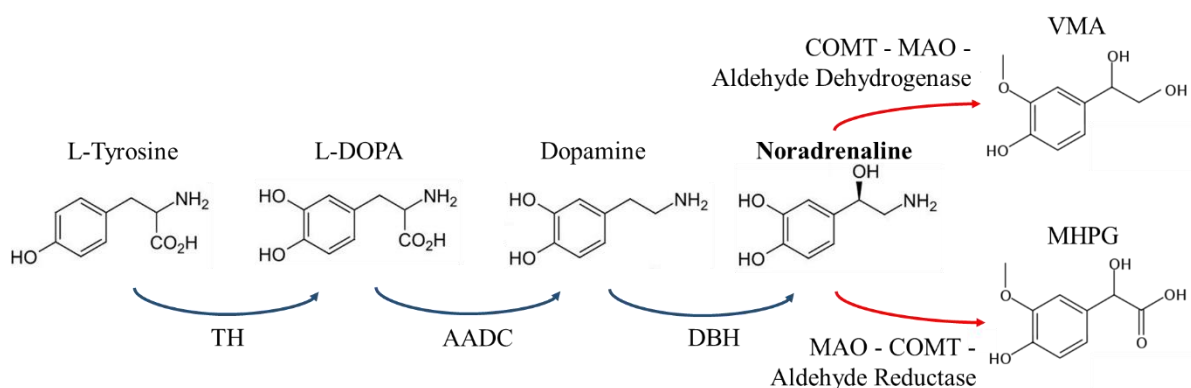
Fig. 10. Noradrenaline synthesis (blue arrows) and catabolism (red arrow).
