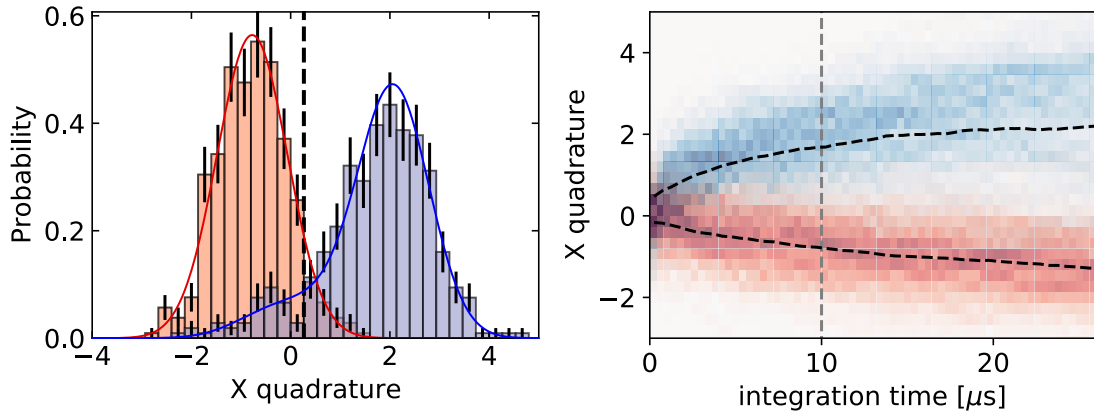
Figure 7.23: X quadratures histograms. Left- The best configuration for the detection with the no-Rydberg distribution (orange) and the one with a Rydberg atom (blue). They are both fitted by the model (solid lines), see text. Right- Evolution of the two distributions with the integration time, blue with a Rydberg and red without. Black dashed lines represent the mean value for both cases and the gray vertical dashed line gives the best integration time.
