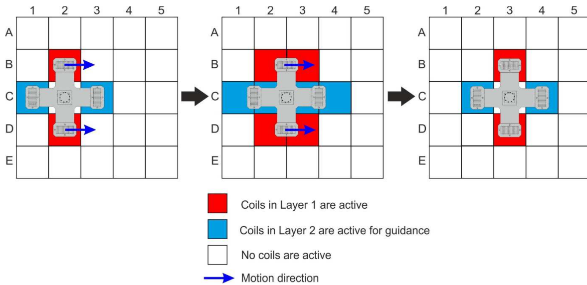
Figure C.2 Switching ‘on’ and ‘off’ of the matrix cells
