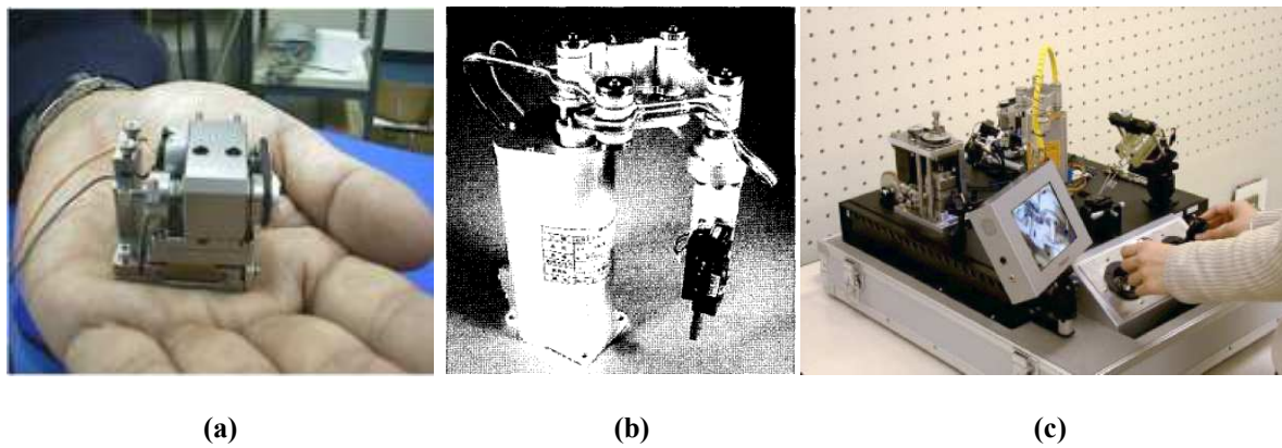
Figure 1.1 Downsize machine tools (a) Microlathe [LU 1998] (b) Micro transfer arm [MAEK 2001] (c) Portable microfactory [OKAZ 2004]
