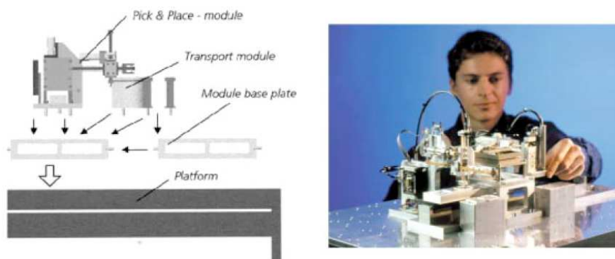
Figure 1.2 Mini factory system [GAUG 2002]
