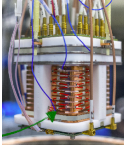
Figure 3.4.1: The Time Projection Chamber of ReD. The TPC is surrounded by a field cage of nine copper rings and is contained by a PTFE structure. It is also possible to see the two FEBS, with each cable connected to its channel.
