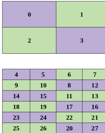
Figure 3.4.3: Mapping for the laser runs which entered the present analysis (top view of the TPC). On the top, the four bottom channel, each composed by the input of six SiPMs. On the bottom, the top tile, with its 24 read-out channels. Two CAEN ADC boards, each with 16 channels, amplify and digitize all the 28 channels.
