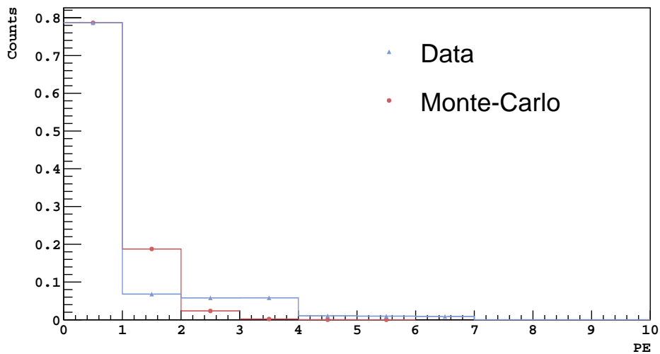
Figure 5.4.2: For Channel 19, the SER amplitude distribution from real data (blue) are compared to the output from the simulation (red), assuming a null Crosstalk Probability, P_{CT} = 0.0 . Afterpulses in itself increase the number of reconstructed photoelectrons in the laser pulse only of one afterpulse, so that in the simulation the number of events above 2 photoelectrons is negligible. Events in the data at higher PE are due to the contribution of crosstalks.
