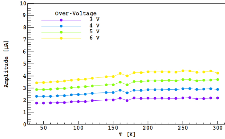
Figure 5.1.6: The amplitude of the average signal from a SPAD increases with the overvoltage. For any overvoltage a slight increase with the temperature is observed [285].
