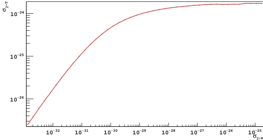
Figure 4.2.1: Scaling between the per nuclear and the elastic per nucleon cross-section for a elementary dark matter particle interacting with liquid argon through a repulsive top-hat potential.
