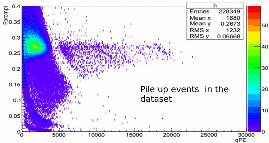
Figure 4.6.2: Pile-up events from Physics Run 022677. The performed cut are F_{prompt} < 0.4 and SubeventN > 1 . As expected from statistics, the main pile-up source is ^{39}\text{Ar} due to high activity.
