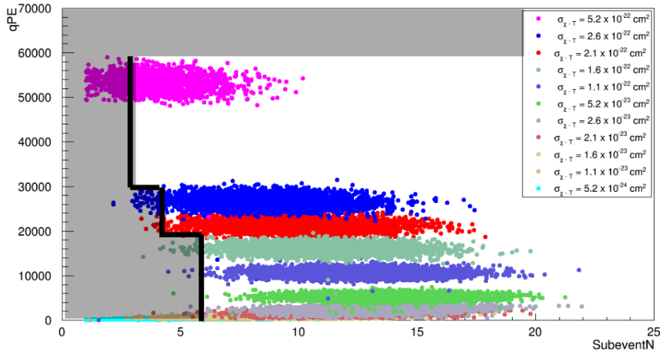
Figure 4.8.5: Cut in the qPE vs. SubeventN plane, tuned on the expected pile-up distribution in three years of lifetime.
