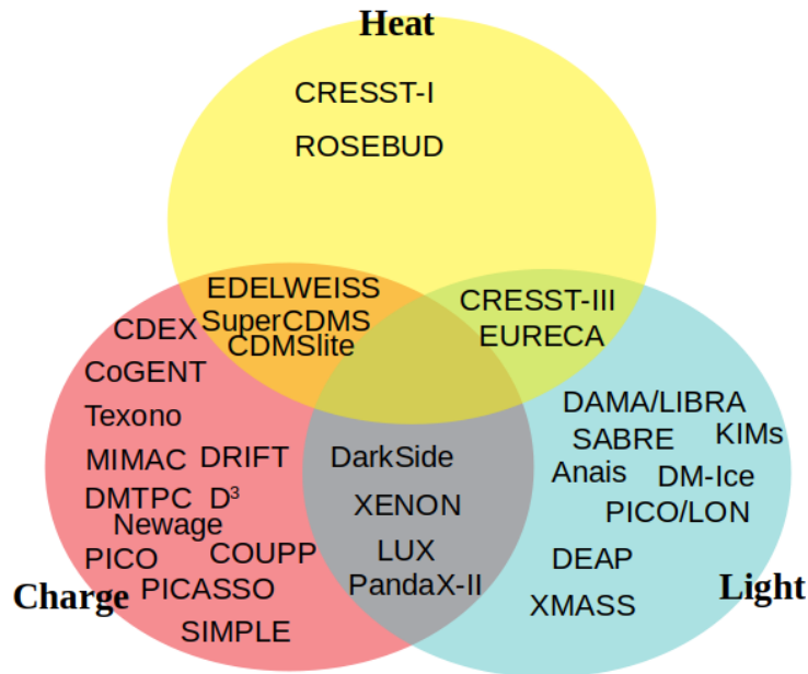
Figure 2.3.5: Representation of the main detectors for each detection strategy: the ionization charge, the scintillation light, the heat (phonons).
