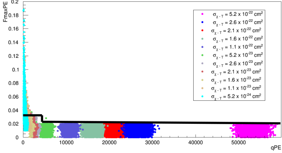
Figure 4.8.3: Selection cut on FmaxPE. As well as Fprompt the cut is stronger above the ^{39}\text{Ar} endpoint, where is F_{\text{maxPE}} < 0.02 , while above it the condition is relaxed to F_{\text{maxPE}} < 0.03 .
