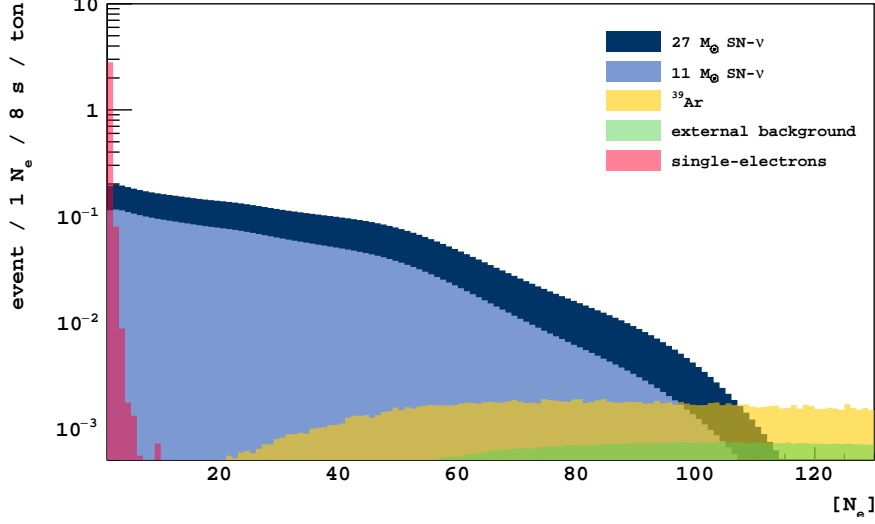
Figure 6.3.4: Energy spectrum in the N_e -variable of CCSN neutrinos, for both the 11 M_\odot and 27 M_\odot set at 10 kpc of distance, compared with the expected backgrounds, namely "single electron" events (purple), ^{39}\text{Ar} decays (yellow) and the external background (green). The selection cut is applied in the energy range (2 - 100)N_{e-} .
