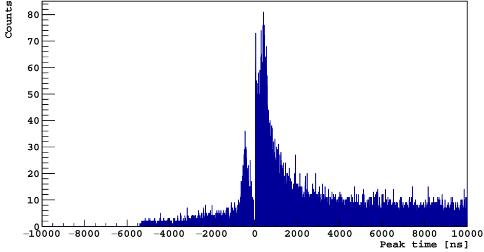
Figure 5.3.1: Peaks found before and after the primary avalanche in 5043 events from Channel 27, where the primary pulse carries 1 PE in the expected trigger time, at 5920 \pm 40 ns. For each events, the primary peak is not stored. The primary peak time is taken as zero; then all the found peaks in that event are stored according to their arrival time respect to the primary pulse. Dark (uncorrelated) noise is distributed with the same probability before and after the primary peak, while afterpulses can lay only after the primary avalanche. The drop below about 50 ns is due to the prominence of the peaks nearby the primary pulse, which results to be below the peak-finder prominence threshold.
