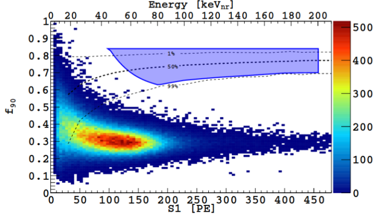
Figure 3.1.5: Distribution of the f_{90} parameter versus S1 , in 532 days of data taking in DarkSide-50 [212]. Events at f_{90} = 0.3 are electron recoils, hence scattering events from \gamma s or \beta s. The main contribution comes from ^{39}\text{Ar} \beta decays. At f_{90} = 0.7 nuclear recoils are expected, as they have a higher singlet state likelihood and then a faster scintillation signal. Nuclear recoils are neutrons and eventually WIMPs, which are specifically expected in the blue area. The three dotted lines show the f_{90} cuts at which 1 %, 50 % and 99% of the WIMPs would "survive", i.e. of WIMP acceptance, obtained thanks to calibrations with the neutron AmBe source.
