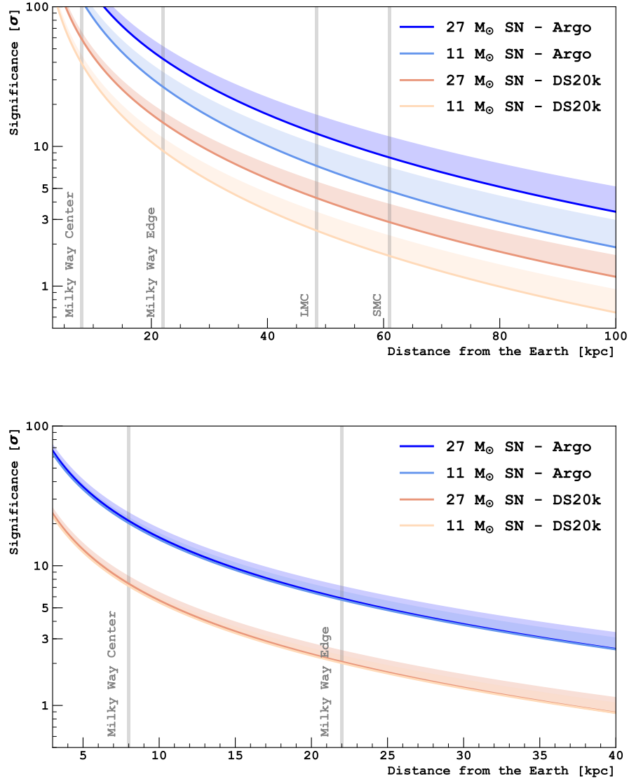
Figure 6.4.1: DarkSide-20k and Argo discovery potential to 11 M_{\odot} and 27 M_{\odot} SNe (top) and to its neutronization burst only (bottom) as a function of the distance, assuming the standard background hypothesis (solid line) and by considering a lower contamination of ^{39}\text{Ar} , up to a factor of 10 less (band). Vertical lines represent the distance from the Earth to the Milky Way center, to its farthest edge and to Large (LMC) and Small (SMC) Magellanic Clouds.
