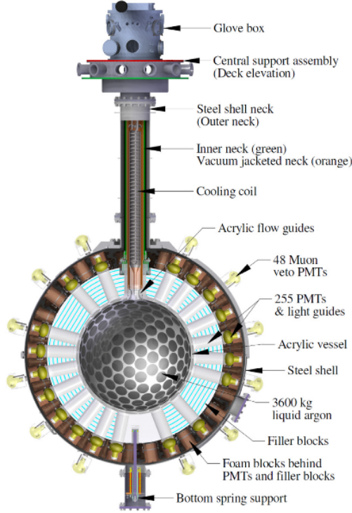
Figure 3.2.1: DEAP-3600 detector design showing the inner vessel, the LGs, the PMTs and the filler blocks, out to the stainless steel outer vessel, together with its neck. The representation does not show the TPB coating and the ultra-pure water veto, in which the outer vessel is immersed [196].
