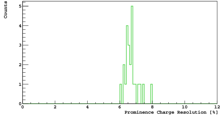
Figure 5.2.14: Resolution for the prominence charge in top tile. The charge defined from the prominence shows to have a resolution of about 6.5 %.
