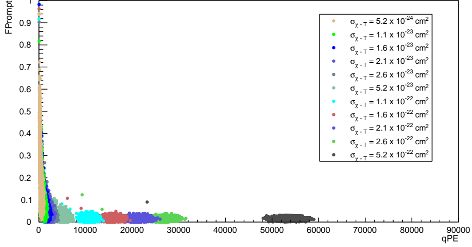
Figure 4.5.3: Comparison of MIMPs in terms of qPE and FPrompt variables. The cross-sections shown go from \sigma_{\chi-T} = 10^{-24} \text{ cm}^2 to \sigma_{\chi-T} = 10^{-22} \text{ cm}^2 , while the mass is M_\chi = 10^{18} \text{ GeV} . For each cross-section, qPE agrees with the number of expected scatterings, assuming average recoil energy of 8-12 \text{keV}_{ee} for each scattering, and hence increases with the cross-section. FPrompt, on the other hand, decreases with the increase of the cross-section, as the number of scatterings which fall out of the prompt window increases.
