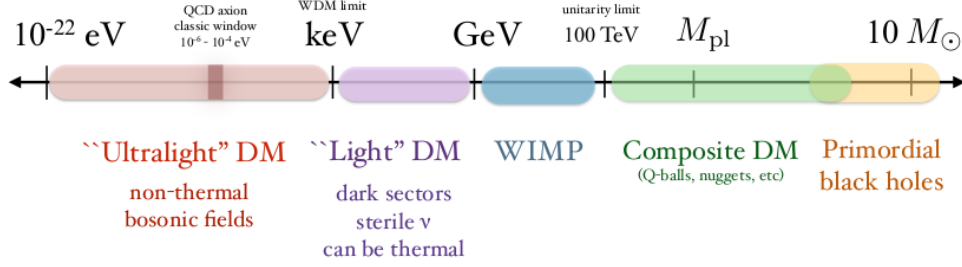
Figure 2.2.2: Dark matter main models, according to the mass of the dark matter particle [44].
