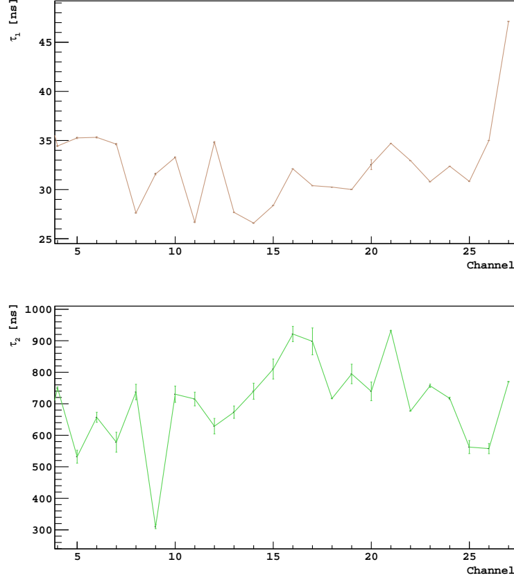
Figure 5.3.4: Characteristic times for the two exponential functions fitting the corrected afterpulse probability, for each ReD top channel.
