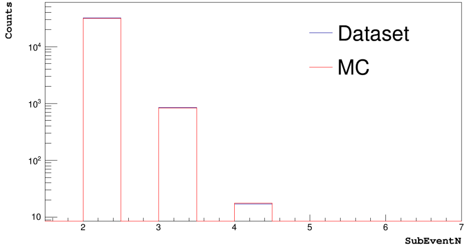
Figure 4.7.5: Distribution of EM pile-up events in Run 020412 compared to the MC simulations of the expected triggered events.
