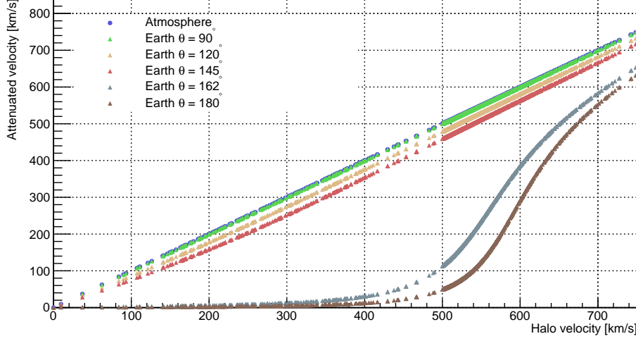
Figure 4.4.4: Attenuation of a MIMP particle coming from different directions (the zenith is set at \theta = 0 ) in DEAP-3600 with mass M_\chi = 10^{16} GeV and cross-section \sigma_{\chi-T} = 2.6 \times 10^{-18} \text{ cm}^2 after passing through the atmosphere (blue) and the mantle (green).
