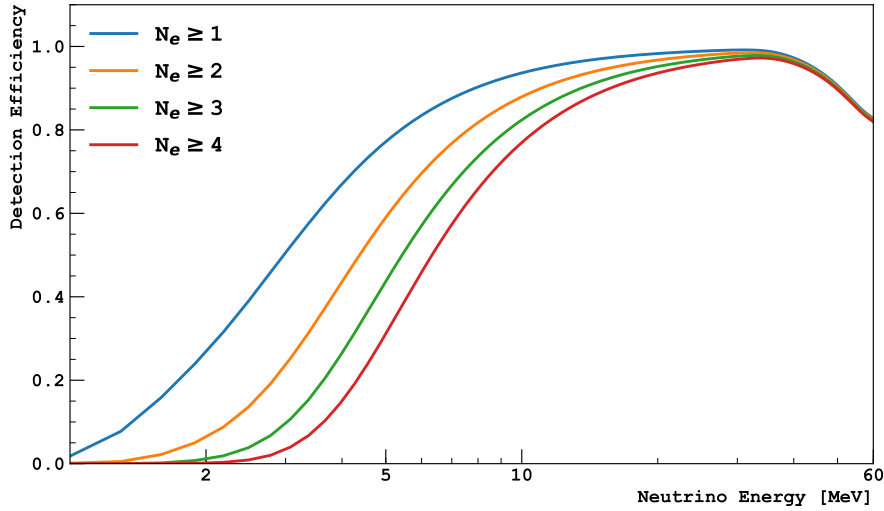
Figure 6.3.5: Detection efficiency to the CCSN signal for different energy threshold. As reference, the neutrino emission from the 27 M ⊙ CCSN at 10 kpc of distance was assumed. The threshold set is at N_e \geq 3 , in order to strongly suppress the contribution to the event rate of the single-electron background.
