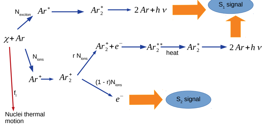
Figure 3.1.3: Scheme of the origins of the signals due to a particle scattering on liquid argon. The fraction f_L of the recoil energy goes in thermal motion. The left energy may excite or ionize argon atoms. In the first case, it will bound in a quite unstable excimer, which may be either in a triplet or a singlet state, according to the spin configuration. Whatever the case, a photon peaked at 128 nm is released. The ions also can recombine with electrons, bringing to a very excited argon dimer, which first decays vibrationally and only then radially, again either from a triplet or a singlet configuration. Both processes - exciton self-trapping and recombination- contribute to the S1 signal, both in a single and in a double phase liquid argon detector. Finally ions which do not recombine also correspond to electrons which are not captured. In a double phase chamber a drift field is applied to collect them and produce the S2 signal in the gas pocket.
