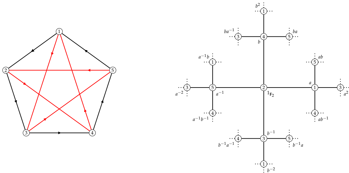
FIGURE 5.1. — On the left, black arrows represent the permutation A , red arrows B . On the right, the portion of an element c \in \mathcal{C} , for which a \star col = b * col , a^{-1} \star col = a^{-1} * col , b \star col = b^{-1} * col and b^{-1} \star col = a * col .
