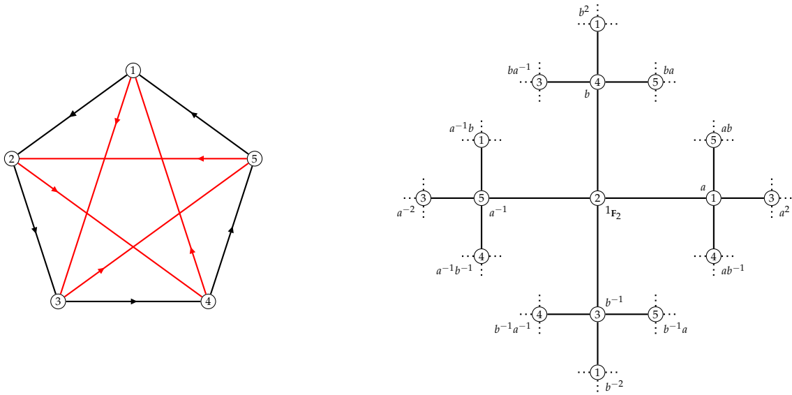
FIGURE 5.1. — On the left, black arrows represent the permutation A , red arrows B . On the right, the portion of an element c \in \mathcal{C} , for which a \star col = b \star col , a^{-1} \star col = a^{-1} * col , b \star col = b^{-1} * col and b^{-1} \star col = a * col .
