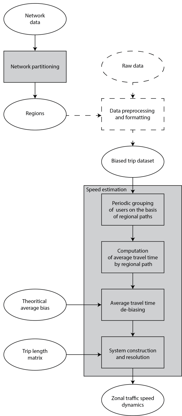
Figure 5.1: Methodological framework
