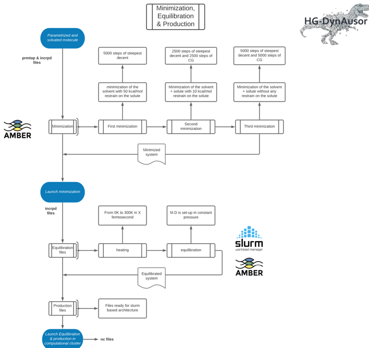
Figure 31: An overview of the last phases of module 01 of the HG-DYNAsur platform
