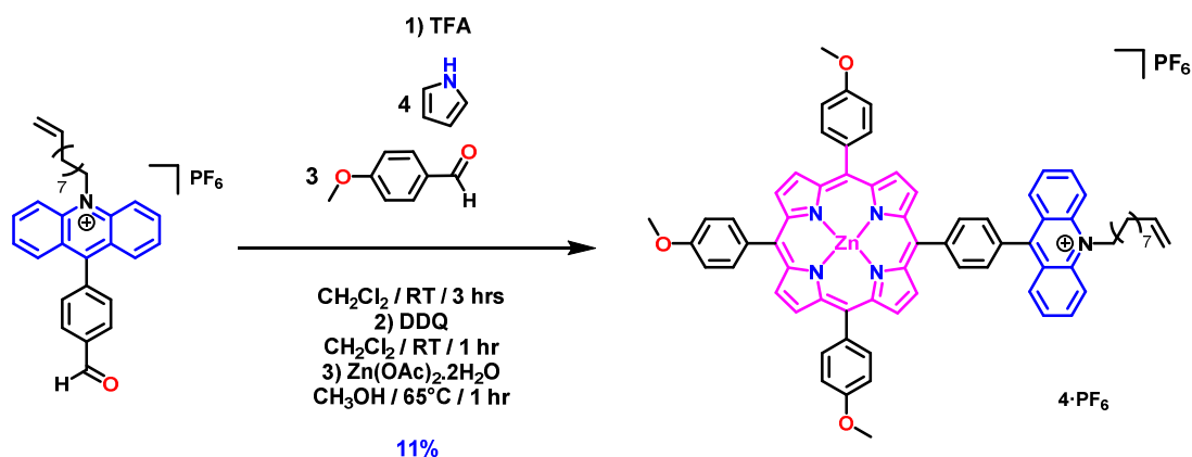
Figure 110: Chemical synthesis of the porphyrin-acridinium conjugate: 4 \cdot PF_6
