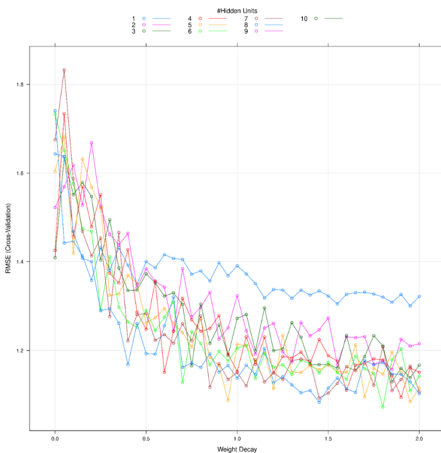
Figure 70: Performances of the NNET using a combination of hidden units and Weight decay to find the best performances for the model.
