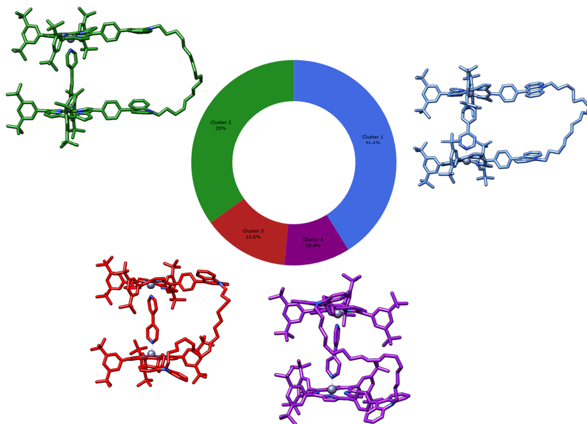
Figure 102: Knn clustering of the Bipyridine-acridinium receptor, coloured by clusters: from the most populated cluster to the less populated cluster: (In blue) the cluster 1, (In green) the cluster 2, (In red) the cluster 3 and (In purple) the cluster 4
