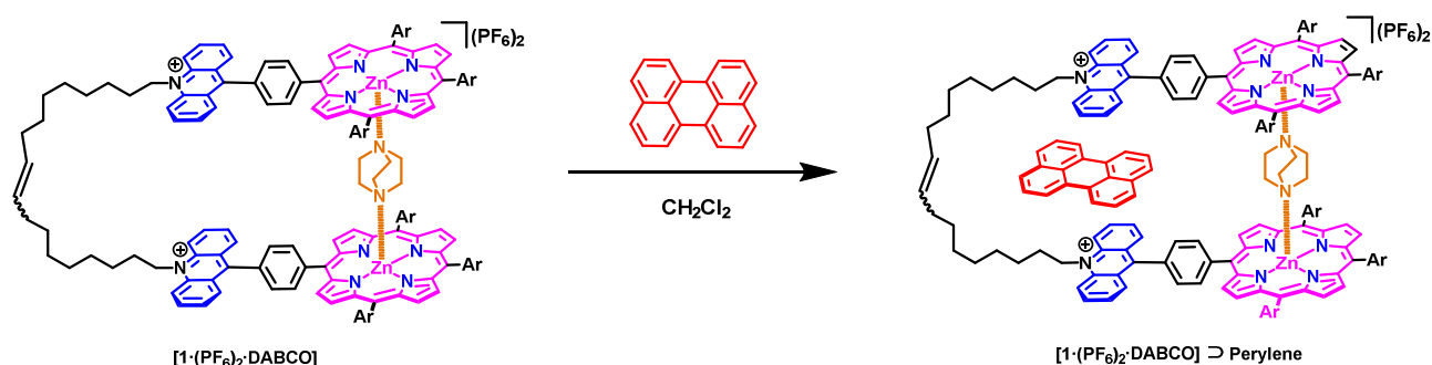
Figure 113: Chemical synthesis of the porphyrin-acridinium conjugate in complex with DABCO and Perylene: [1 \cdot (\text{PF}_6)_2 \cdot \text{DABCO}] \supset \text{Perylene}
