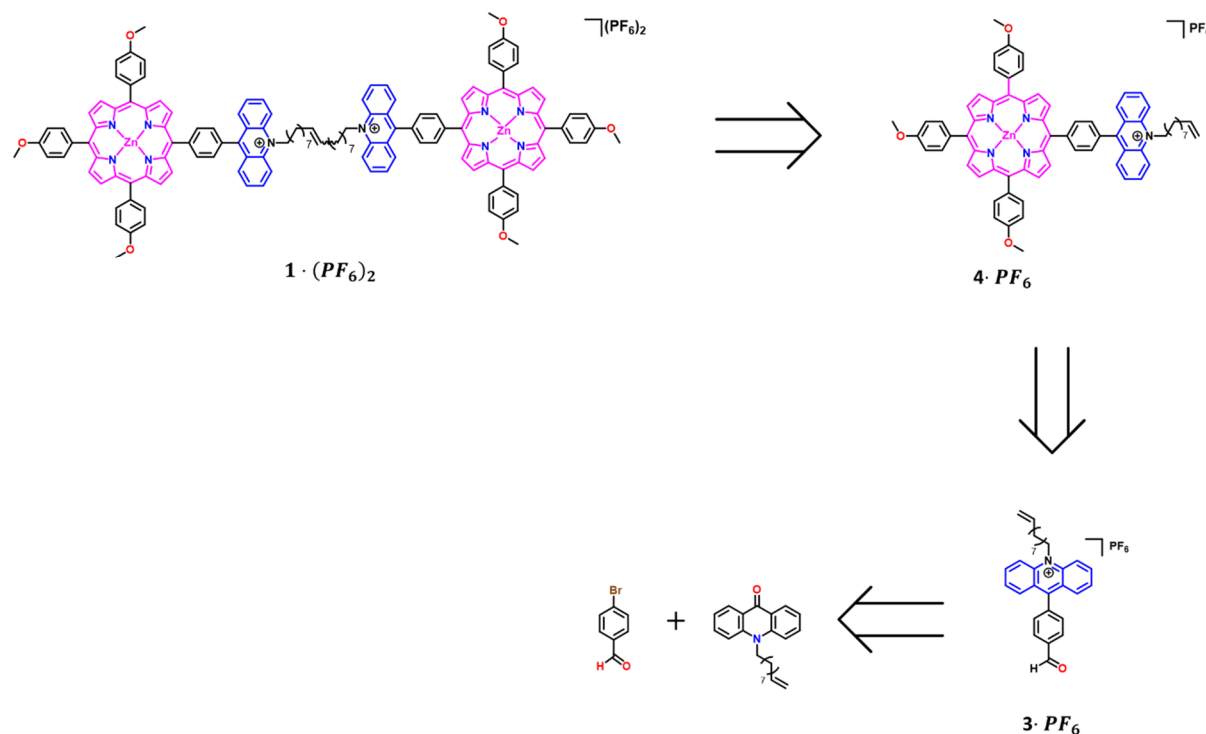
Figure 107: Retrosynthesis study of the porphyrin-acridinium conjugate: 1 · ( \text{PF}_6 ) 2
