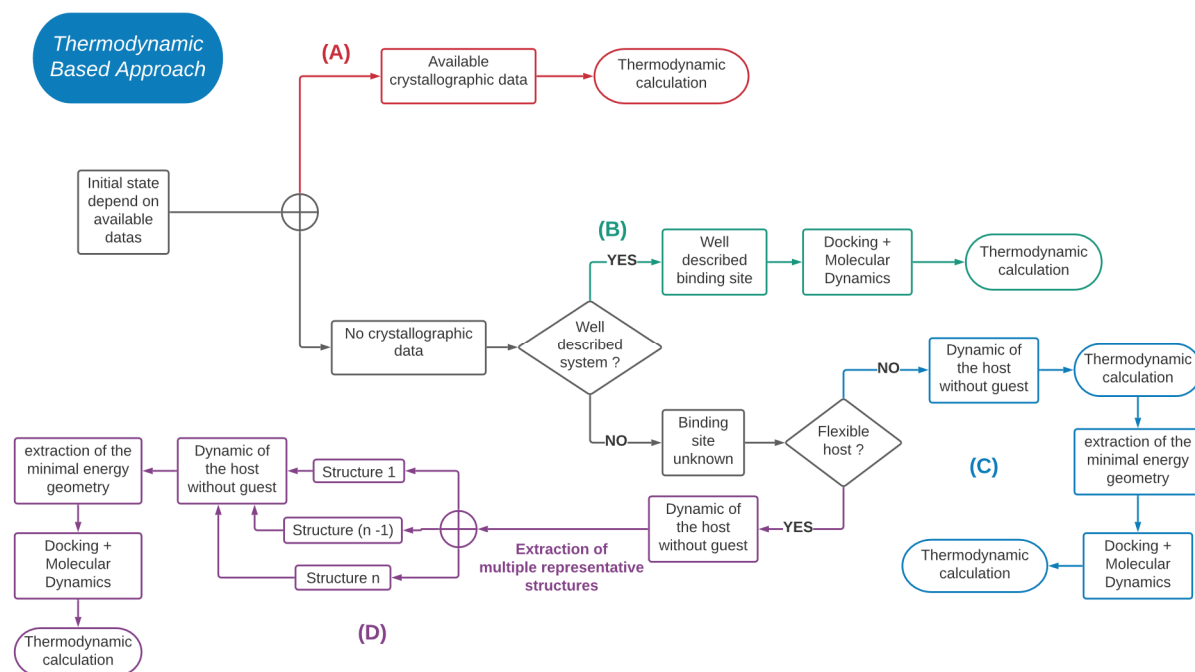
Figure 2: Flowchart of the molecular modelling approaches
