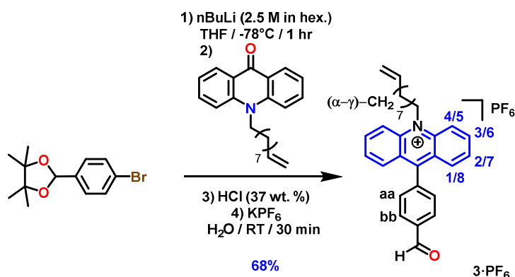
Figure 123: Chemical synthesis of the synthesis of the 10-allyl-9-(4-formylphenyl)acridin-10-ium ( 3 \cdot \text{PF}_6 )
