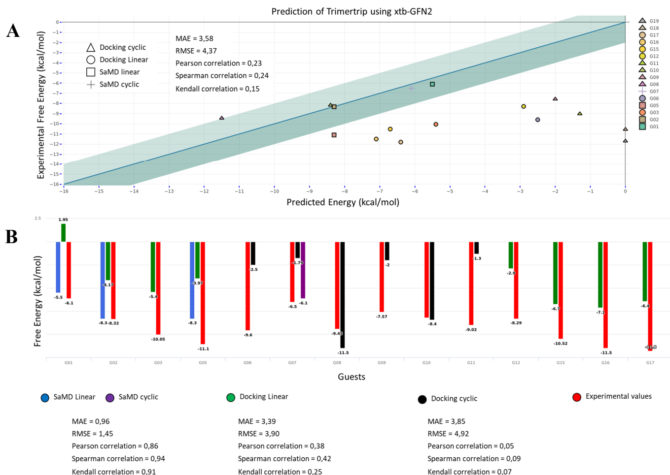
Figure 58: Comparison of experimental binding free energies with predicted values. (Top) correlation plot; the green-shaded area represents a threshold of \pm 1 kcal/mol from the experimental energy; the symbols indicate the nature of the guest and the method used for binding mode generation (triangle = docking for cyclic guest, circle = docking for linear guest, square = SaMD for linear guest, cross = SaMD for cyclic guest). (Bottom) histogram of binding free energy coloured by the method used for binding mode generation (black = docking for cyclic guest, green = docking for linear guest, blue = SaMD for Linear guest, purple = SaMD for cyclic guest). G18 and G19 guests are not shown or considered for statistical analysis because it was not possible to generate a plausible binding mode for them.
