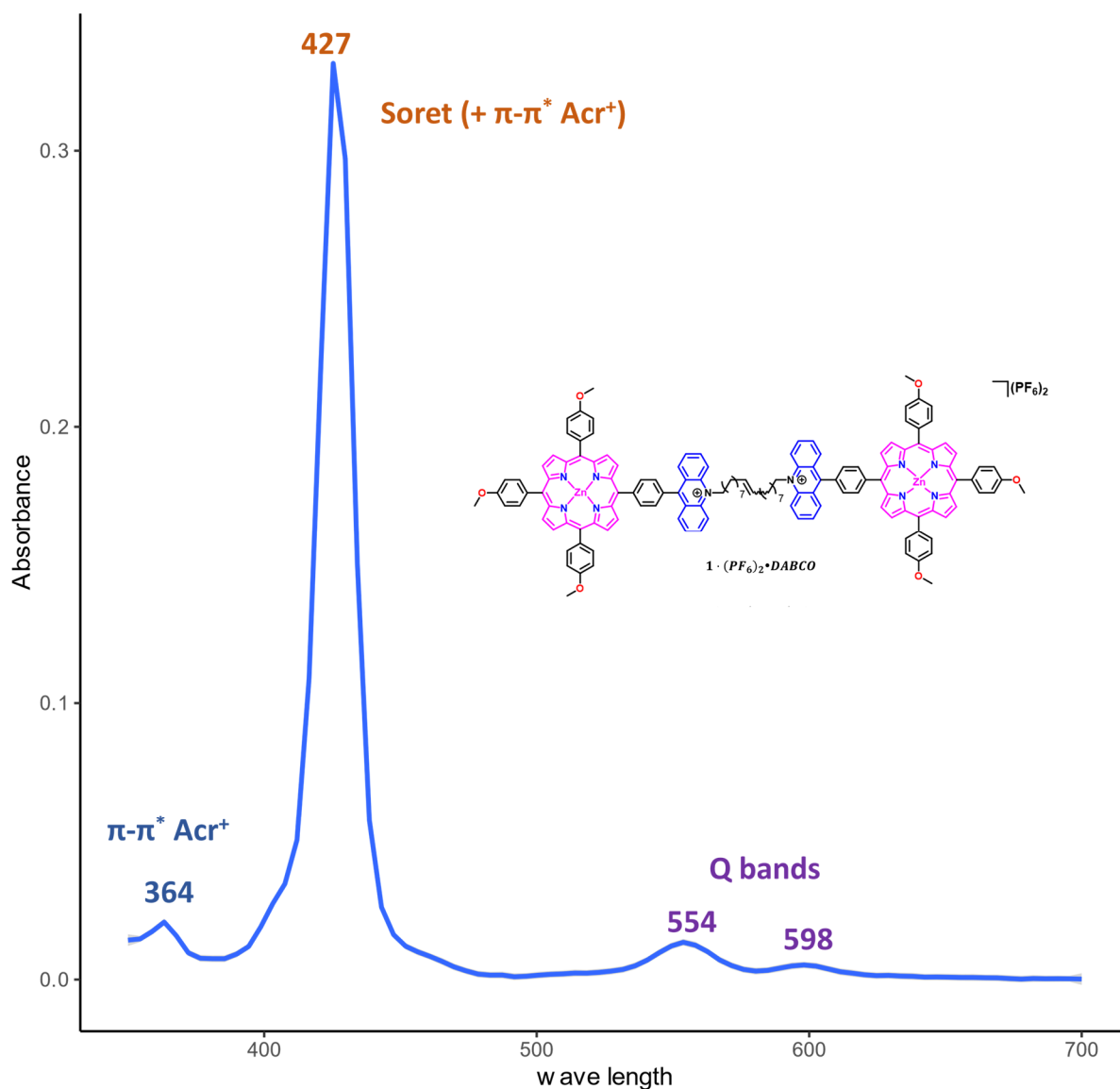
Figure 115: UV/Visible spectrum ( \text{CH}_2\text{Cl}_2 , 298 K, l = 1\text{ cm} , c = 4.37 \cdot 10^{-6}\text{ M} ) of the tweezer ( \mathbf{1} \cdot (\text{PF}_6)_2 )
