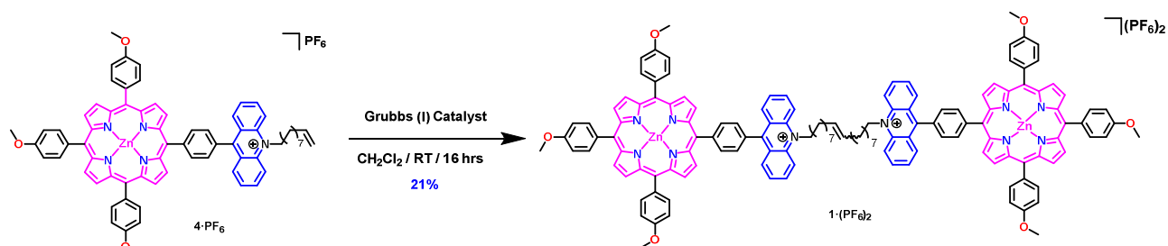
Figure 111: Synthesis of the porphyrin-acridinium conjugate: 1 \cdot (PF_6)_2
