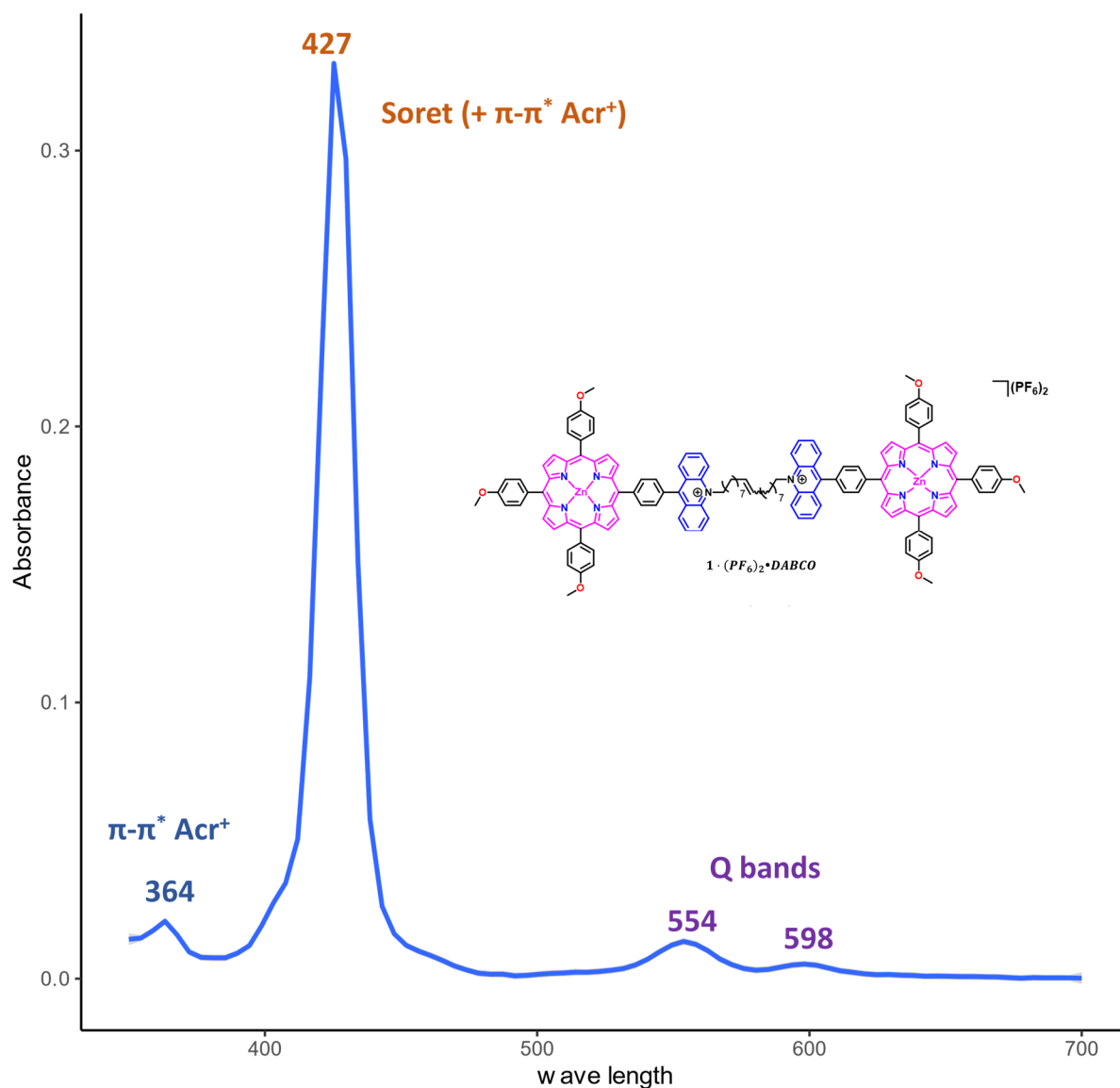
Figure 115: UV/Visible spectrum ( \text{CH}_2\text{Cl}_2 , 298 K, l = 1\text{ cm} , c = 4.37 \cdot 10^{-6}\text{ M} ) of the tweezer ( 1 \cdot (\text{PF}_6)_2 )
