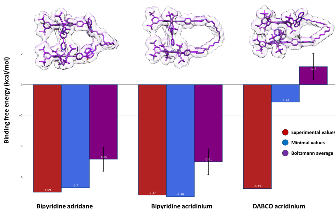
Figure 105: Binding free energy prediction of Zn(II)-porphyrin receptor considering three different receptors: (Left) the Zn(II)-porphyrin-acridane with bipyridine as a ligand ; (Middle) The Zn(II)-porphyrin-acridinium with bipyridine as a ligand ; (Right) The Zn(II)-porphyrin-acridinium with DABCO as a ligand
