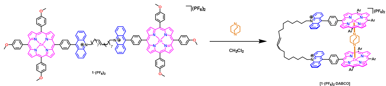
Figure 112: Chemical synthesis of the porphyrin-acridinium conjugate in complex with DABCO: [1 \cdot (\text{PF}_6)_2 \cdot \text{DABCO}]
