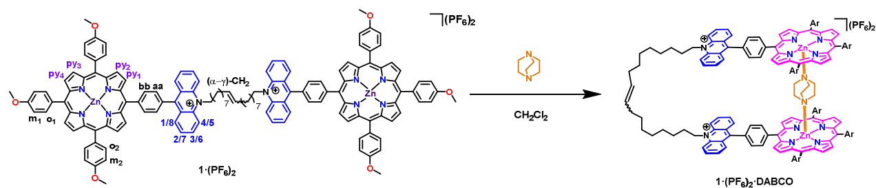
Figure 126: Synthesis of 1 \cdot (PF_6)_2 \cdot DABCO
