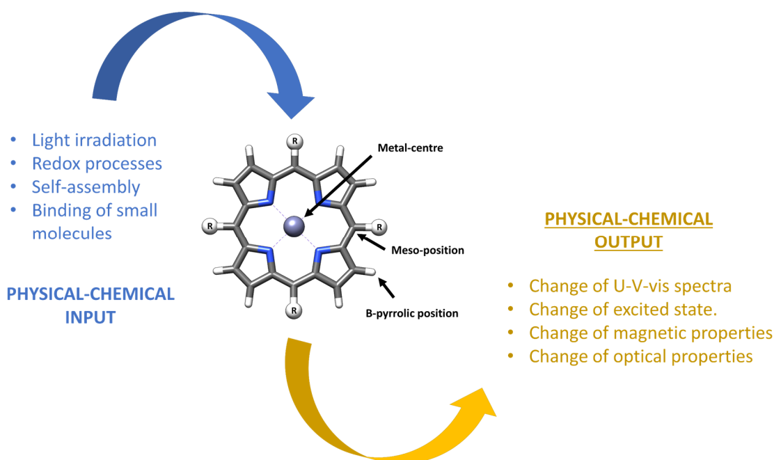
Figure 91: Overview of the application of porphyrinoids, whose physical-chemical output depend on the applied stimuli. The porphyrin core is also defined and described by the metal-centre and the main functionalisation sites ( meso and \beta -positions) 151
