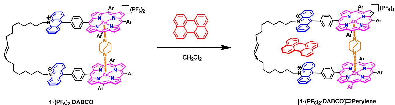
Figure 127: Synthesis of [1 \cdot (PF_6)_2 \bullet DABCO] \supset Perylene
