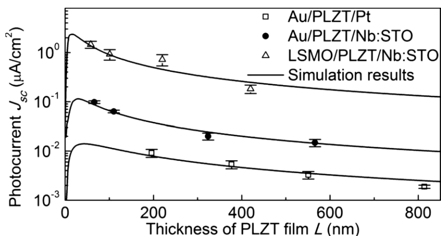
Figure 1.14 Short-circuit photovoltaic current vs thickness of PLZT thin film, as determined from calculations with different electrodes [60].
