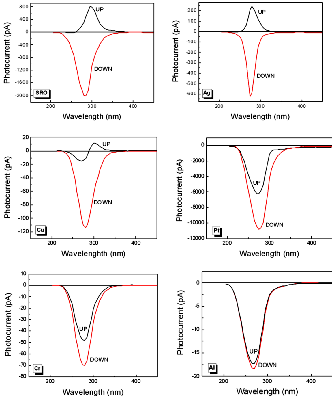
Figure 1.12. Photocurrent measured in PZT capacitors for different upper electrodes [61].
