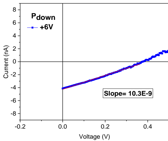
Figure 3.10 (a) Conductance plotted as a function of fluence of UV light for up and down polarization state. b) Linear fit of I-V curve at small voltages for +6V pre-polarized state under 365nm wavelength at 35.5 mW/cm 2 .
