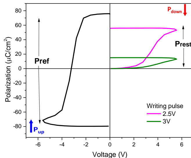
Figure 4.5. Half loop for negative voltage showing the amount of switchable polarization ( P_{pref} ) from P_{down} to P_{up} state after removing the leakage contribution obtained during the writing pulse. After polarization writing and photocurrent measurements, the amount of polarization without leakage ( P_{prest} ) which can still be switched down is measured by the positive voltage during the reading pulses. P_{prest} is shown for writing pulse of 2.5V and 3V.
