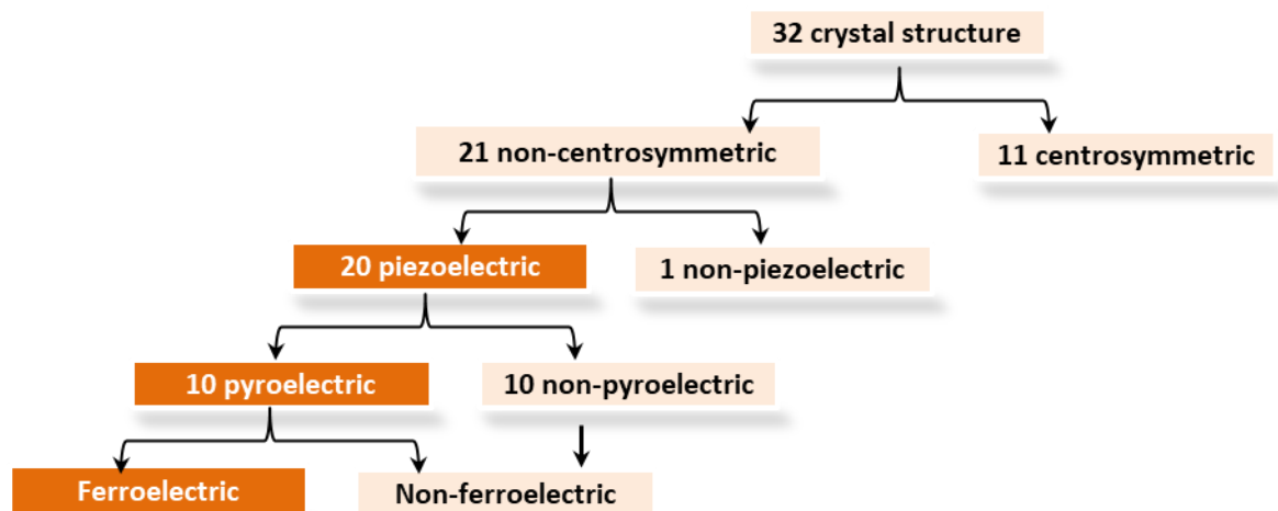
Figure 1.1. Flow chart of 32 crystal classes.
