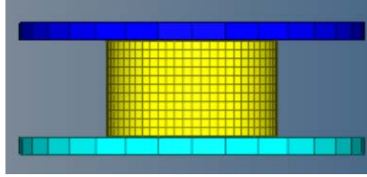
Figure 2.4: Finite element modeling of the SEBS gel under compressive plate tests.
