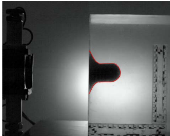
(b) Photograph of the gel wall displacement of SEBS gel during blunt impacts.
