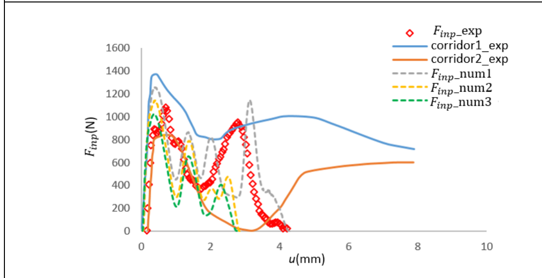
(b) Force-displacement relationship with different curvature radii (num1, 2 and 3 correspond to curvature radius r=56.80 mm, 63.31 mm and 70 mm respectively).
