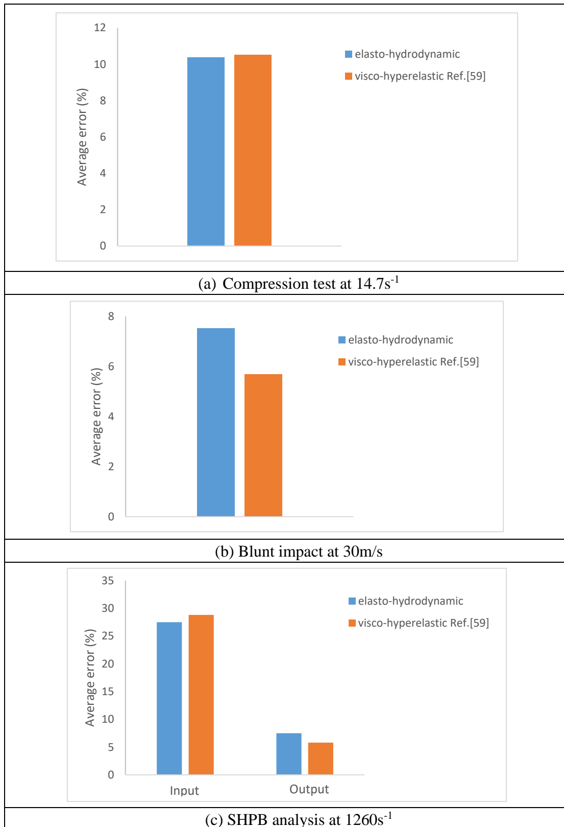
Figure 2.14: Comparison of average error of experimental and numerical results between this chapter (elasto-hydrodynamic with strain rate effect) and Ref. [59].
