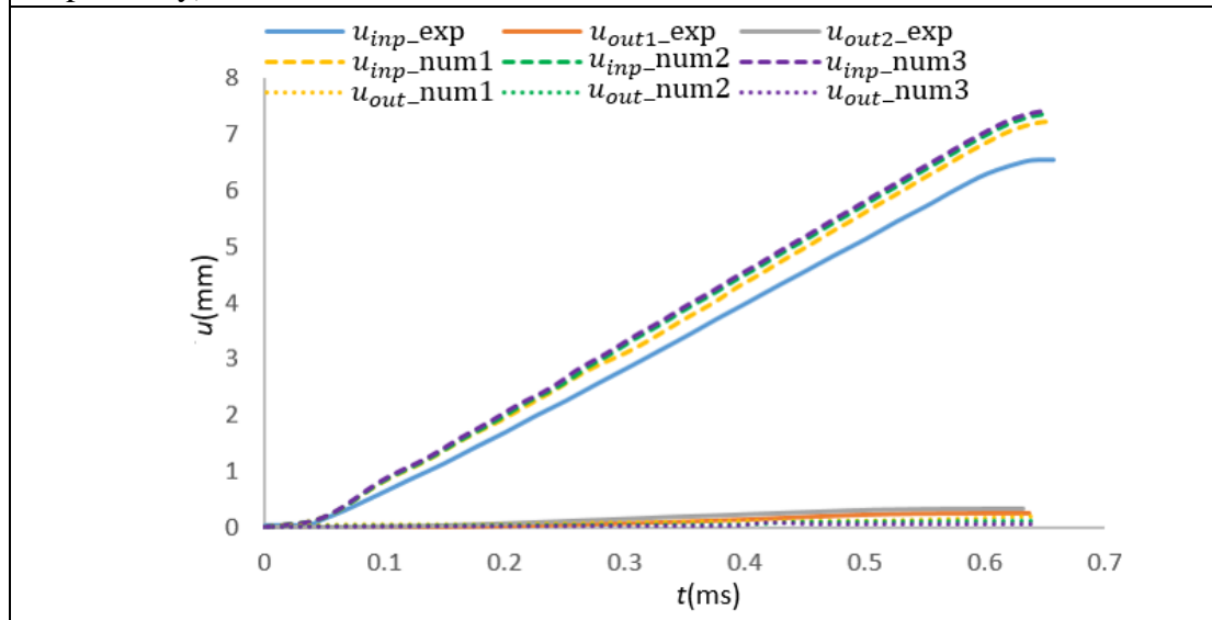
(b) Interface displacements ( u_{inp}, u_{out} ) with different curvature radii (num1, 2 and 3 correspond to curvature radius r=56.80\text{mm} , 63.31\text{mm} and 70\text{mm} respectively).
