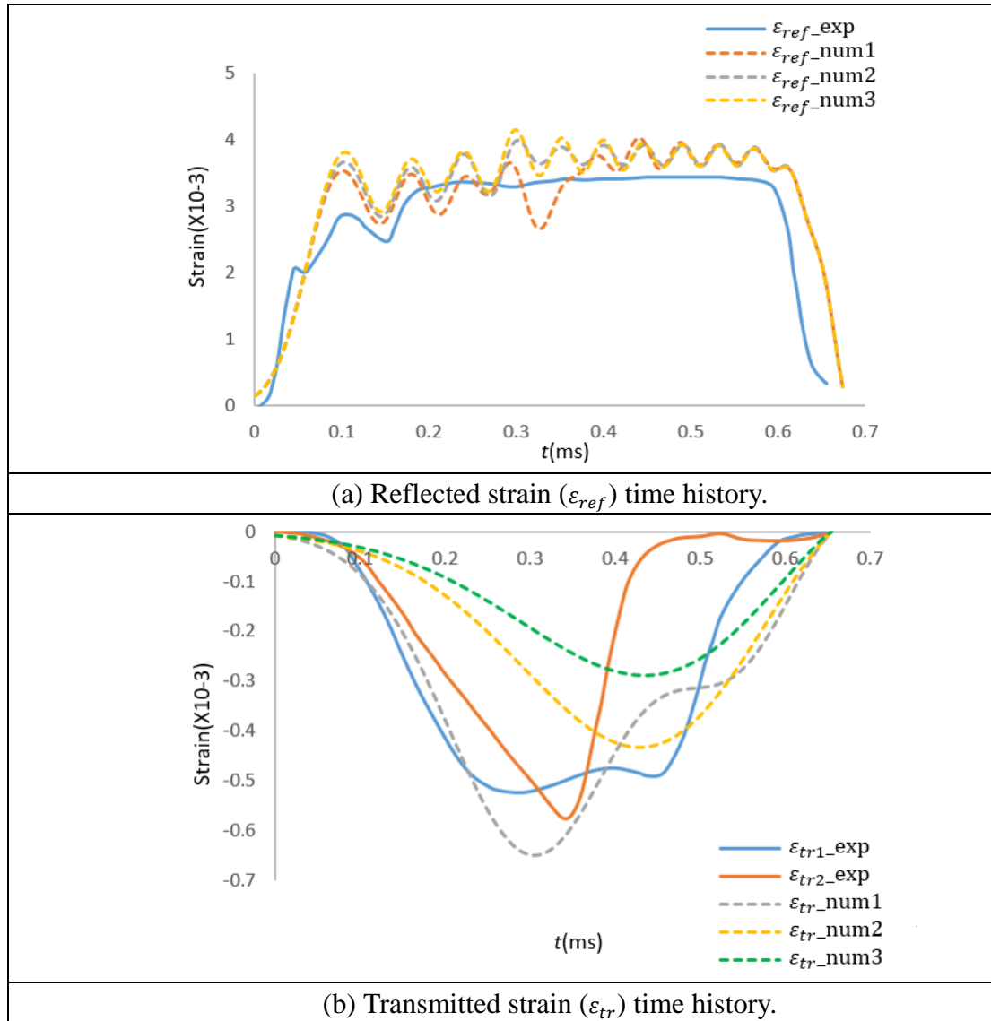
Figure 3.9: Effect of curvature radii on reflected and transmitted strain signals using porcine rib material properties, where num1, 2 and 3 correspond to curvature radius r=56.80\text{mm} , 63.31\text{mm} and 70\text{mm} respectively.
