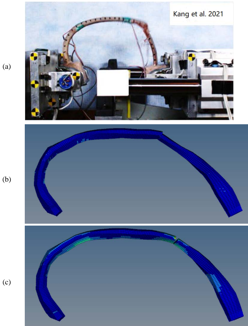
Figure 4.7: Illustration of experimental (a) and numerical fracture locations with human rib (b) and porcine rib (c) material properties.
