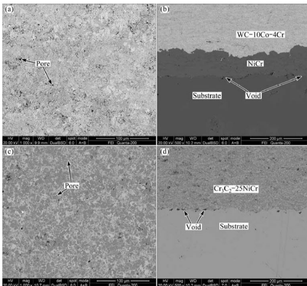
Fig. 1.7 SEM photographs of WC–10Co–4Cr and Cr 3 C 2 –25NiCr coated on H13 steel: (a) WC–10Co–4Cr (plan view); (b) WC–10Co–4Cr (cross-section); (c) Cr 3 C 2 –25NiCr (planar view); (d) Cr 3 C 2 –25NiCr (cross-section) [41]
