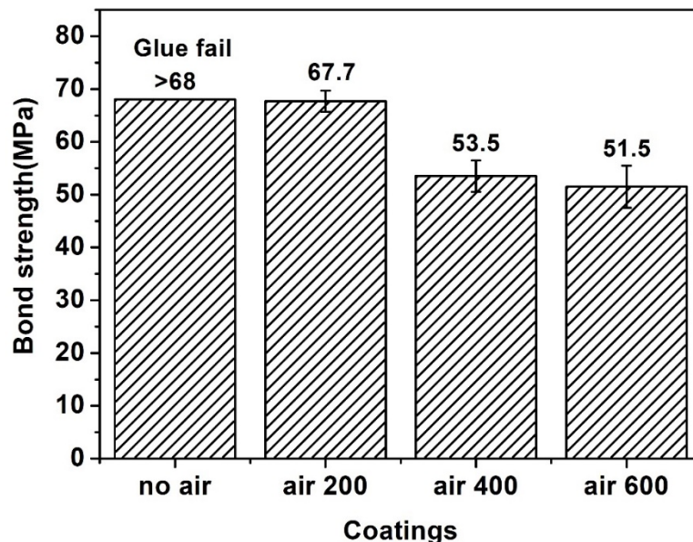
Fig. 5.12 The bonding strength of the four as-sprayed NiCoCrAlYTa coatings
