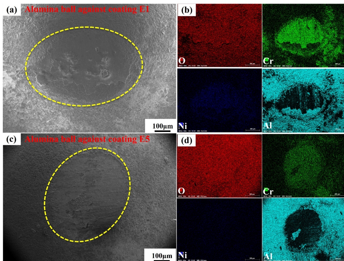
Fig. 4.24. SEM micrographs and element mappings of the wear scars produced on the alumina counter-bodies against Cr 3 C 2 -NiCr coatings. (a) and (b): vs coating E1; (c) and (d): vs coating E5.
