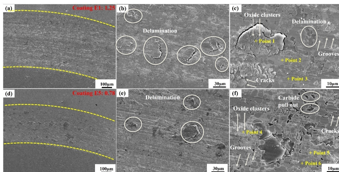
Fig. 4.22. SEM micrographs of the wear scar surfaces of Cr 3 C 2 -NiCr coatings. (a), (b) and (c): coating E1; (d), (e) and (f): coating E5.
