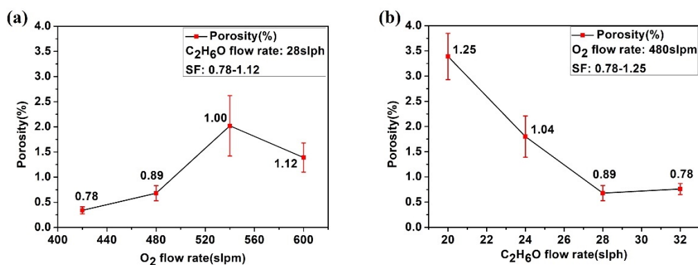
Fig. 4.11 Evolution of the porosity of Cr 3 C 2 -NiCr coatings: (a) vs. different O 2 flow rates; (b) vs. different C 2 H 6 O flow rates.
